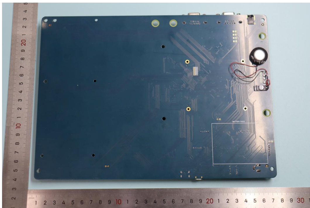
SC200E-WF + EVB _Bottom
