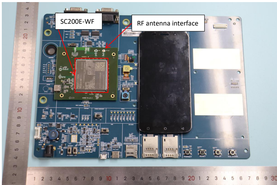
SC200E-WF + EVB _Top
