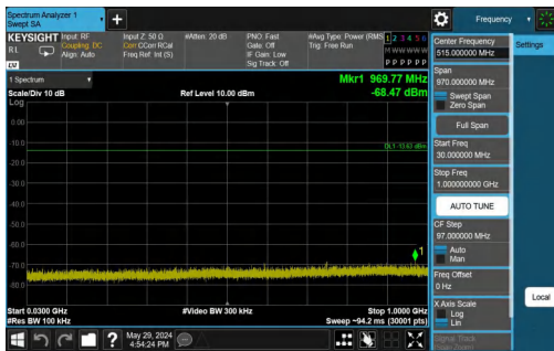
3DH5-Ant1-2402-30~1000-PASS
