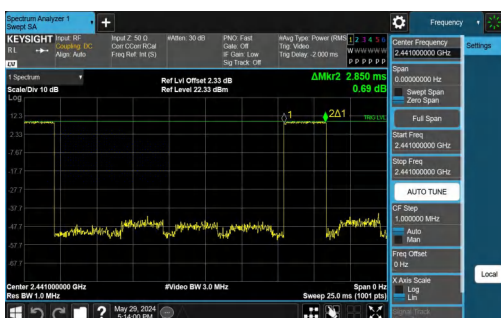
3DH1-Ant1-Hop-PASS
