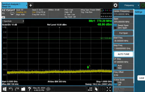
2DH5-Ant1-2441-30~1000-PASS
