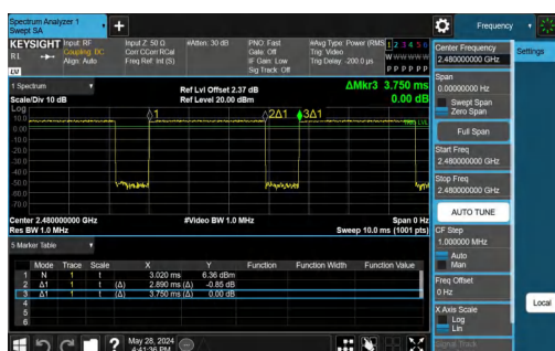
NTVN-3DH5-Ant1-2480
