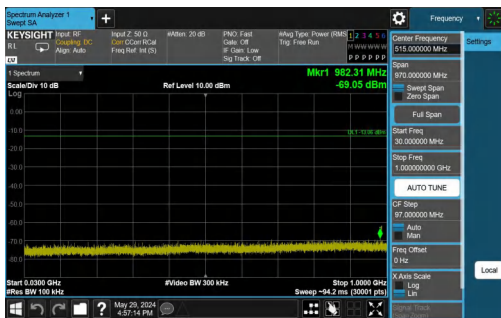
3DH5-Ant1-2441-30~1000-PASS
