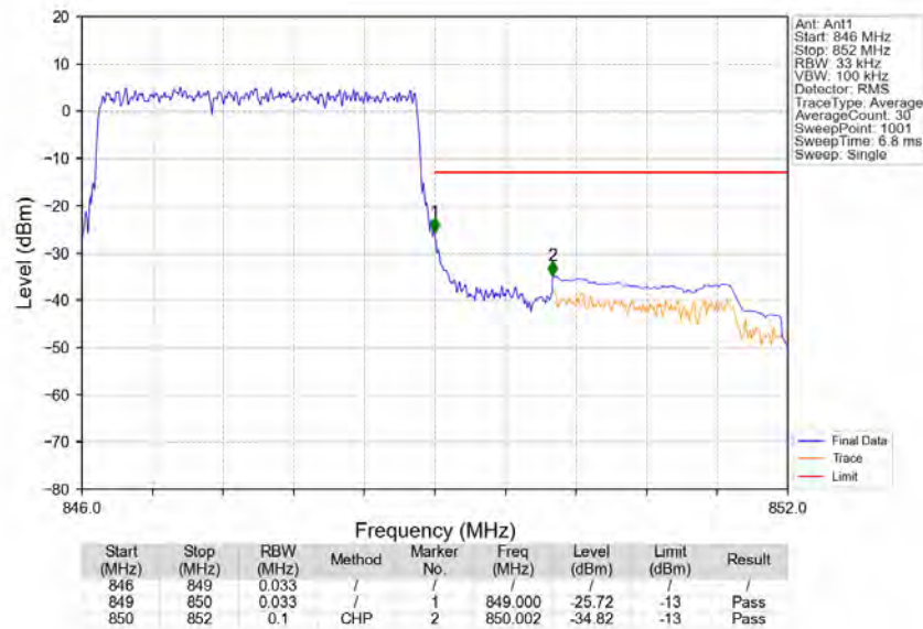
Band5_3MHz_QPSK_HCH_847.5MHz_RB_15_0_NTNV
