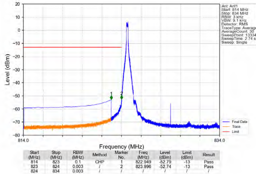
Band5_10MHz_64QAM_LCH_829MHz_RB_1_0_NTNV
