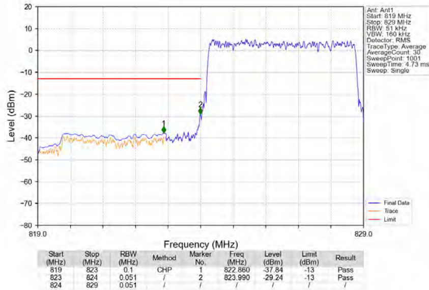
Band5_5MHz_QPSK_LCH_826.5MHz_RB_25_0_NTNV
