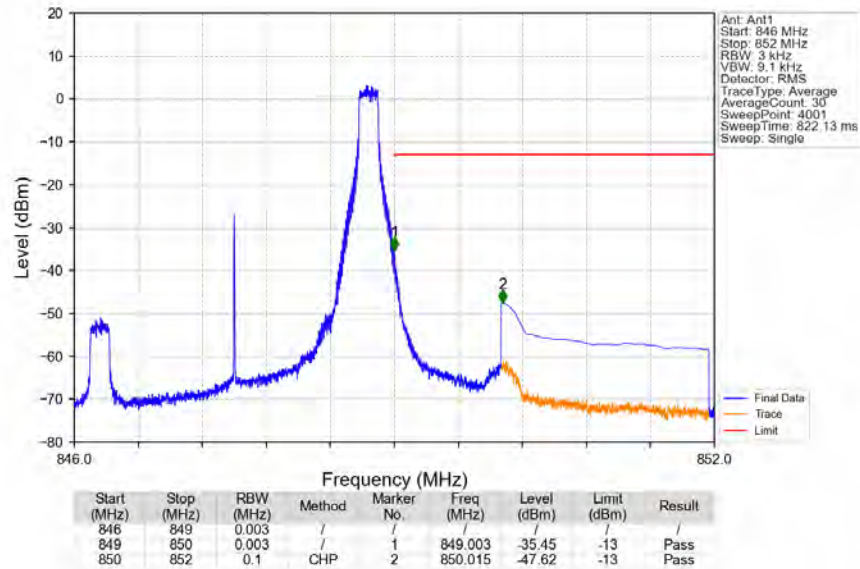
Band5_3MHz_256QAM_HCH_847.5MHz_RB_1_14_NTNV
