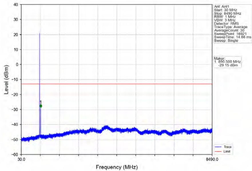
Band5_10MHz_64QAM_HCH_844MHz_RB_1_49_NTNV
