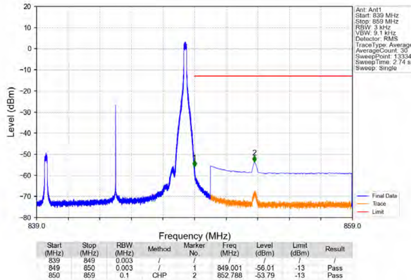
Band5_10MHz_256QAM_HCH_844MHz_RB_1_49_NTNV
