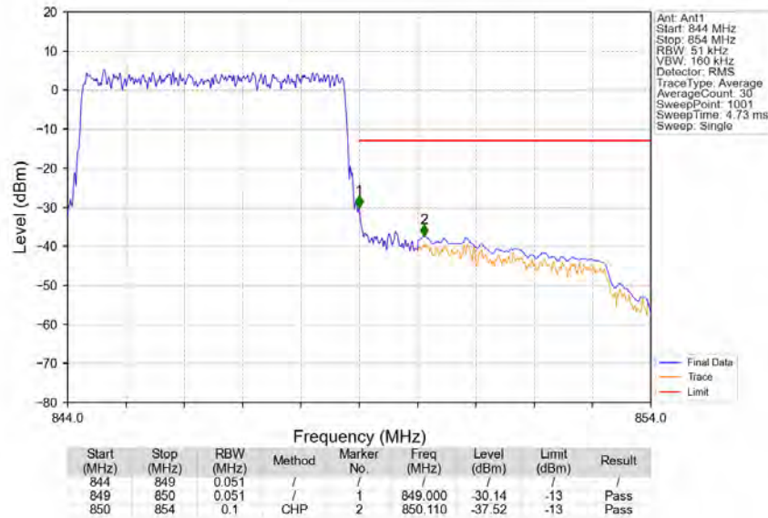
Band5_5MHz_QPSK_HCH_846.5MHz_RB_25_0_NTNV
