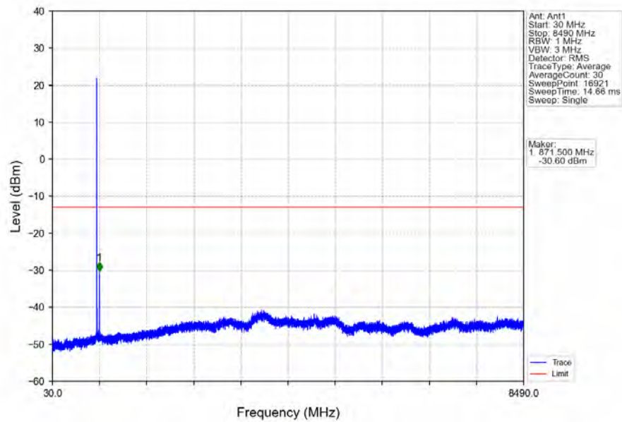
Band5_10MHz_16QAM_LCH_829MHz_RB_50_0_NTNV
