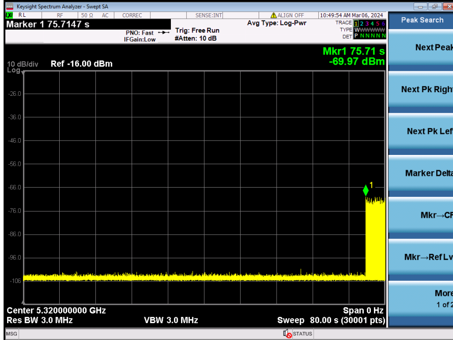
power-on cycle(5320MHz)
