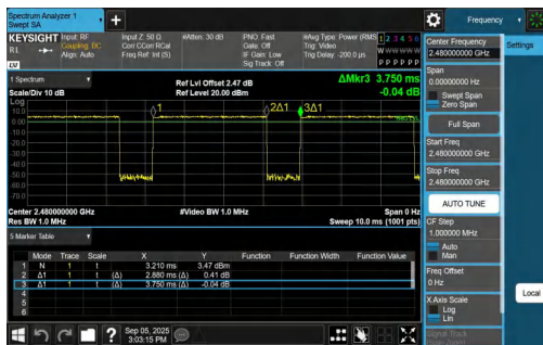
NTVN-3DH5-Ant1-2480
