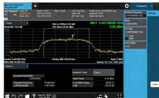
3DH5-Ant1-2441
