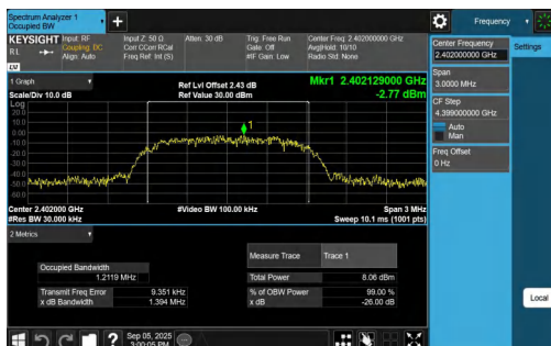
3DH5-Ant1-2402
