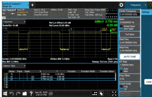
NTVN-2DH5-Ant1-2441
