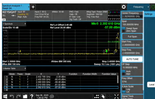
3DH5-Ant1-Hop_2402-PASS
