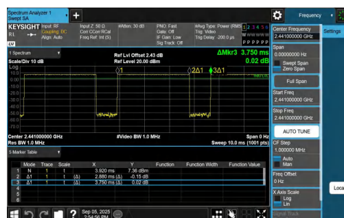
NTNV-DH5-Ant1-2441
