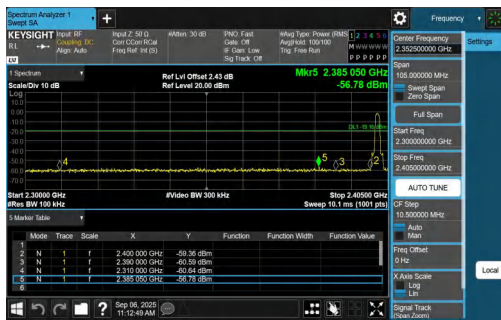
2DH5-Ant1-2402-PASS
