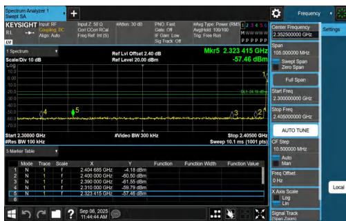
2DH5-Ant1-Hop_2402-PASS
