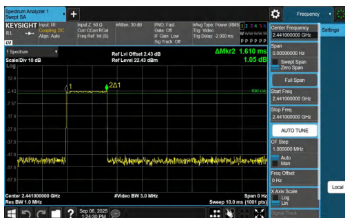
2DH3-Ant1-Hop-PASS
