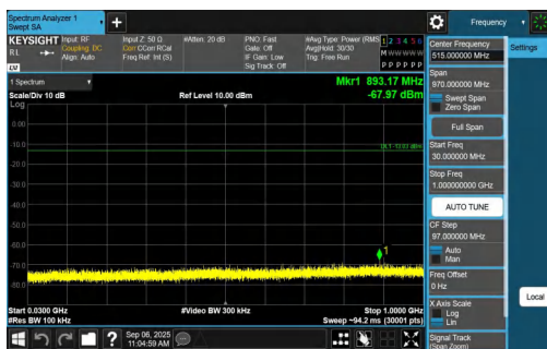
DH5-Ant1-2441-30~1000-PASS
