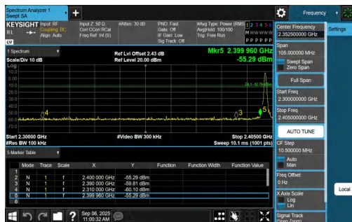
DH5-Ant1-2402-PASS
