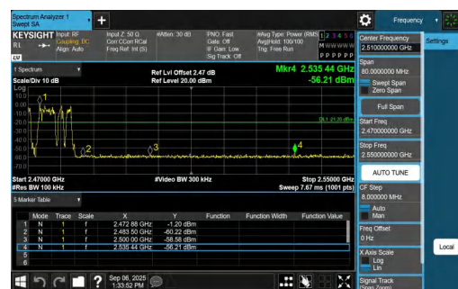
3DH5-Ant1-Hop_2480-PASS
