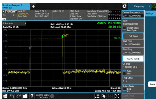
DH5-Ant1-Hop-PASS
