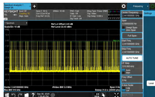
3DH5-Ant1-Hop-PASS
