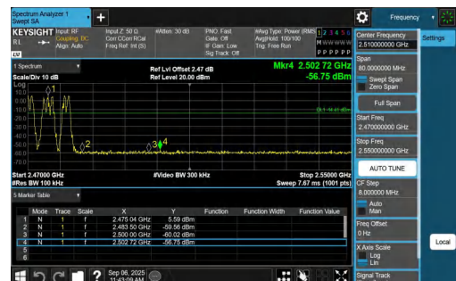
DH5-Ant1-Hop_2480-PASS
