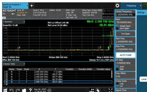
DH5-Ant1-Hop_2402-PASS
