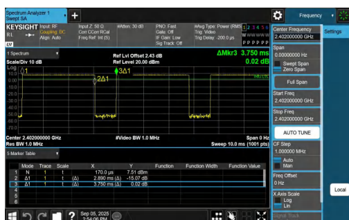
NTNV-DH5-Ant1-2402
