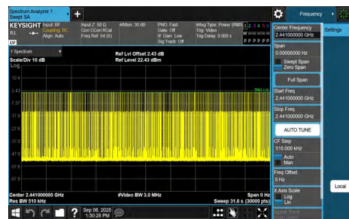
3DH1-Ant1-Hop-PASS
