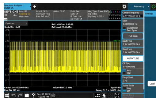
2DH1-Ant1-Hop-PASS
