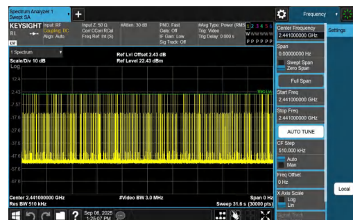
2DH3-Ant1-Hop-PASS
