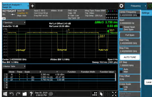
NTVN-3DH5-Ant1-2402
