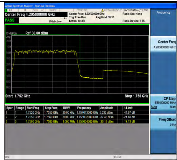
Band4-3MHz-QPSK-20385-15RB#0-PASS
