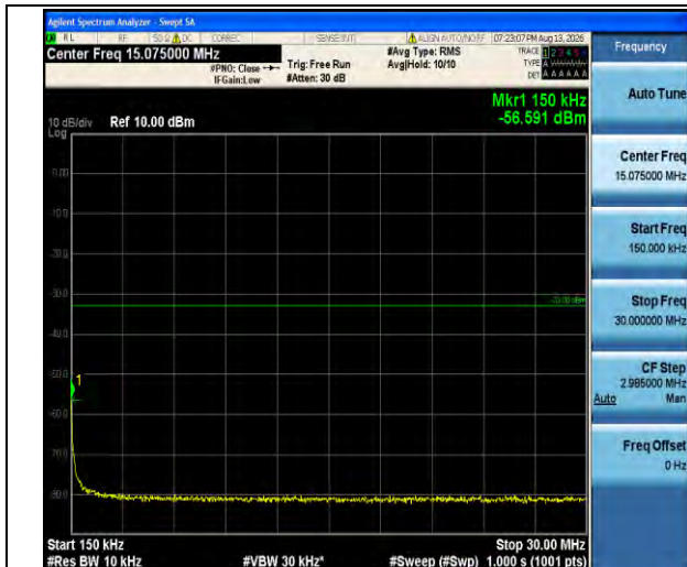
Band4-20MHz-QPSK-20175-1RB#0-0.15~30-PASS
