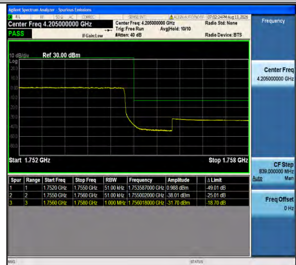
Band4-5MHz-QPSK-20375-25RB#0-PASS
