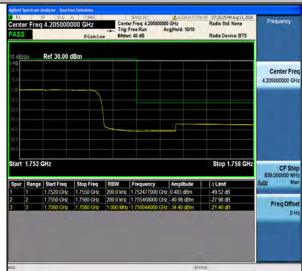
Band4-20MHz-QPSK-20300-100RB#0-PASS
