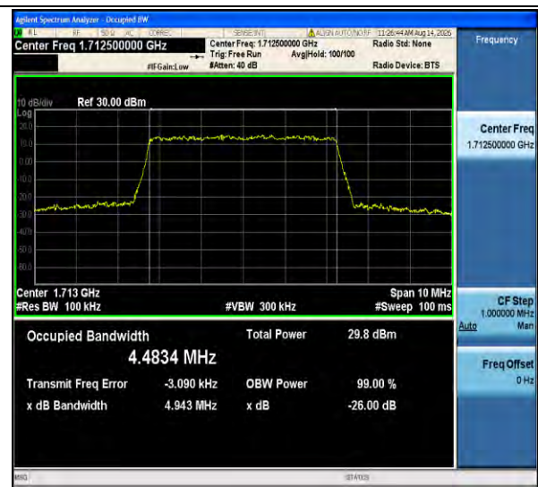
Band4-5MHz-16QAM-19975-25RB#0-PASS
