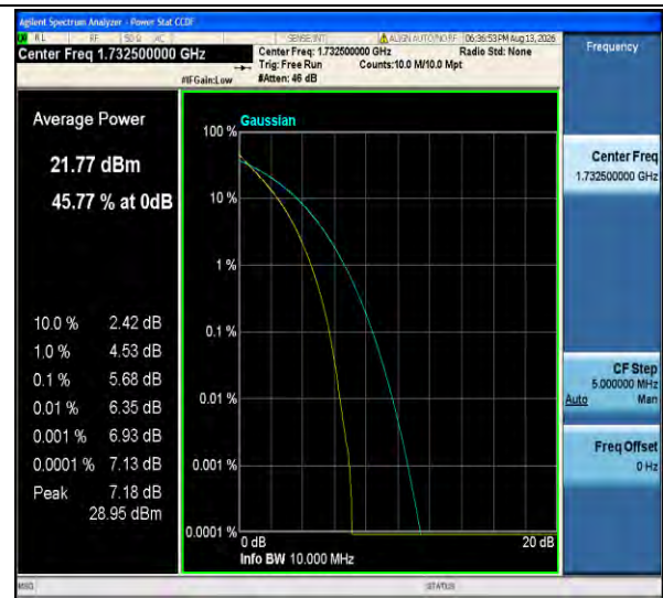
Band4-10MHz-QPSK-20175-50RB#0-PASS
