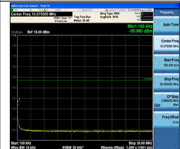
Band4-20MHz-QPSK-20300-1RB#0-0.15~30-PASS
