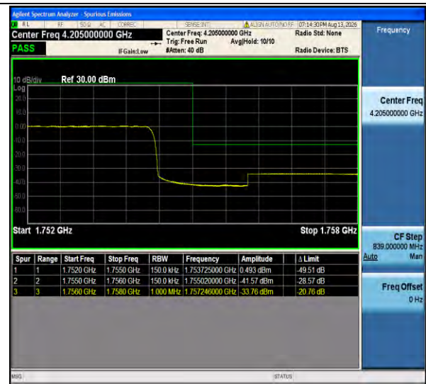
Band4-15MHz-QPSK-20325-75RB#0-PASS
