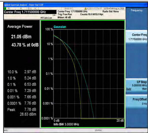
Band4-3MHz-16QAM-19965-15RB#0-PASS
