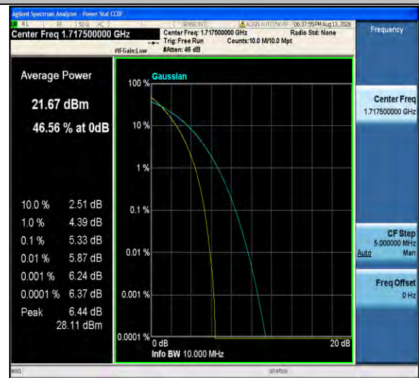
Band4-15MHz-QPSK-20025-75RB#0-PASS
