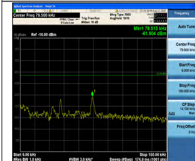
Band4-20MHz-QPSK-20300-1RB#0-0.009~0.15-PASS
