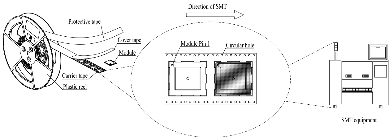
Figure 3: Mounting Direction
