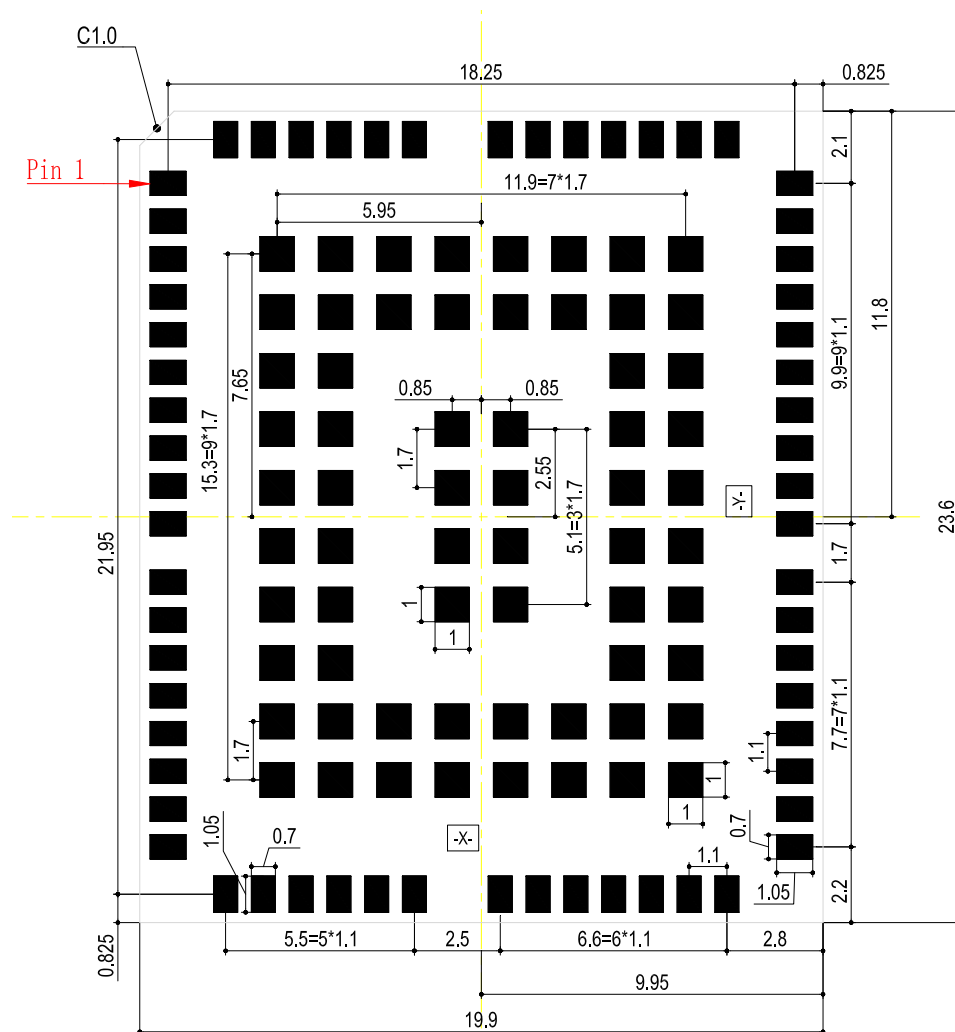
Figure 44: Recommended Footprint
