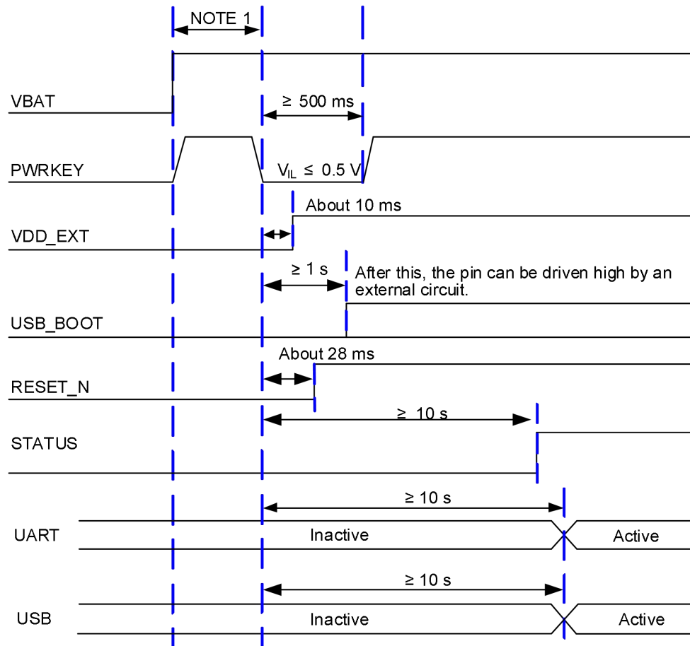
Figure 13: Power-up Timing
