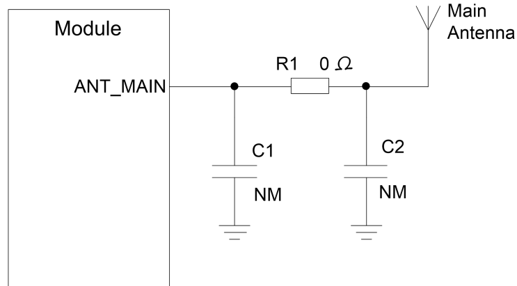
Figure 32: Reference Design for Main Antenna Interface
