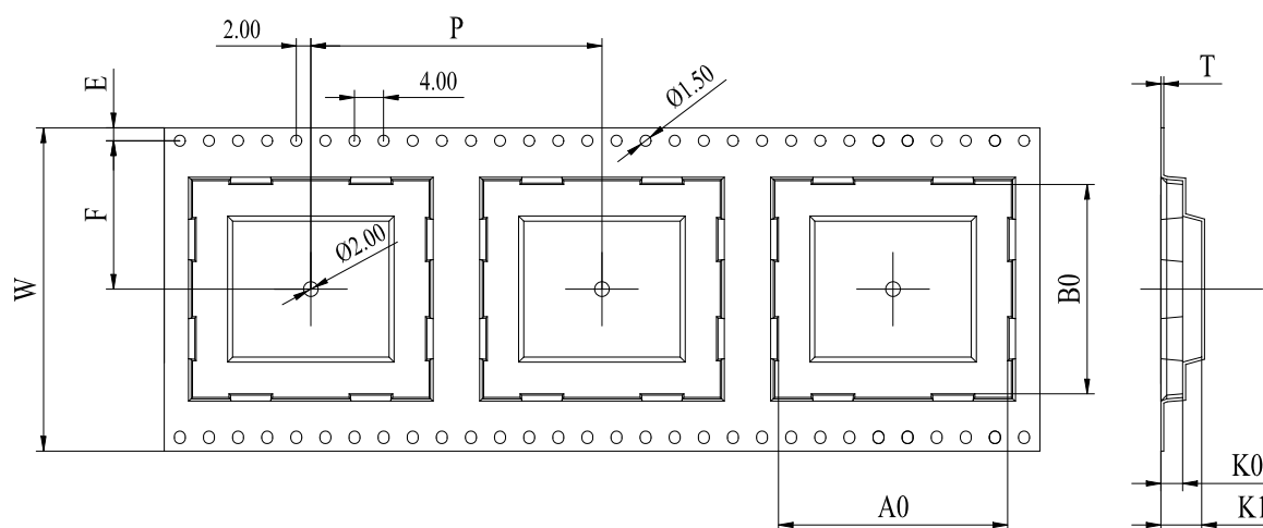
Figure 1: Carrier Tape Dimension Drawing (Unit: mm)
