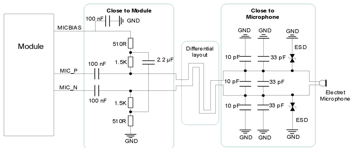
Figure 27: Reference Design for Microphone Interface
