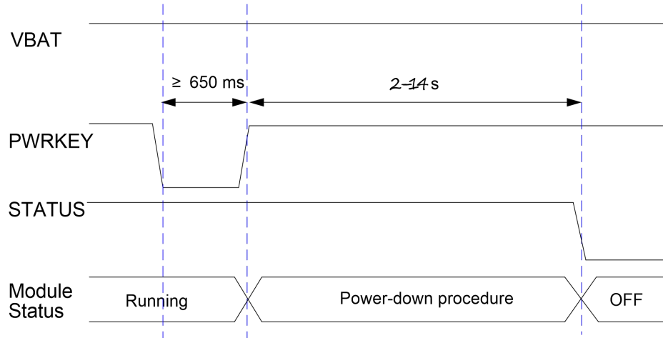
Figure 14: Power-down Timing
