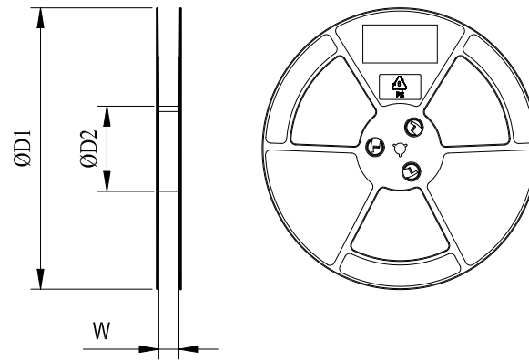
Figure 2: Plastic Reel Dimension Drawing
