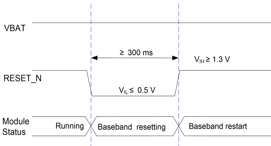
Figure 17: Reset Timing
