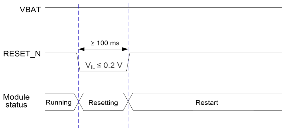
Figure 12: Reset Timing
