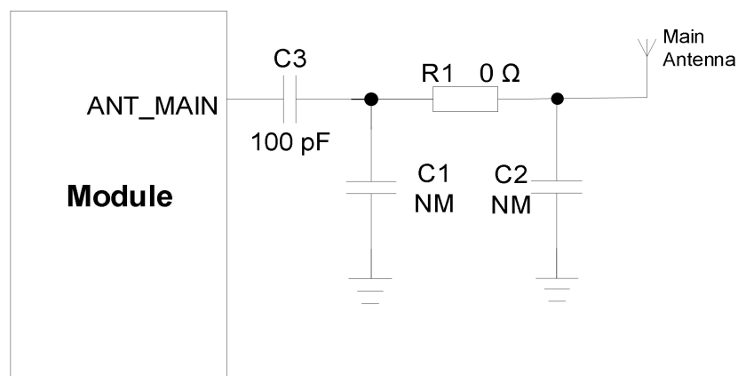
Figure 22: Reference Design of Main Antenna Interface
