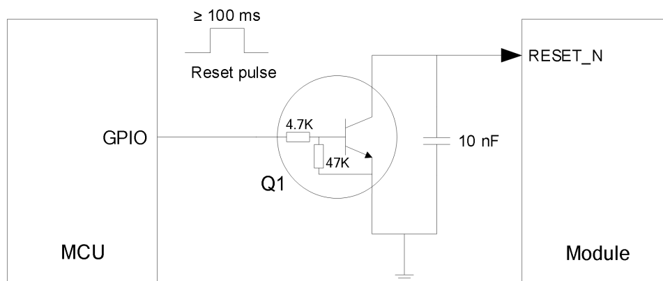
Figure 10: Reference Design of RESET_N with Driving Circuit
