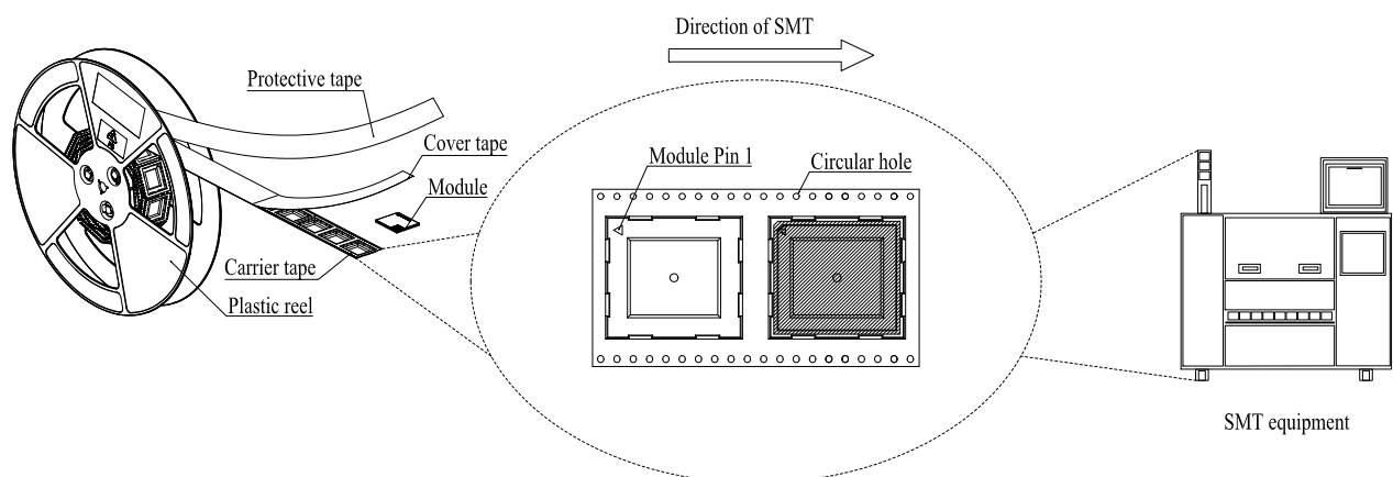
Figure 38: Mounting Direction
