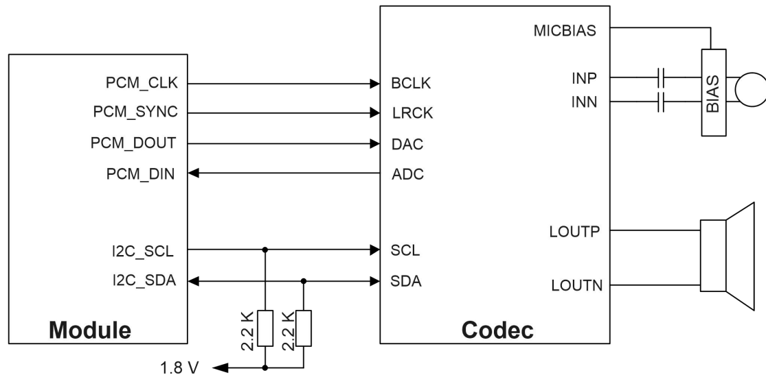
Figure 21: Reference Design of PCM and I2C Interfaces
