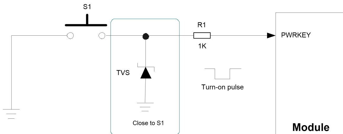
Figure 6: Turn On the Module with a Button
