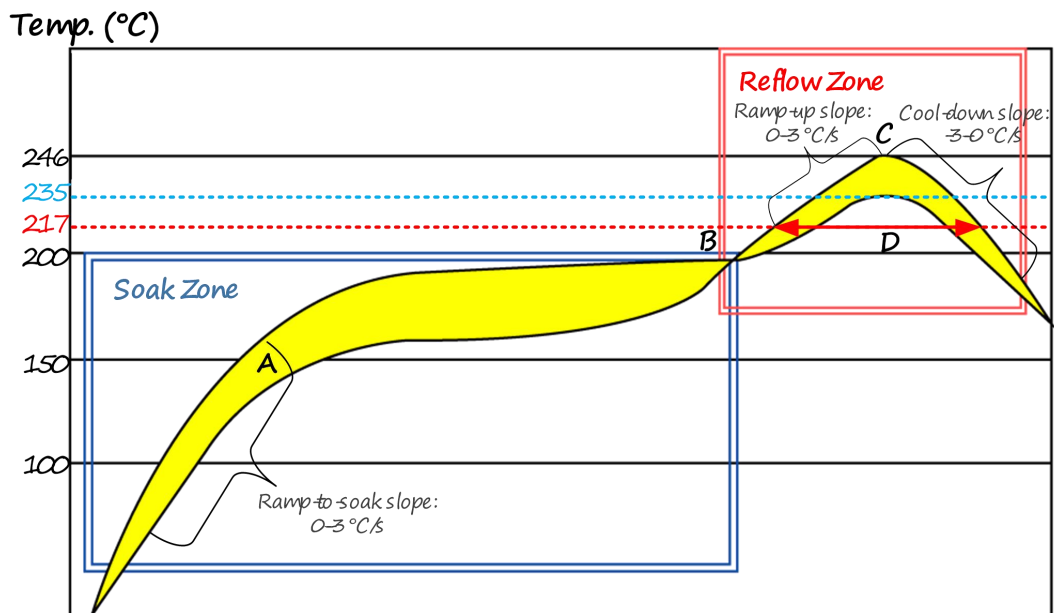
Figure 35: Recommended Reflow Soldering Thermal Profile
