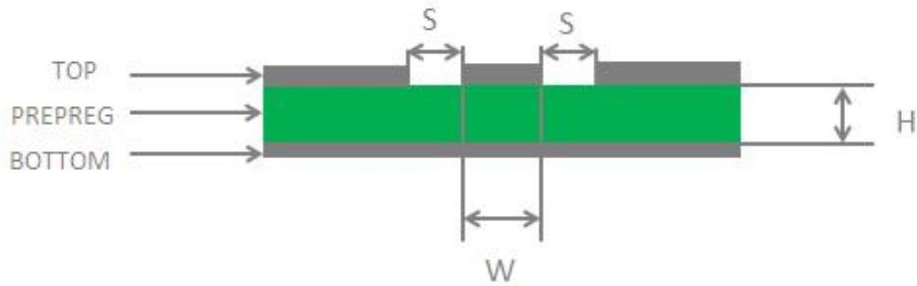
Figure 25: Coplanar Waveguide Design on a 2-layer PCB
