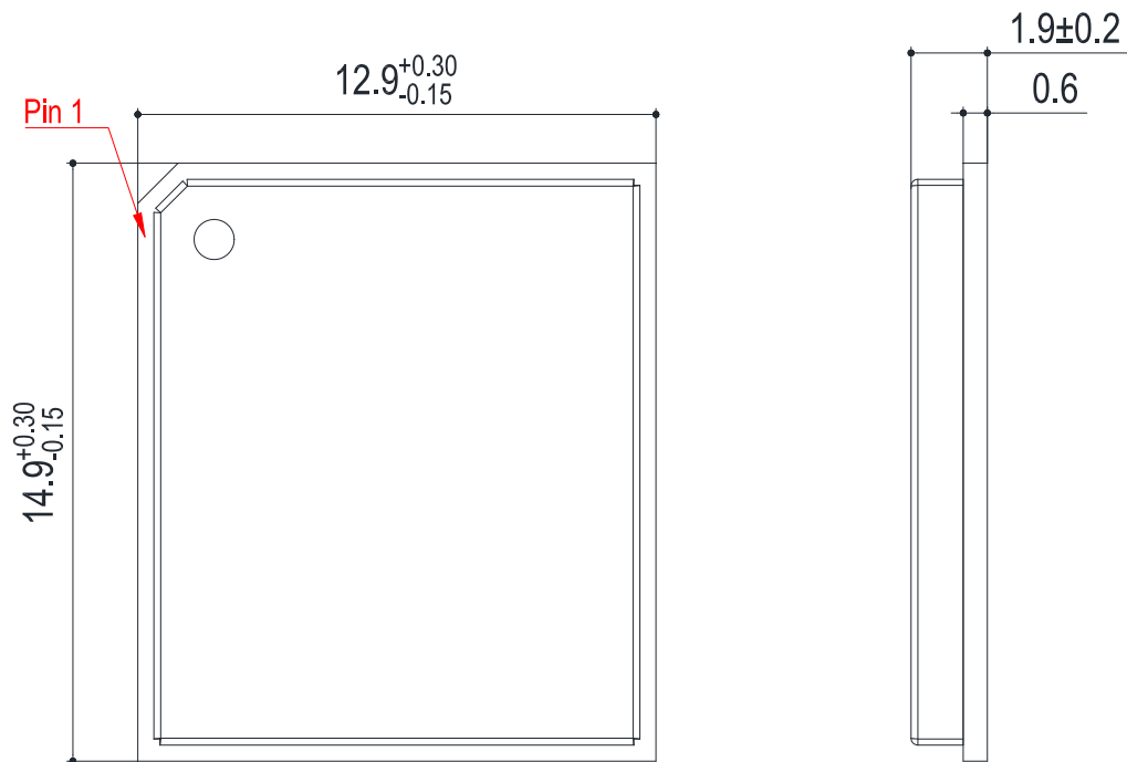
Figure 31: Module Top and Side Dimensions
