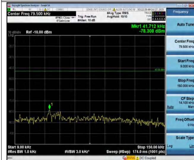
Band2-20MHz-QPSK-19100-1RB#0-0.009~0.15-PASS
