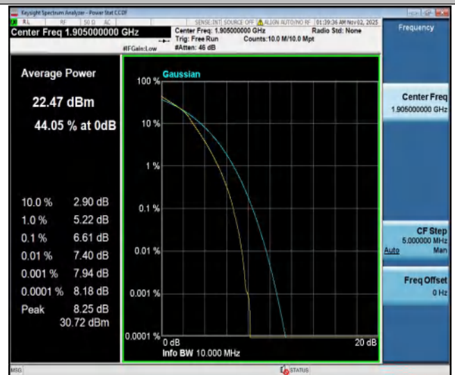
Band2-10MHz-16QAM-19150-27RB#0-PASS
