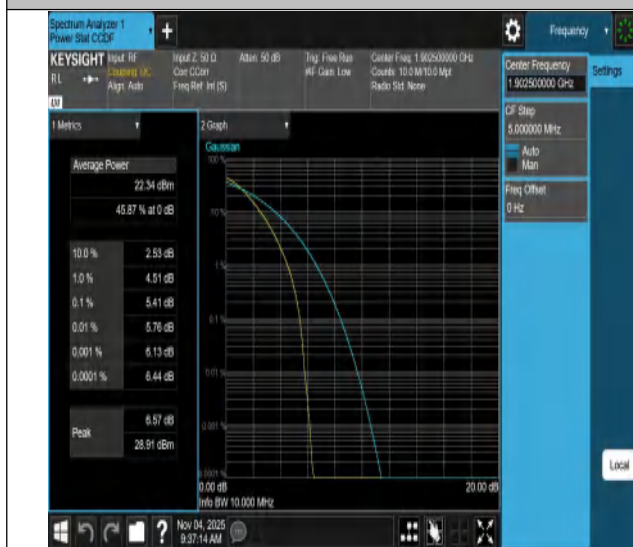
Band2-15MHz-QPSK-19125-75RB#0-PASS
