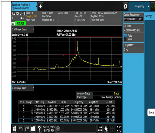
Band7-20MHz-QPSK-20850-1RB#0-PASS
