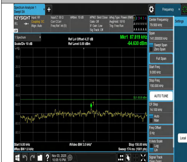
Band7-20MHz-QPSK-21350-1RB#0-0.009~0.15-PASS
