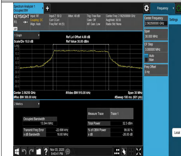
Band7-15MHz-QPSK-21375-75RB#0-PASS
