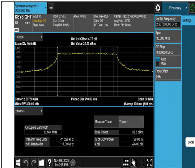
Band7-15MHz-QPSK-20825-75RB#0-PASS
