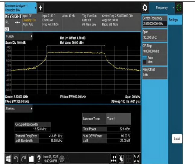
Band7-15MHz-QPSK-21100-75RB#0-PASS
