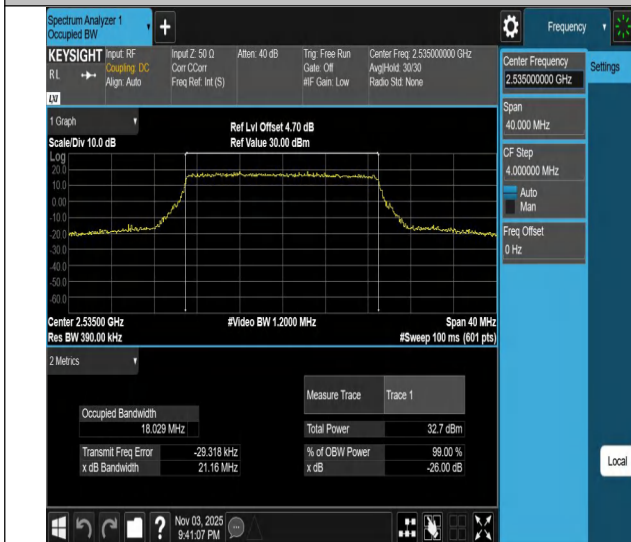
Band7-20MHz-QPSK-21100-100RB#0-PASS
