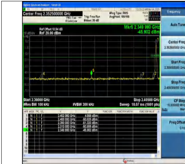
DH5-Ant1-2402-PASS
