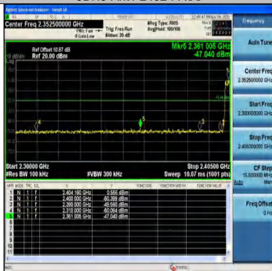
3DH5-Ant1-Hop_2402-PASS
