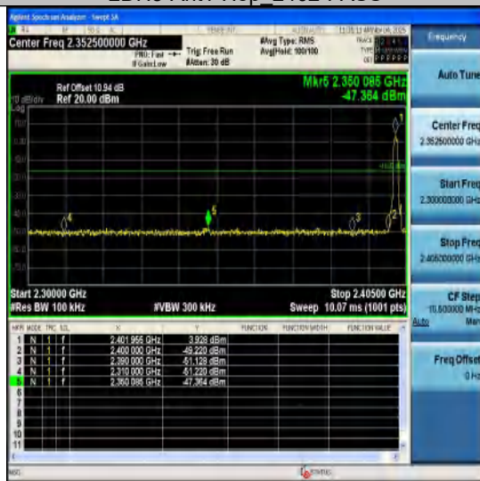
3DH5-Ant1-2402-PASS
