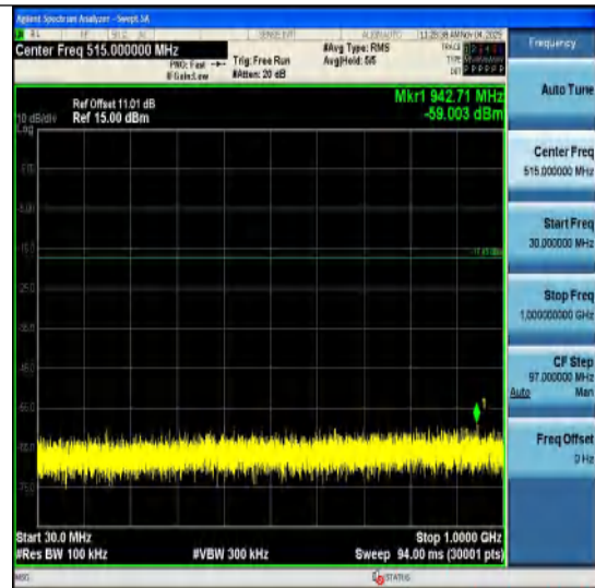
2DH5-Ant1-2441-30~1000-PASS
