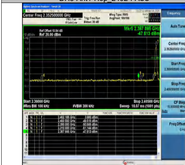
2DH5-Ant1-2402-PASS
