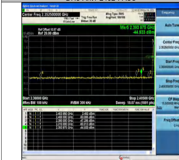
DH5-Ant1-Hop_2402-PASS
