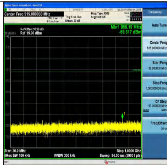
DH5-Ant1-2480-30~1000-PASS
