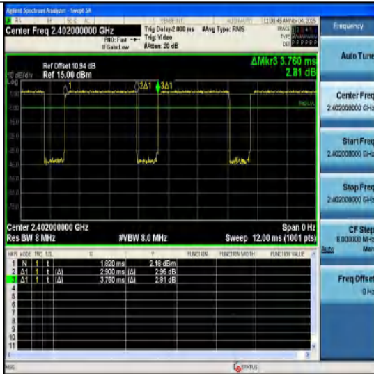
NTNV-3DH5-Ant1-2402
