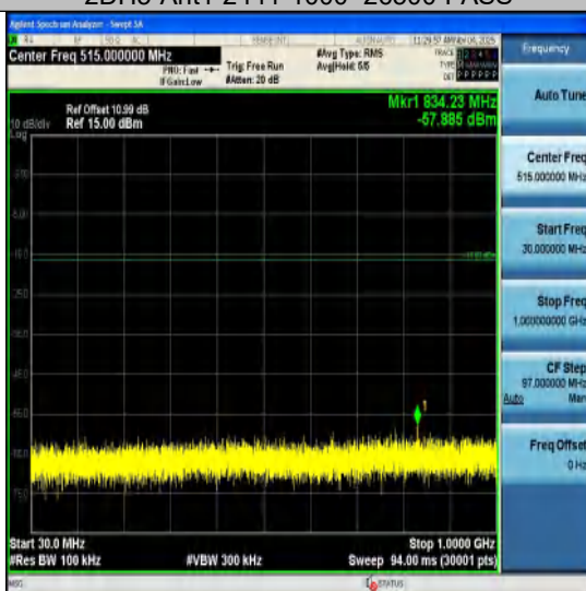
2DH5-Ant1-2480-30~1000-PASS
