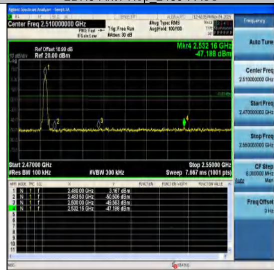
3DH5-Ant1-2480-PASS
