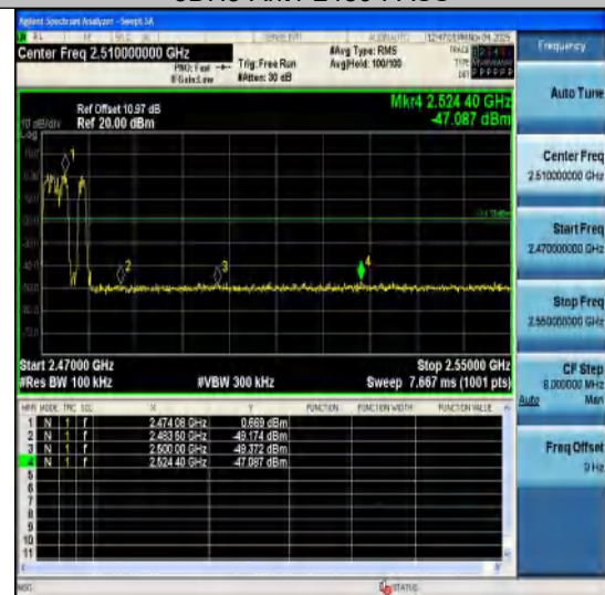
3DH5-Ant1-Hop_2480-PASS
