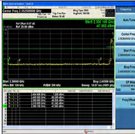
2DH5-Ant1-Hop_2402-PASS
