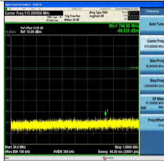
3DH5-Ant1-2480-30~1000-PASS
