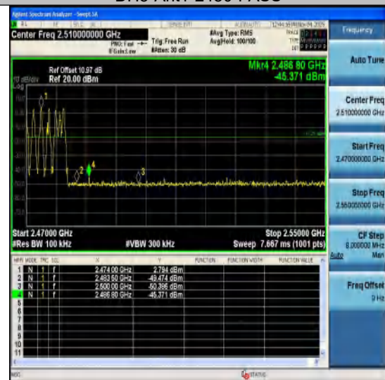
DH5-Ant1-Hop_2480-PASS
