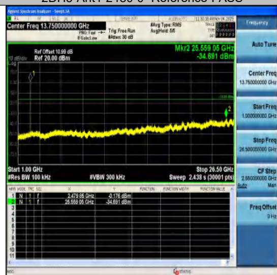
2DH5-Ant1-2480-1000~26500-PASS
