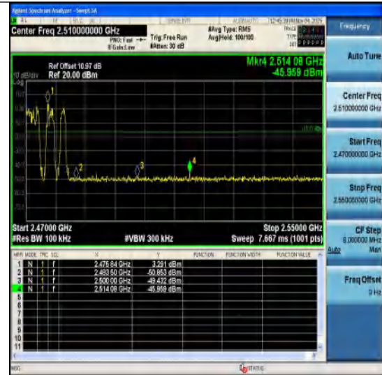
2DH5-Ant1-Hop_2480-PASS
