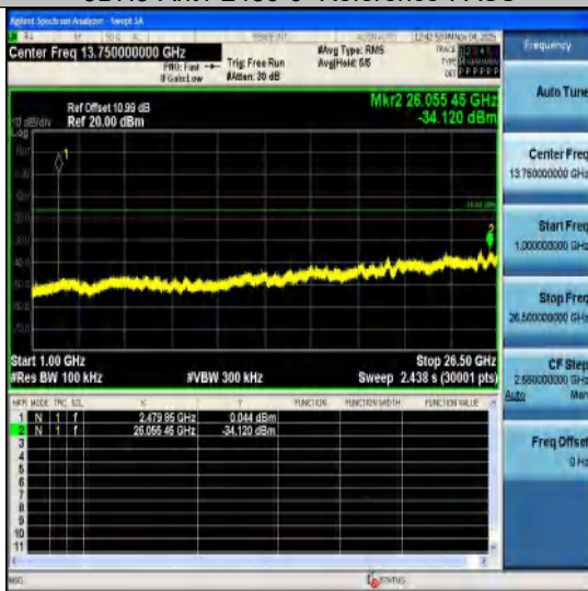
3DH5-Ant1-2480-1000~26500-PASS
