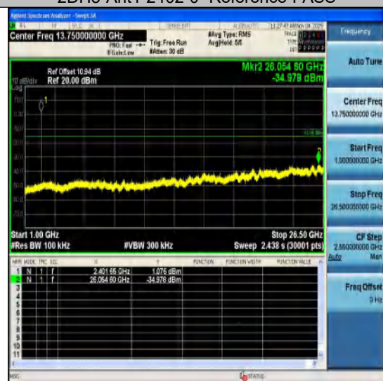
2DH5-Ant1-2402-1000~26500-PASS
