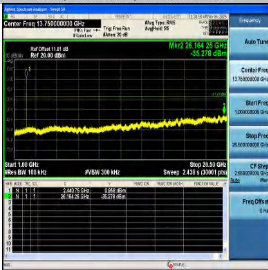
2DH5-Ant1-2441-1000~26500-PASS
