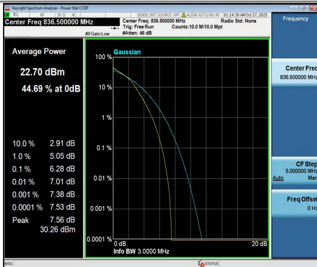
Band5-3MHz-16QAM-20525-15RB#0-PASS
