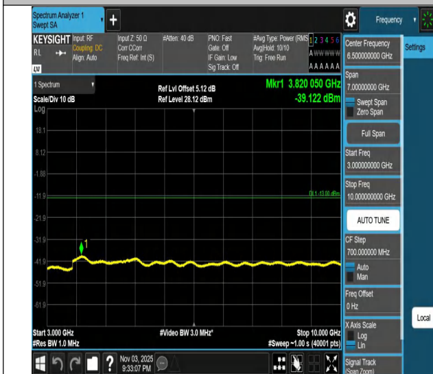
Band5-10MHz-QPSK-20600-1RB#0-3000~10000-PASS
