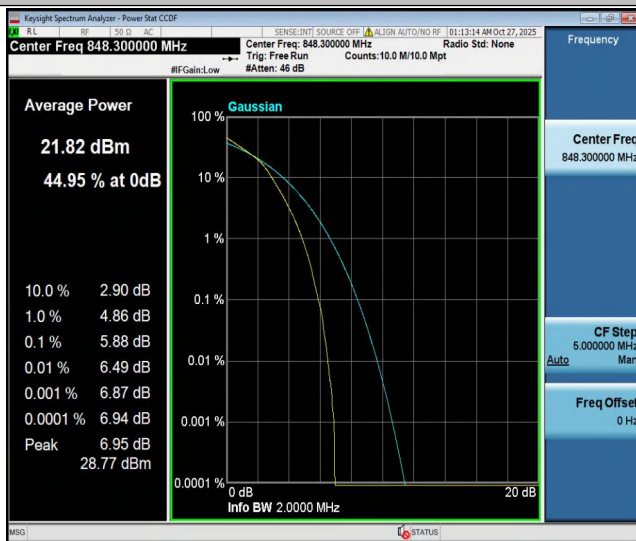
Band5-1.4MHz-16QAM-20643-6RB#0-PASS
