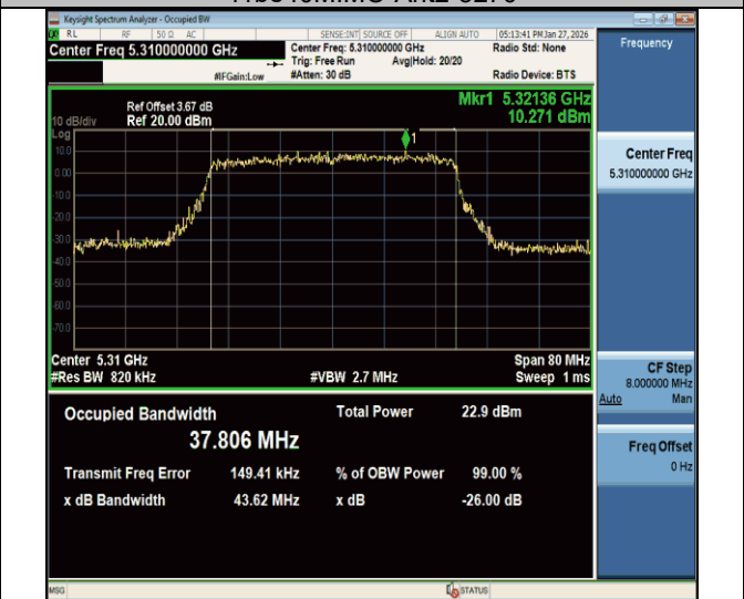
11be40MIMO-Ant2-5310
