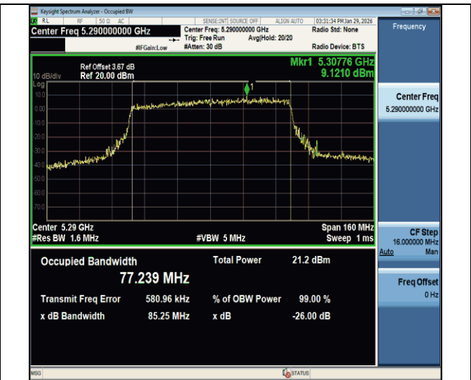
11be80MIMO-Ant2-5290
