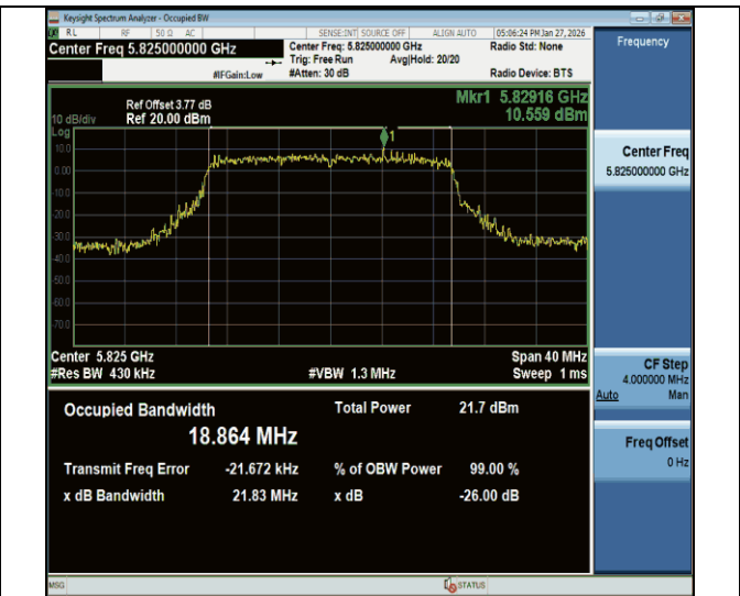
11be20MIMO-Ant2-5825
