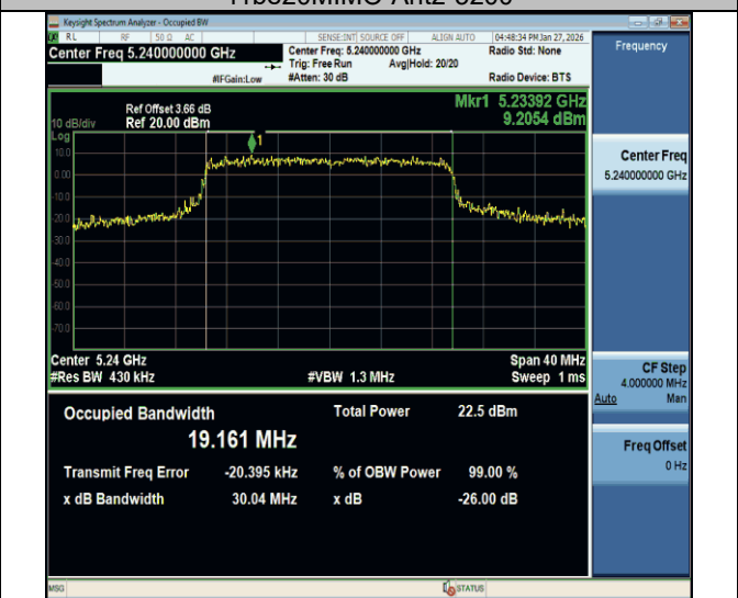
11be20MIMO-Ant2-5240
