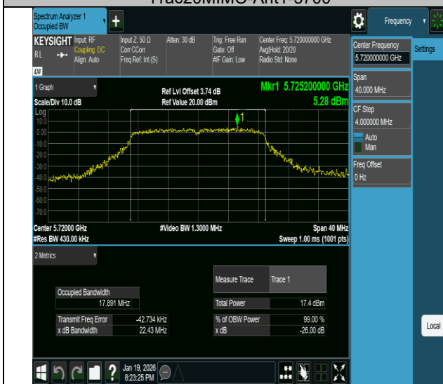
11ac20MIMO-Ant1-5720
