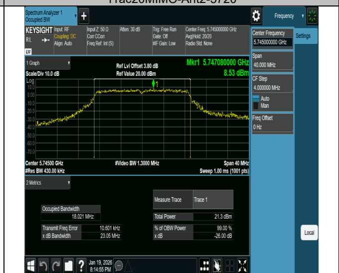
11ac20MIMO-Ant2-5745
