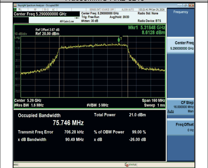
11ac80MIMO-Ant2-5290
