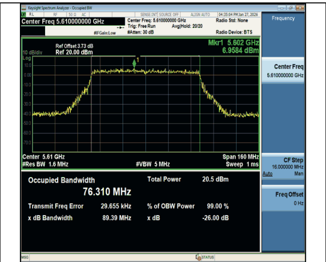
11ac80MIMO-Ant2-5610
