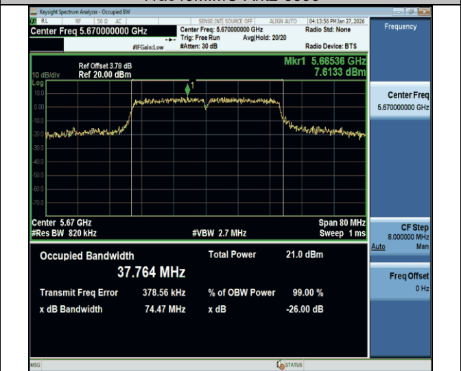
11ac40MIMO-Ant2-5670
