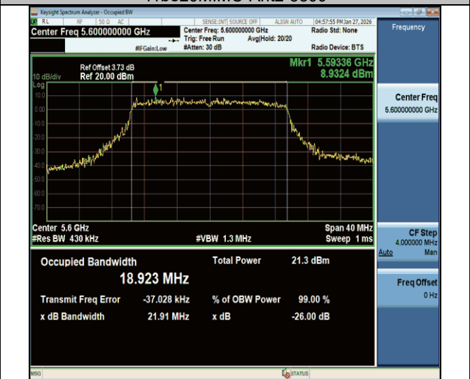
11be20MIMO-Ant2-5600
