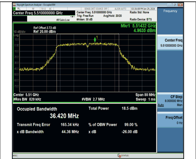
11ac40MIMO-Ant2-5510
