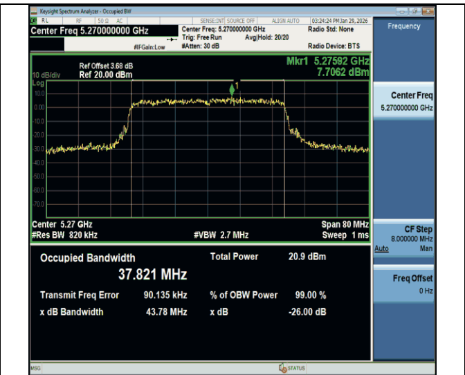
11be40MIMO-Ant2-5270
