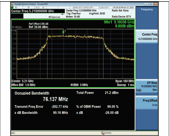
11ac80MIMO-Ant2-5210
