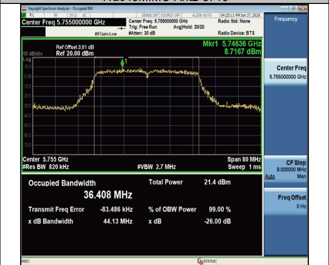
11ac40MIMO-Ant2-5755
