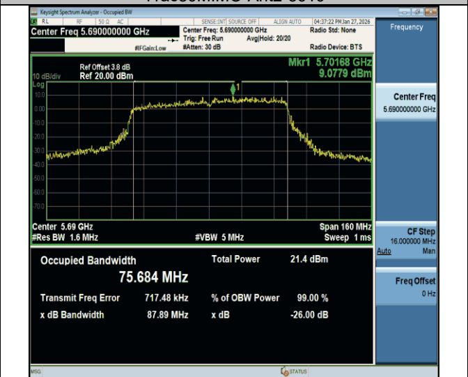
11ac80MIMO-Ant2-5690
