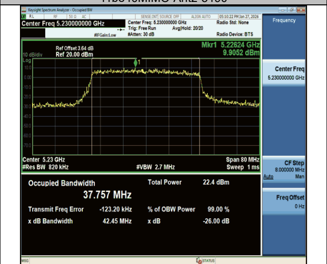
11be40MIMO-Ant2-5230
