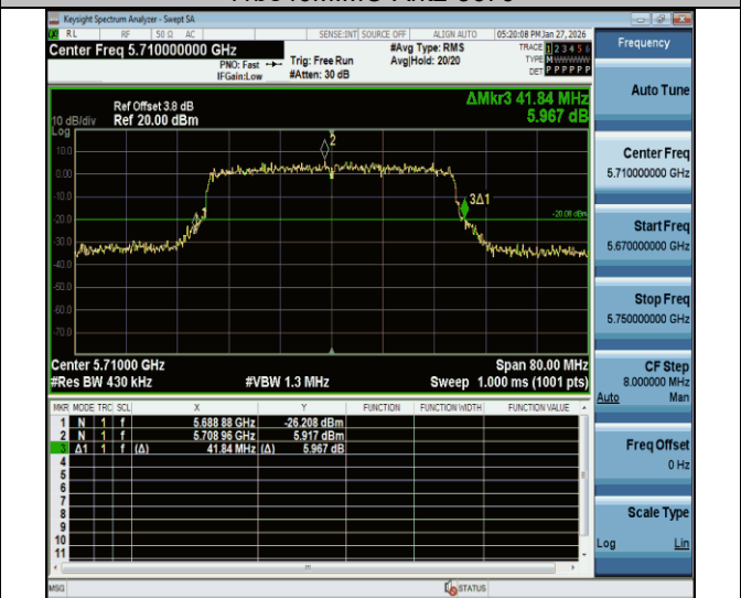
11be40MIMO-Ant2-5710
