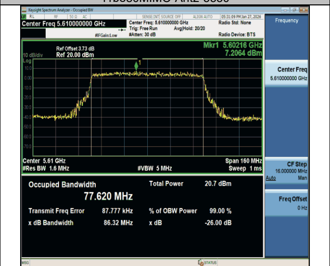
11be80MIMO-Ant2-5610
