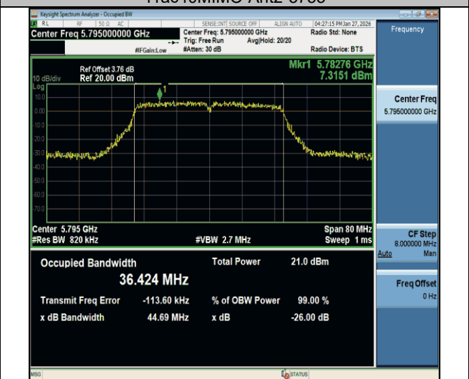
11ac40MIMO-Ant2-5795
