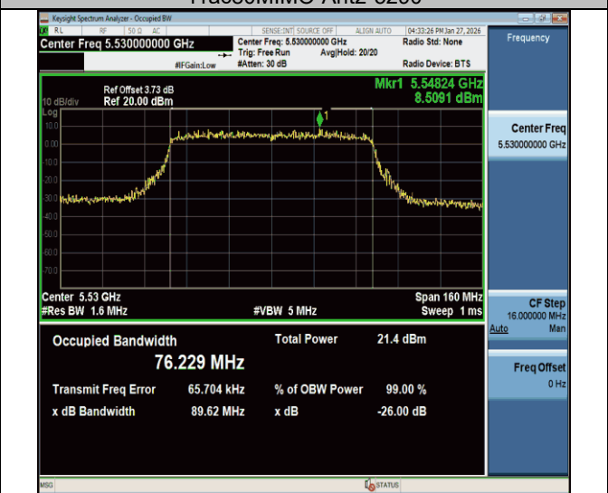
11ac80MIMO-Ant2-5530
