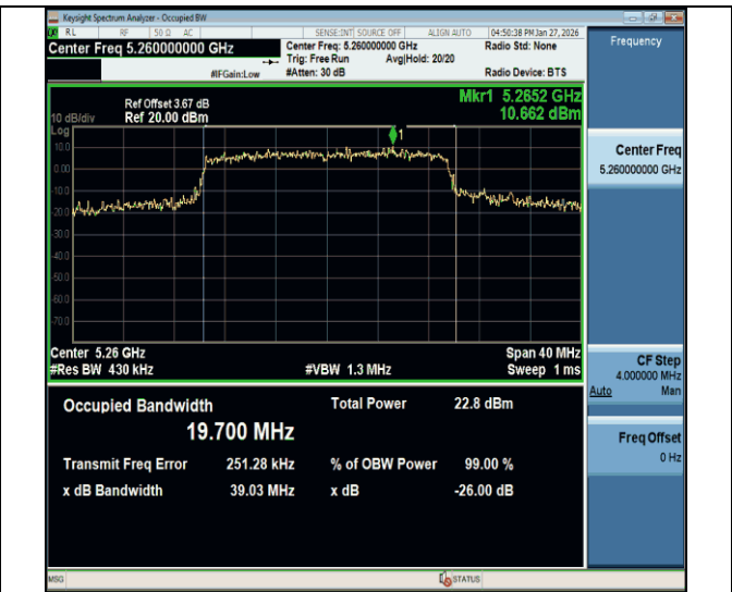
11be20MIMO-Ant2-5260
