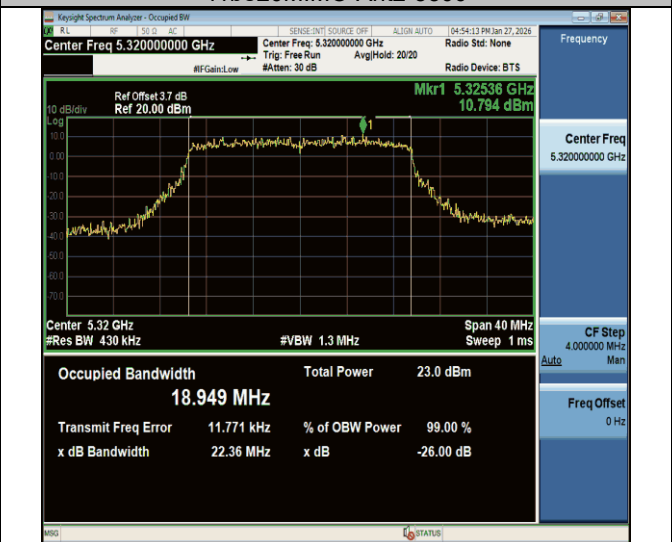
11be20MIMO-Ant2-5320
