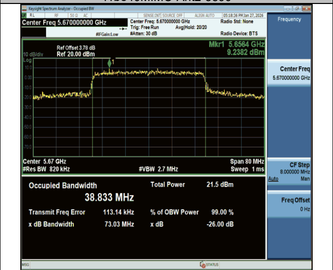
11be40MIMO-Ant2-5670
