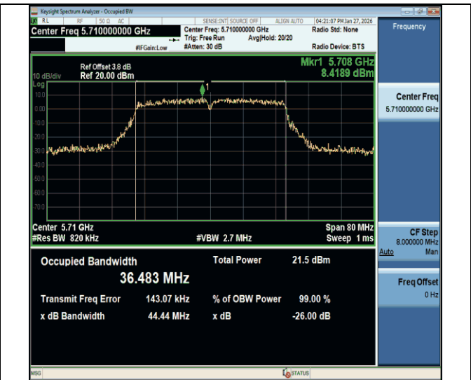
11ac40MIMO-Ant2-5710
