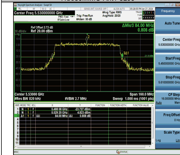
11be80MIMO-Ant1-5530
