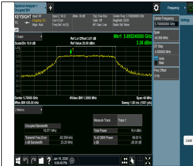
11ac20MIMO-Ant1-5700
