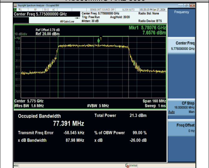
11be80MIMO-Ant2-5775
