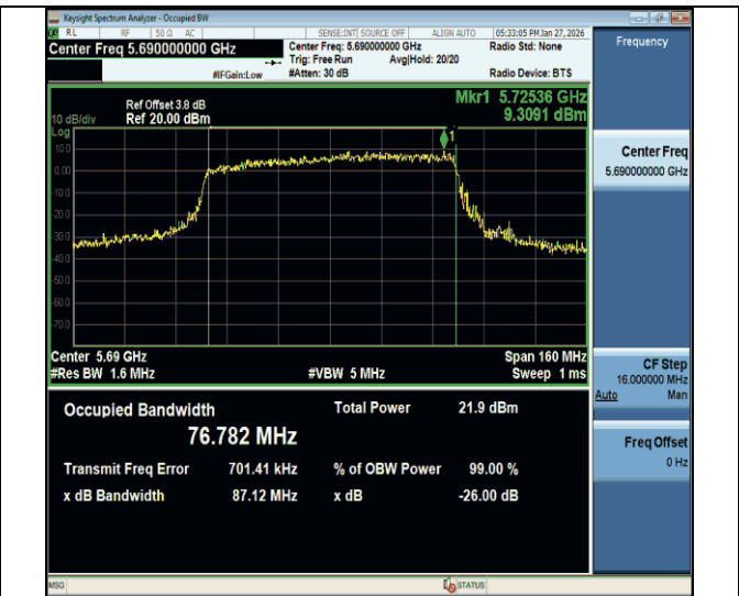
11be80MIMO-Ant2-5690
