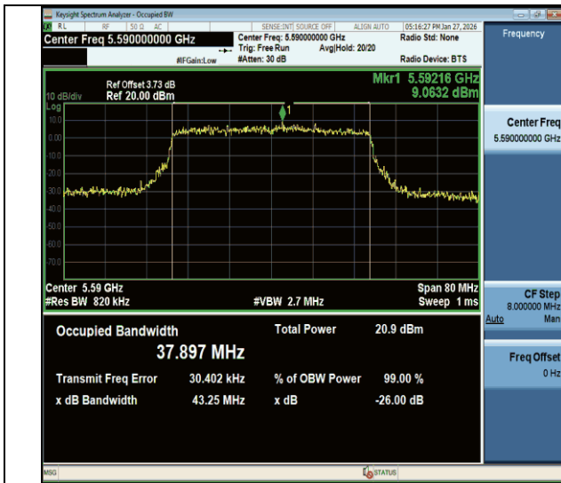
11be40MIMO-Ant1-5590
