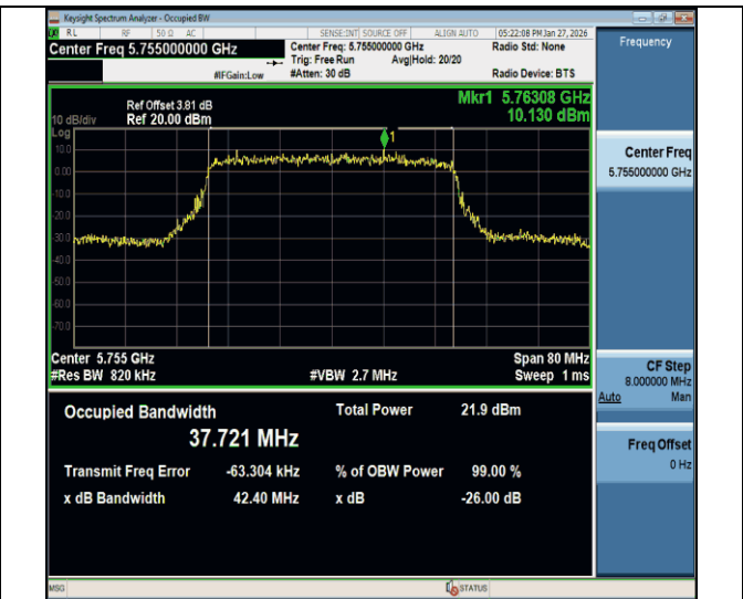
11be40MIMO-Ant2-5755
