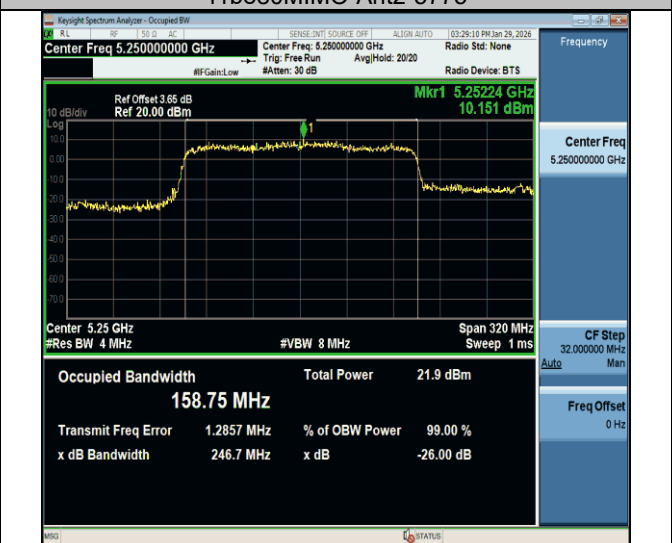
11be160MIMO-Ant2-5250
