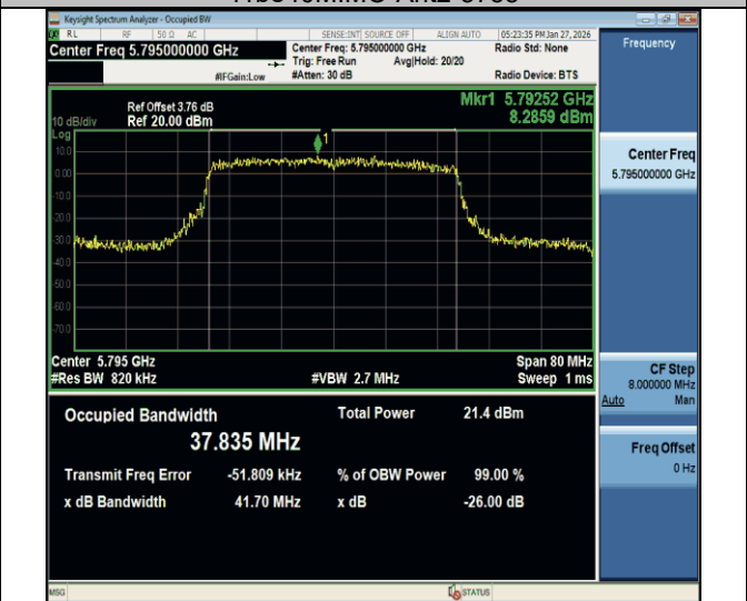
11be40MIMO-Ant2-5795
