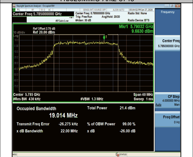
11be20MIMO-Ant2-5785
