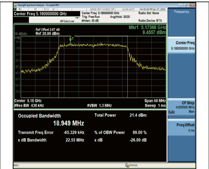
11be20MIMO-Ant2-5180
