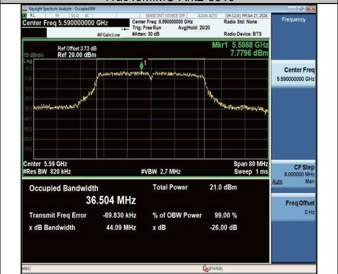
11ac40MIMO-Ant2-5590
