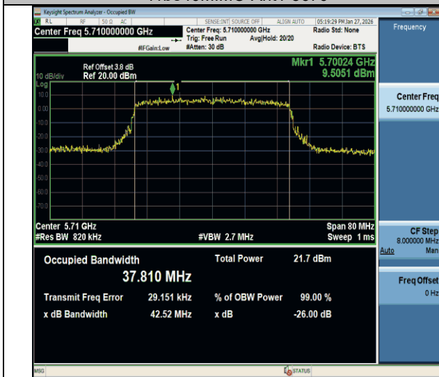
11be40MIMO-Ant1-5710
