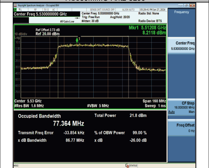
11be80MIMO-Ant2-5530
