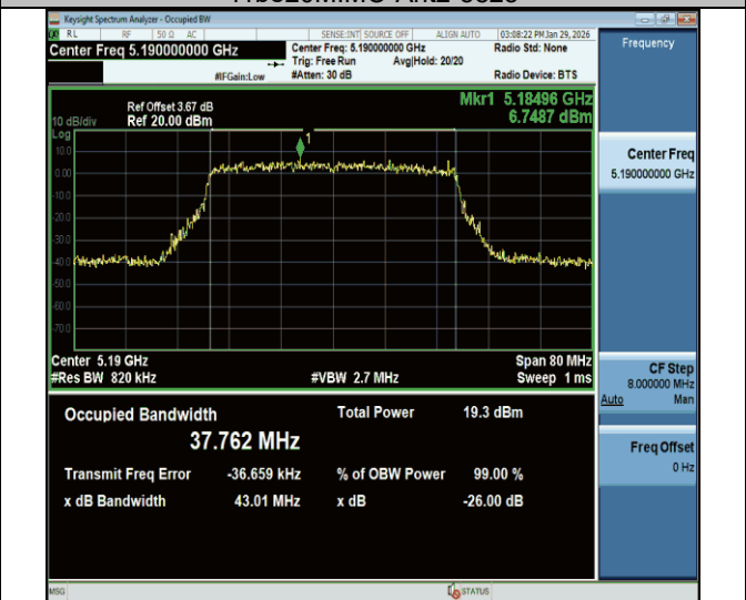
11be40MIMO-Ant2-5190
