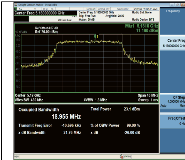
11be20MIMO-Ant1-5180
