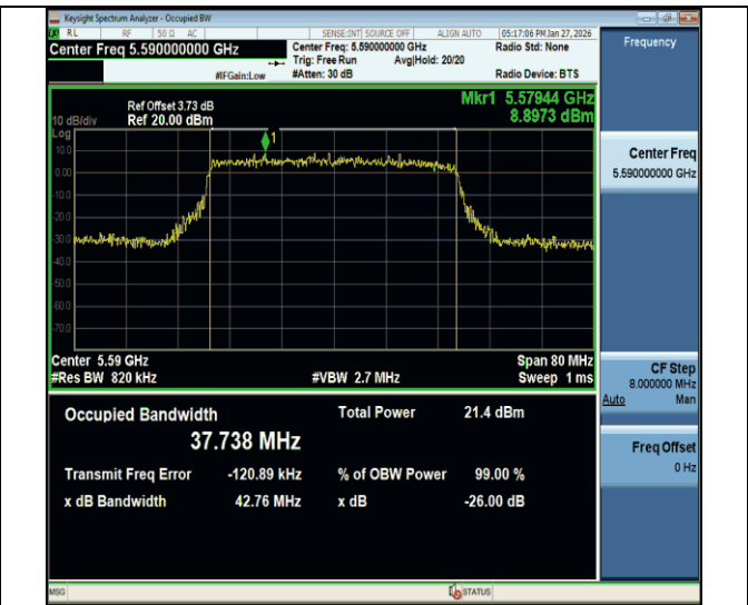
11be40MIMO-Ant2-5590
