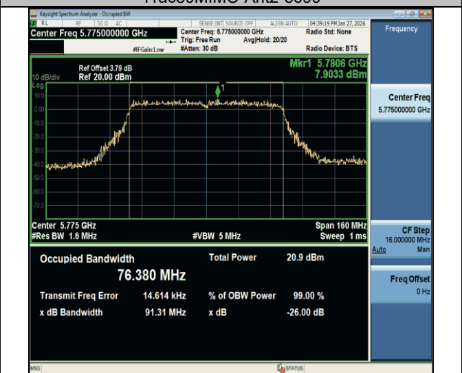
11ac80MIMO-Ant2-5775
