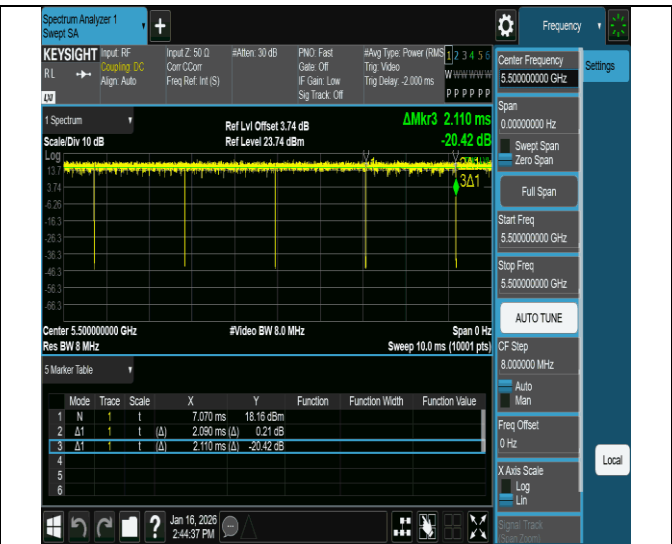
NTNV-11a-CDD-Ant2-5500
