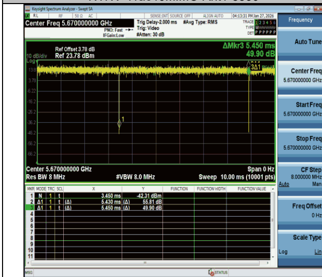
NTNV-11ac40MIMO-Ant1-5670
