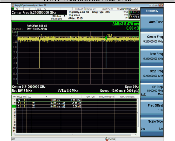
NTNV-11be80MIMO-Ant2-5210
