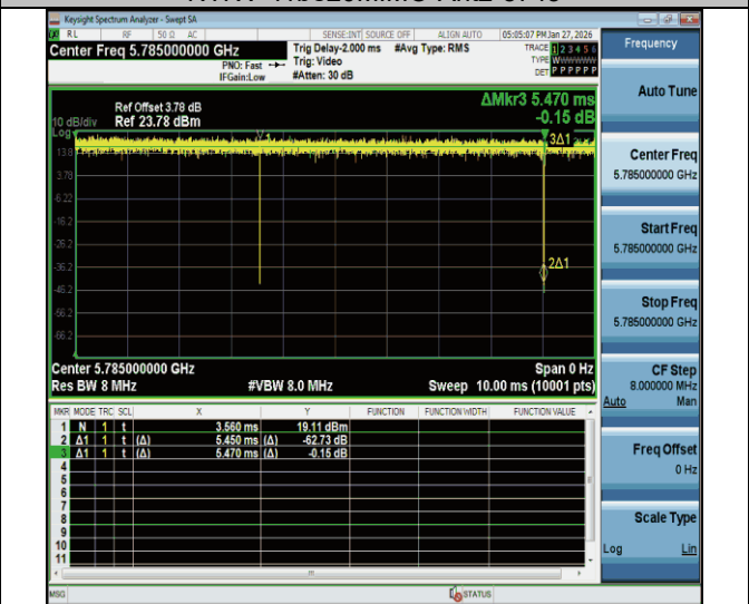
NTNV-11be20MIMO-Ant2-5785
