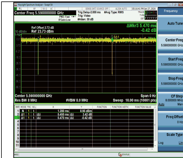
NTNV-11be40MIMO-Ant1-5590
