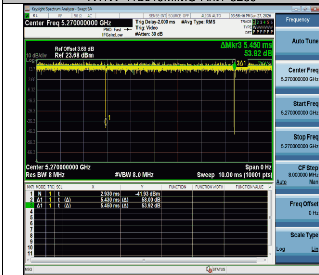
NTNV-11ac40MIMO-Ant1-5270
