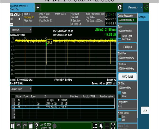
NTNV-11a-CDD-Ant2-5700
