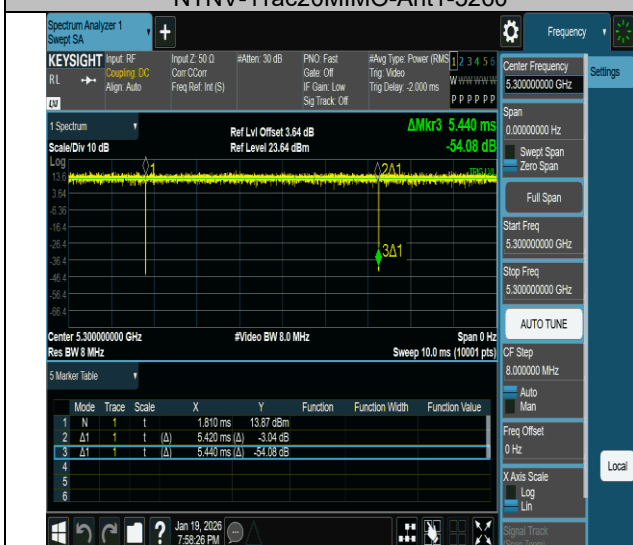
NTNV-11ac20MIMO-Ant1-5300
