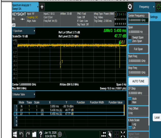
NTVN-11ac20MIMO-Ant1-5600
