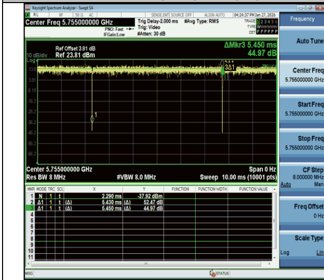
NTNV-11ac40MIMO-Ant1-5755
