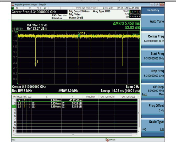
NTNV-11ac40MIMO-Ant2-5310
