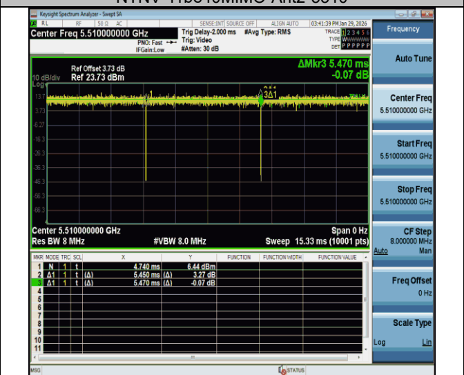
NTNV-11be40MIMO-Ant2-5510
