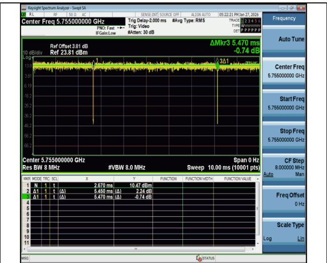
NTNV-11be40MIMO-Ant2-5755
