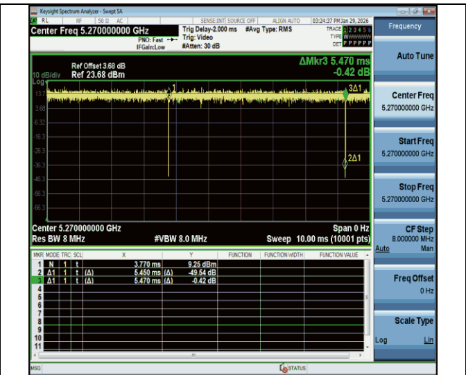
NTNV-11be40MIMO-Ant2-5270
