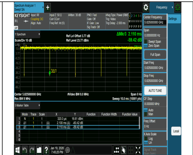
NTNV-11a-CDD-Ant2-5825
