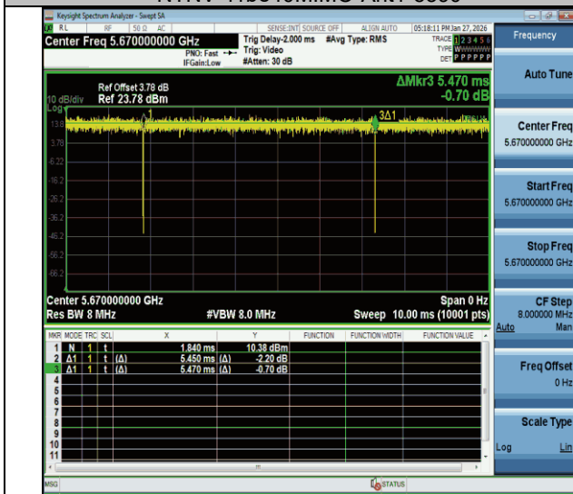
NTNV-11be40MIMO-Ant1-5670
