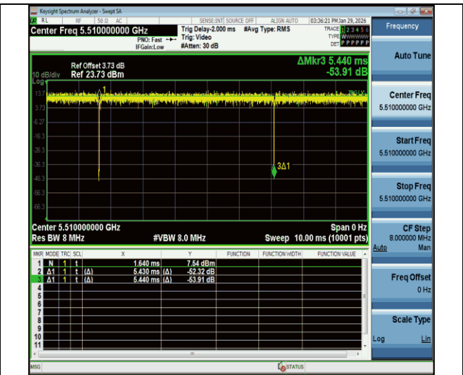
NTNV-11ac40MIMO-Ant2-5510
