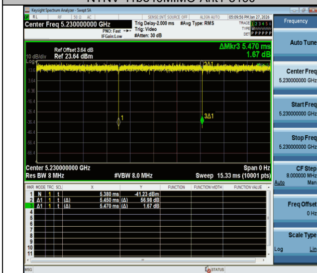
NTNV-11be40MIMO-Ant1-5230
