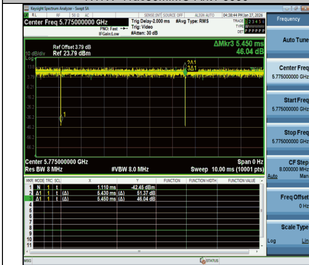
NTNV-11ac80MIMO-Ant1-5775
