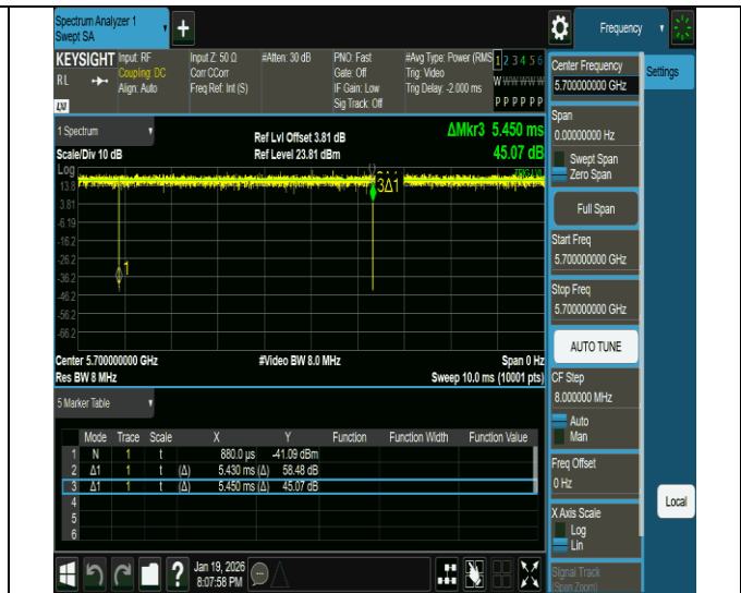
NTNV-11ac20MIMO-Ant2-5700
