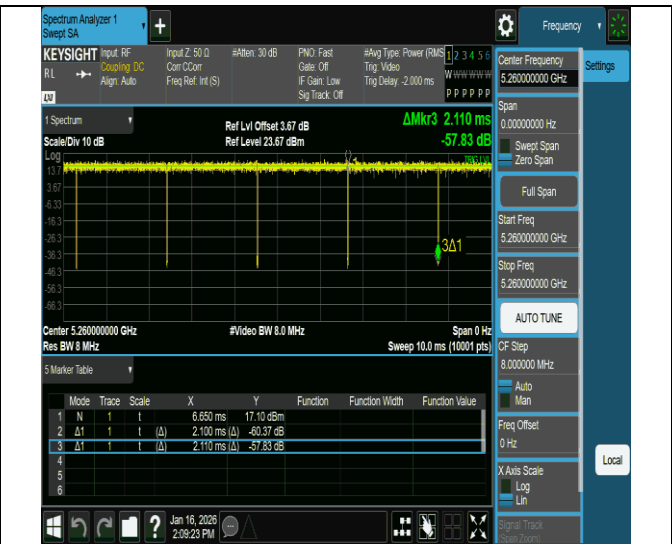
NTNV-11a-CDD-Ant2-5260
