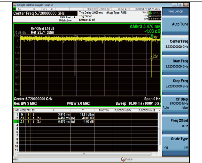
NTNV-11be20MIMO-Ant2-5720
