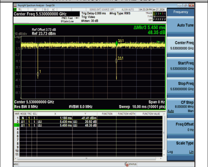
NTNV-11ac80MIMO-Ant2-5530
