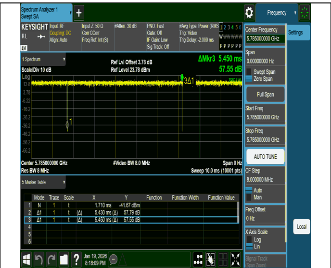
NTVN-11ac20MIMO-Ant2-5785
