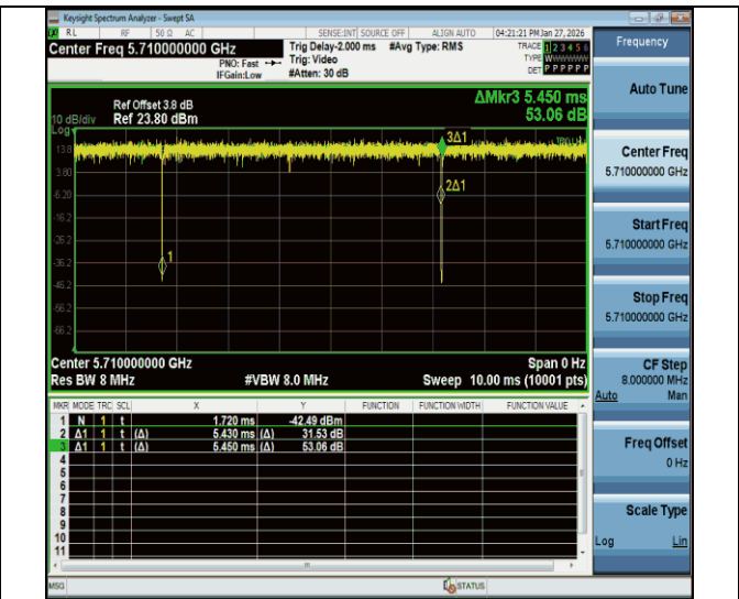
NTNV-11ac40MIMO-Ant2-5710
