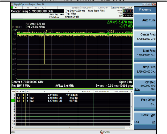
NTNV-11be40MIMO-Ant2-5795
