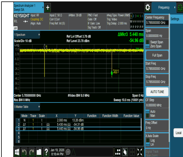
NTVN-11ac20MIMO-Ant1-5785
