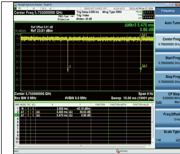
NTNV-11be40MIMO-Ant1-5755
