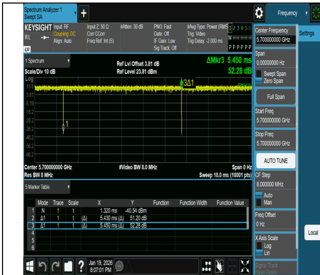
NTNV-11ac20MIMO-Ant1-5700
