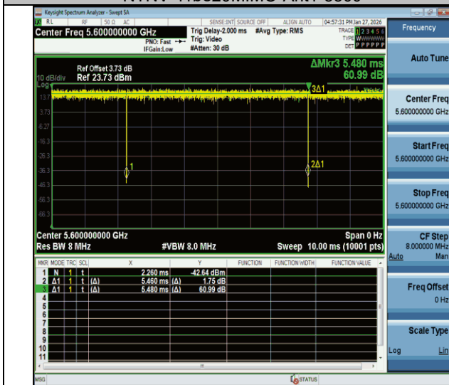
NTNV-11be20MIMO-Ant1-5600
