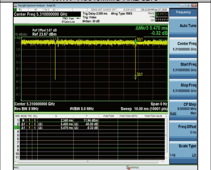
NTNV-11be40MIMO-Ant2-5310
