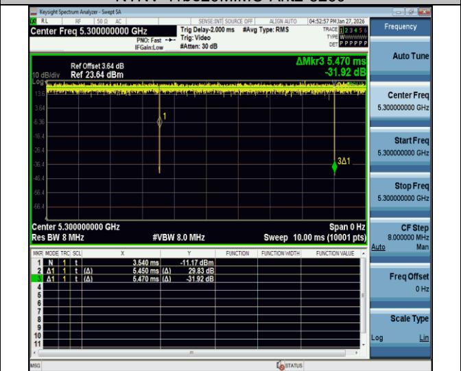
NTNV-11be20MIMO-Ant2-5300
