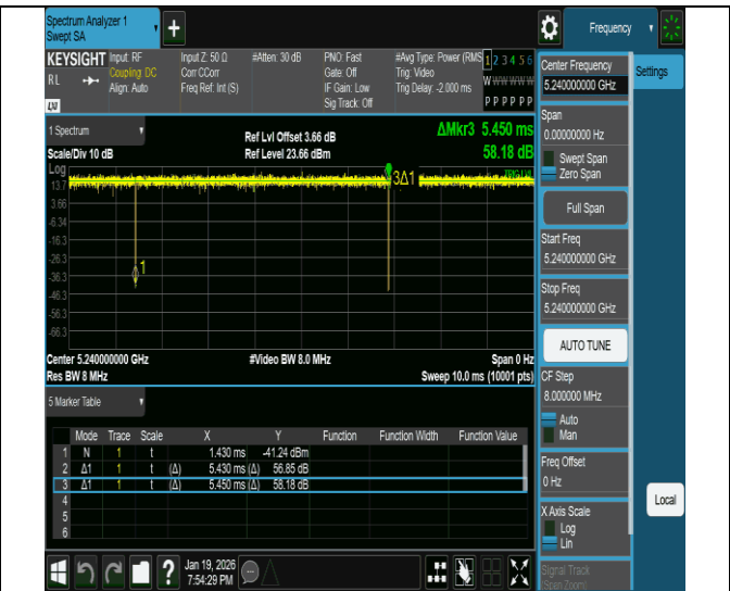
NTNV-11ac20MIMO-Ant2-5240
