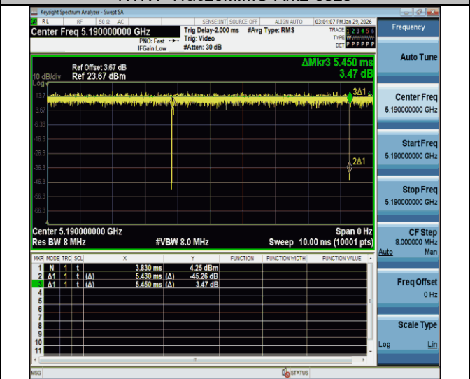
NTVN-11ac40MIMO-Ant2-5190
