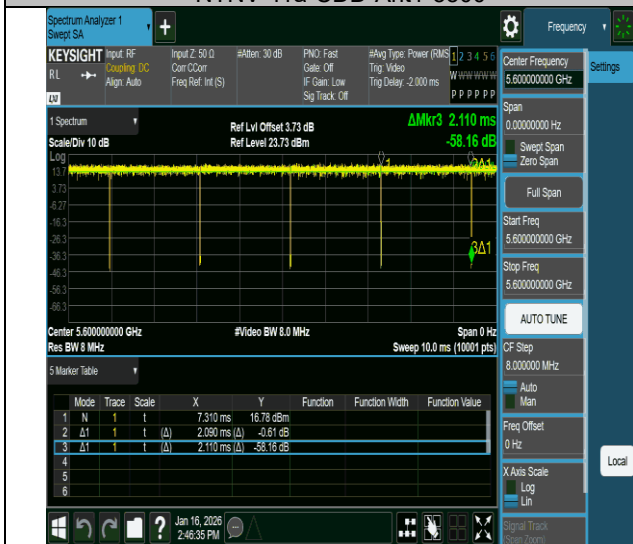
NTNV-11a-CDD-Ant1-5600
