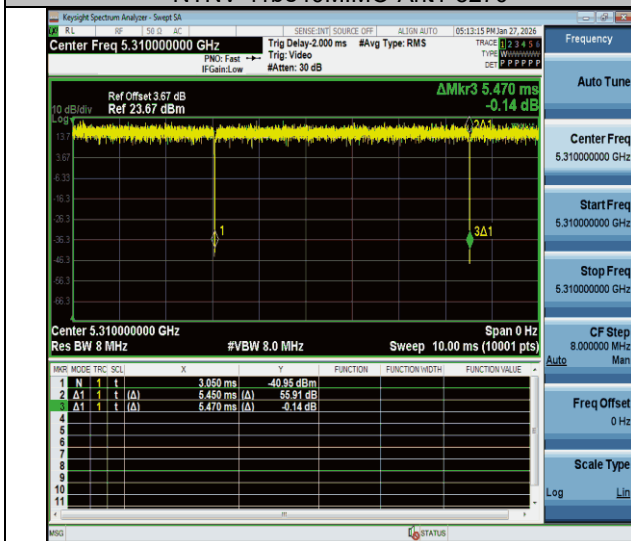
NTNV-11be40MIMO-Ant1-5310
