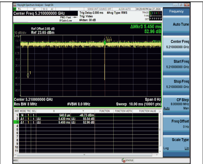
NTNV-11ac80MIMO-Ant2-5210
