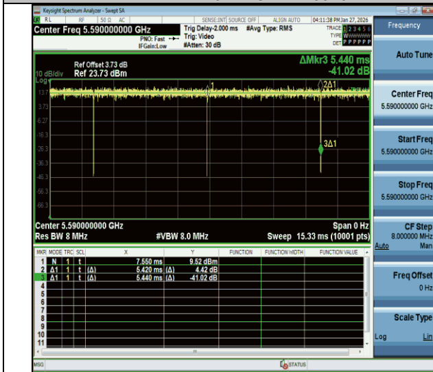
NTNV-11ac40MIMO-Ant1-5590
