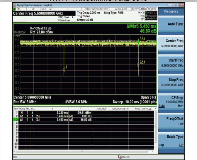
NTNV-11ac80MIMO-Ant2-5690
