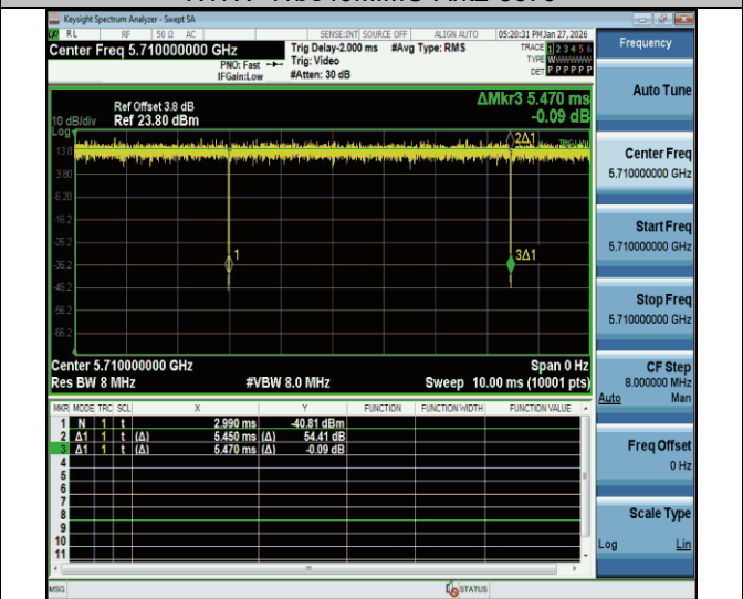
NTNV-11be40MIMO-Ant2-5710
