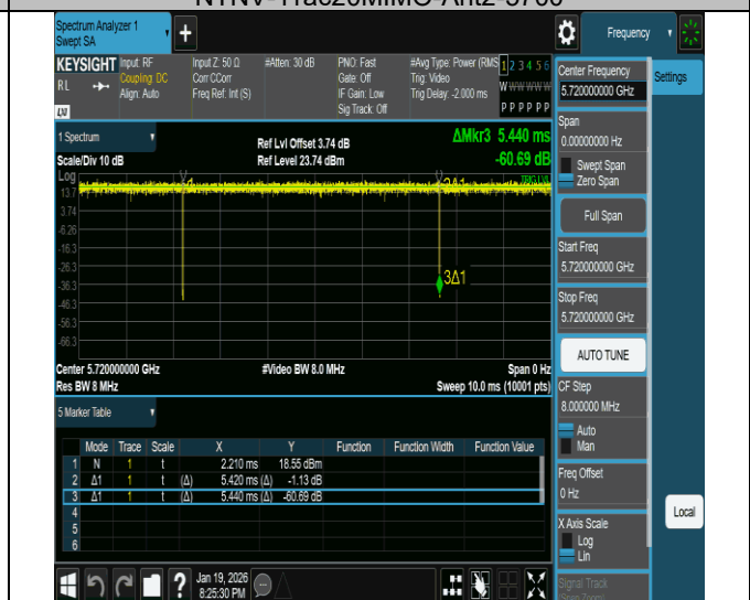
NTNV-11ac20MIMO-Ant2-5720
