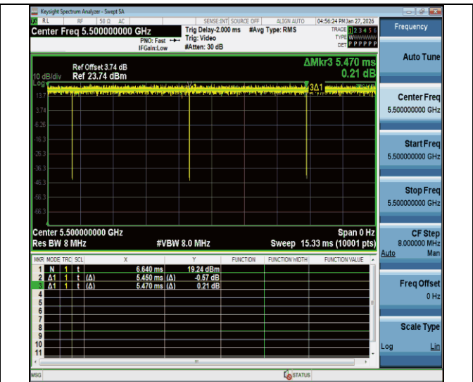
NTNV-11be20MIMO-Ant2-5500
