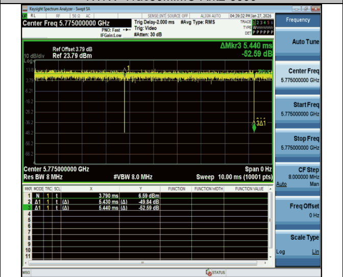
NTNV-11ac80MIMO-Ant2-5775
