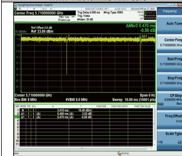
NTNV-11be40MIMO-Ant1-5710
