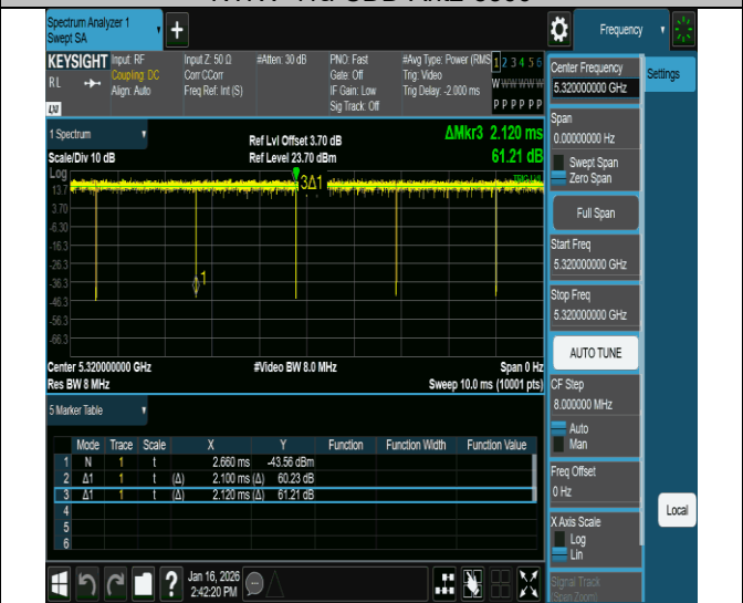
NTNV-11a-CDD-Ant2-5320
