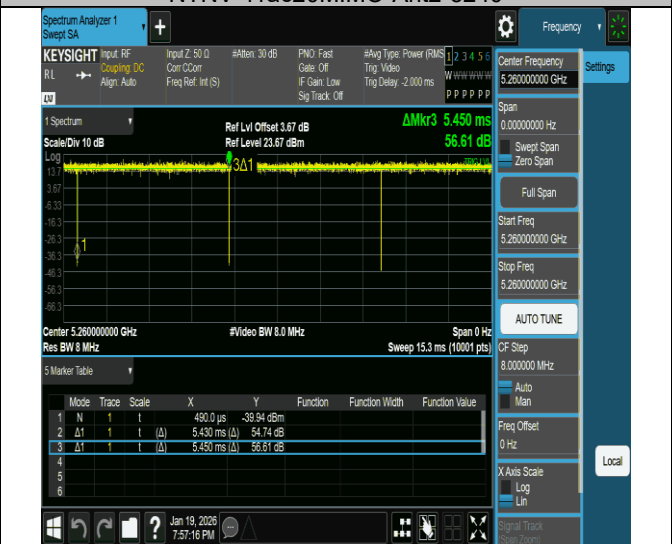
NTNV-11ac20MIMO-Ant2-5260
