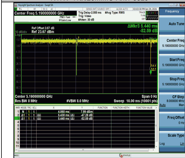
NTVN-11ac40MIMO-Ant1-5190
