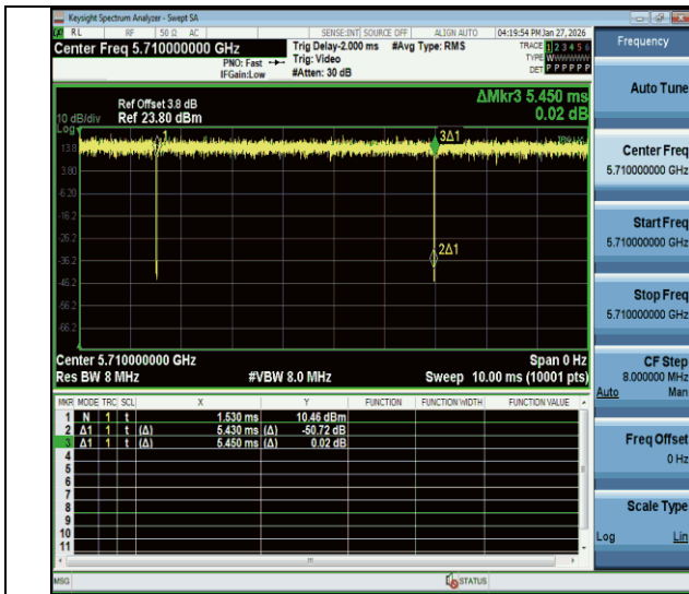
NTNV-11ac40MIMO-Ant1-5710
