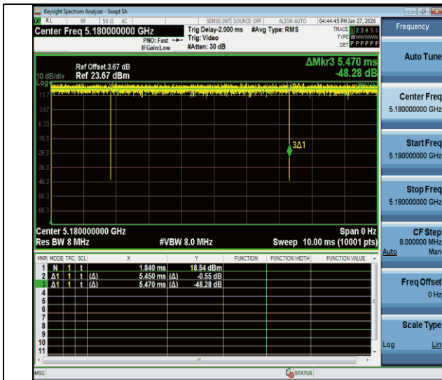
NTNV-11be20MIMO-Ant1-5180
