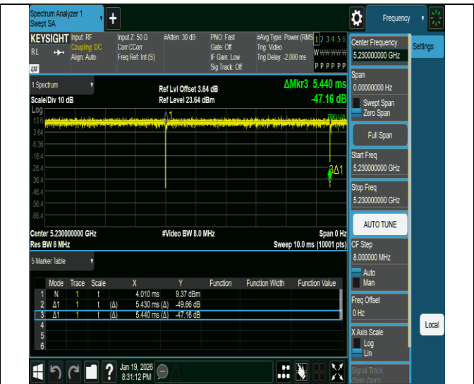
NTNV-11ac40MIMO-Ant2-5230
