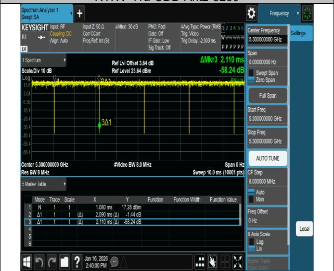
NTNV-11a-CDD-Ant2-5300
