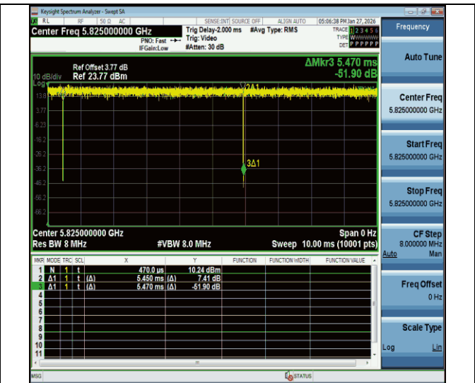
NTNV-11be20MIMO-Ant2-5825
