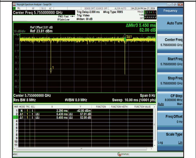
NTNV-11ac40MIMO-Ant2-5755
