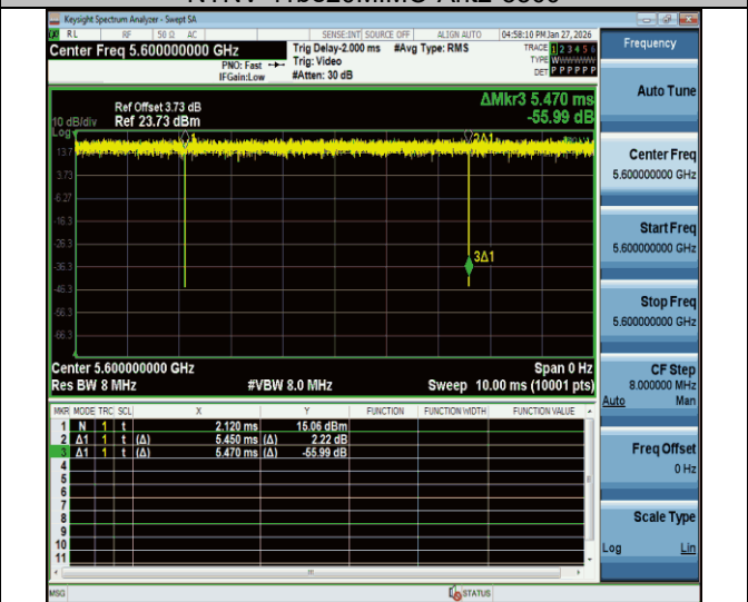
NTNV-11be20MIMO-Ant2-5600
