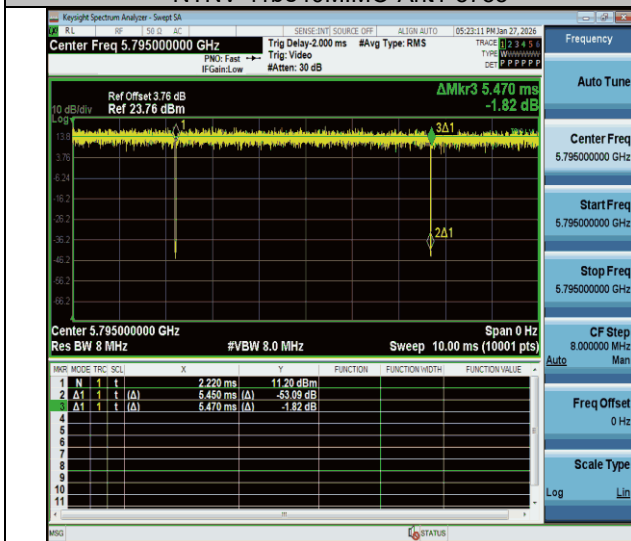
NTNV-11be40MIMO-Ant1-5795
