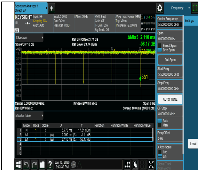
NTNV-11a-CDD-Ant1-5500
