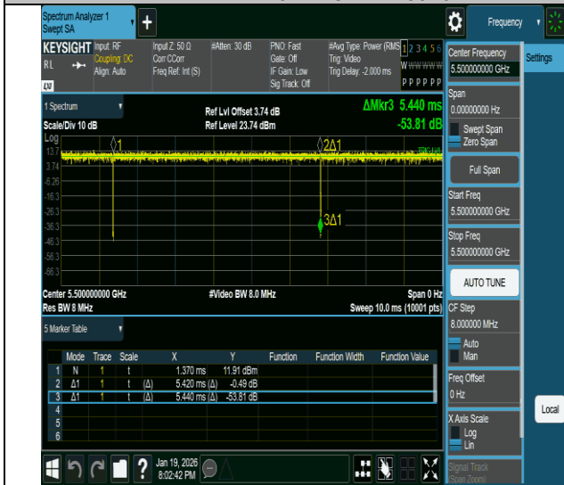
NTVN-11ac20MIMO-Ant1-5500
