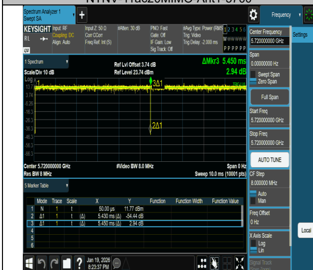
NTNV-11ac20MIMO-Ant1-5720
