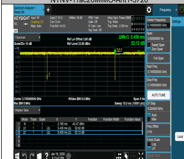
NTNV-11ac20MIMO-Ant1-5745
