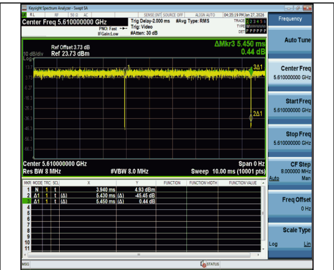
NTNV-11ac80MIMO-Ant2-5610
