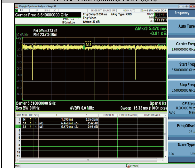
NTNV-11be40MIMO-Ant1-5510
