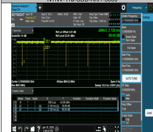
NTNV-11a-CDD-Ant1-5700
