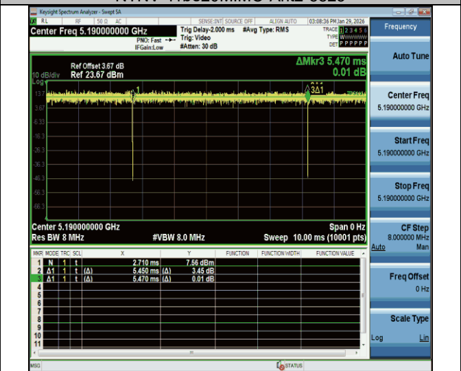
NTNV-11be40MIMO-Ant2-5190
