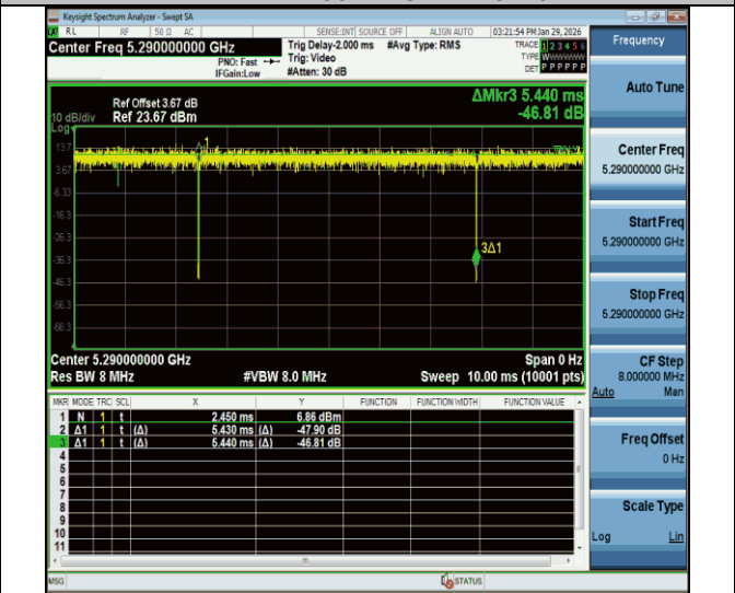
NTNV-11ac80MIMO-Ant2-5290
