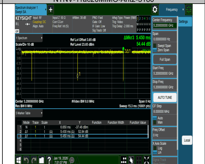
NTNV-11ac20MIMO-Ant2-5200
