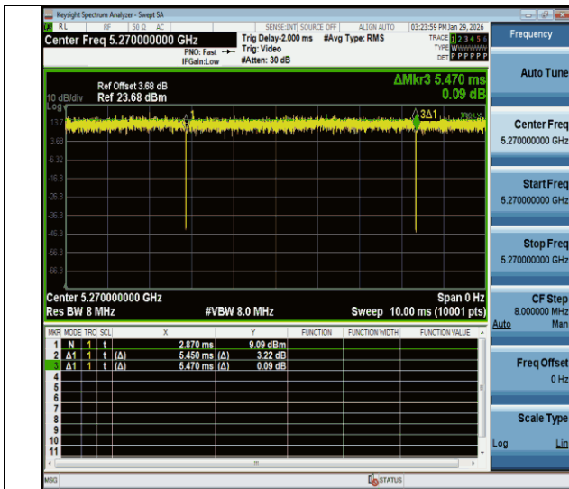
NTNV-11be40MIMO-Ant1-5270
