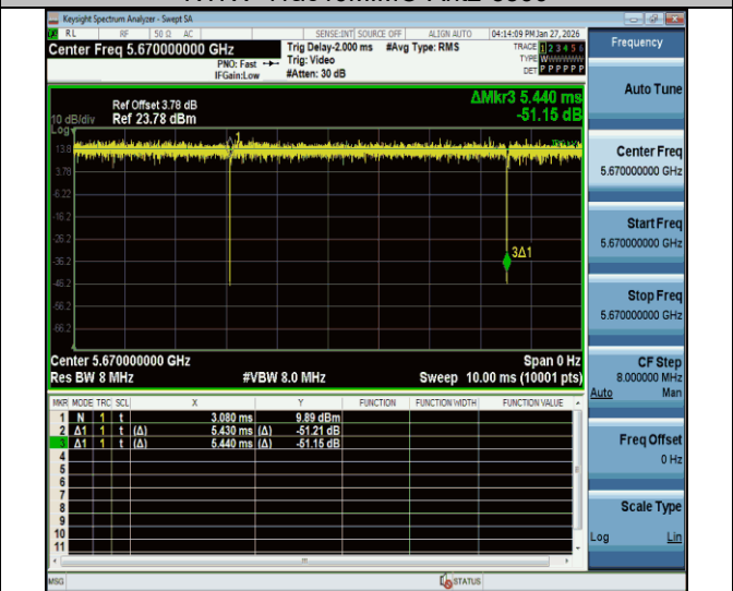
NTNV-11ac40MIMO-Ant2-5670
