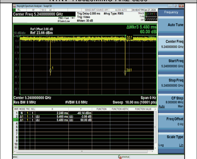
NTNV-11be20MIMO-Ant2-5240
