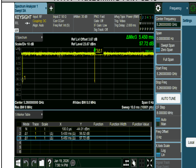
NTNV-11ac20MIMO-Ant1-5260
