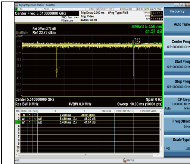
NTNV-11ac40MIMO-Ant1-5510
