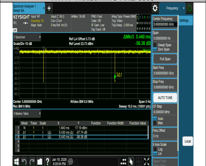
NTVN-11ac20MIMO-Ant2-5600
