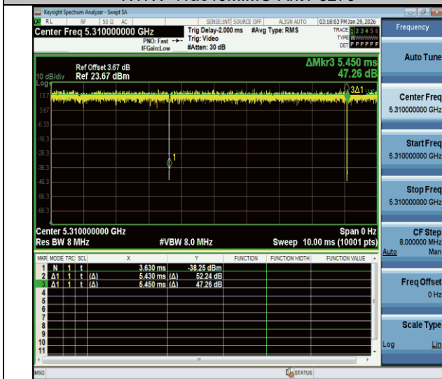
NTNV-11ac40MIMO-Ant1-5310
