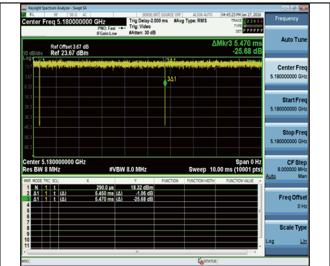
NTNV-11be20MIMO-Ant2-5180
