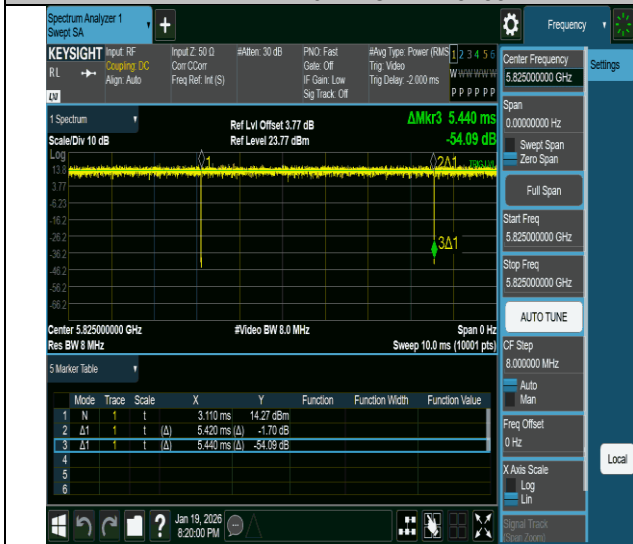
NTVN-11ac20MIMO-Ant1-5825
