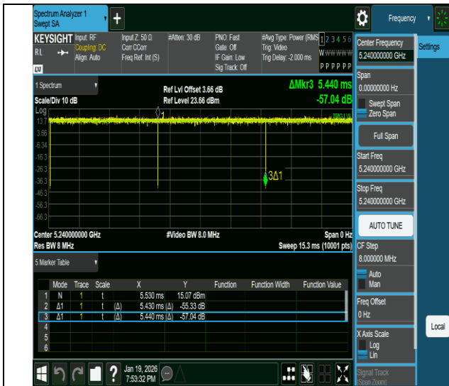
NTNV-11ac20MIMO-Ant1-5240
