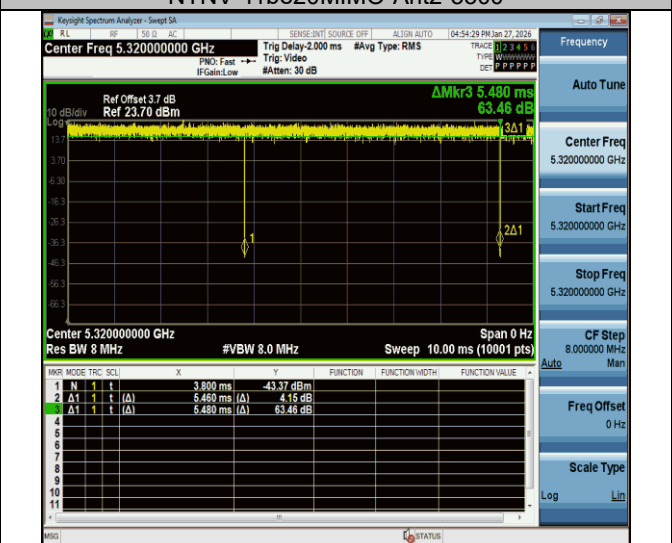
NTNV-11be20MIMO-Ant2-5320
