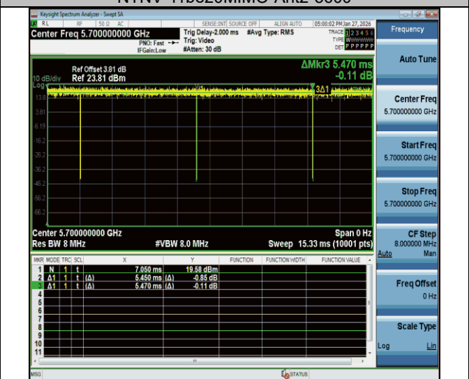
NTNV-11be20MIMO-Ant2-5700
