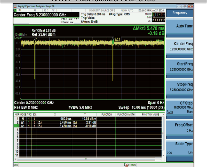
NTNV-11be40MIMO-Ant2-5230
