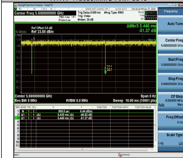
NTNV-11ac80MIMO-Ant1-5690
