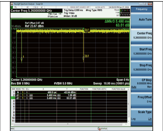
NTNV-11be20MIMO-Ant2-5260
