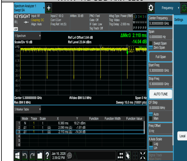
NTNV-11a-CDD-Ant1-5300
