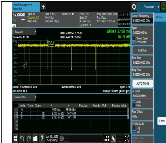
NTNV-11a-CDD-Ant1-5825
