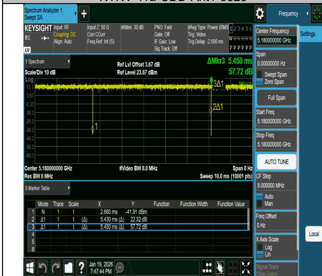
NTNV-11ac20MIMO-Ant1-5180
