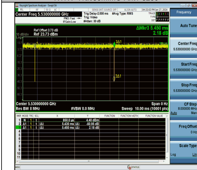
NTNV-11ac80MIMO-Ant1-5530
