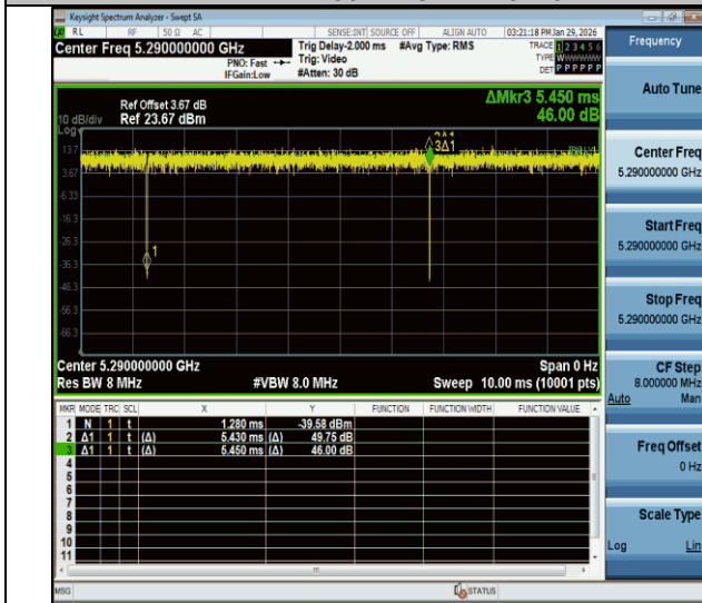
NTNV-11ac80MIMO-Ant1-5290
