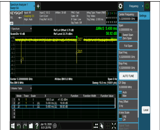
NTVN-11ac20MIMO-Ant2-5320
