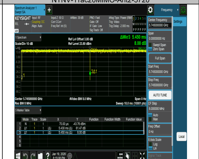
NTNV-11ac20MIMO-Ant2-5745
