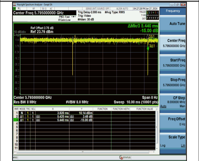
NTNV-11ac40MIMO-Ant2-5795
