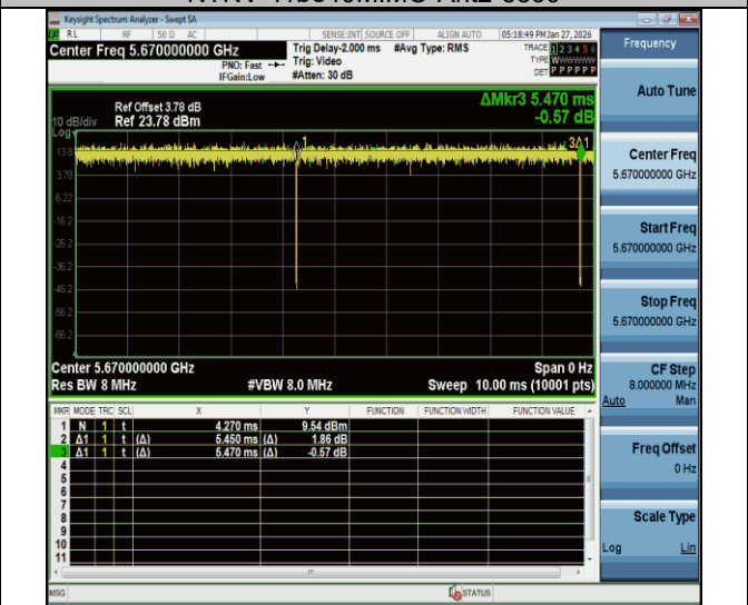
NTNV-11be40MIMO-Ant2-5670
