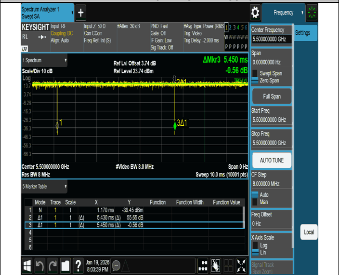
NTVN-11ac20MIMO-Ant2-5500
