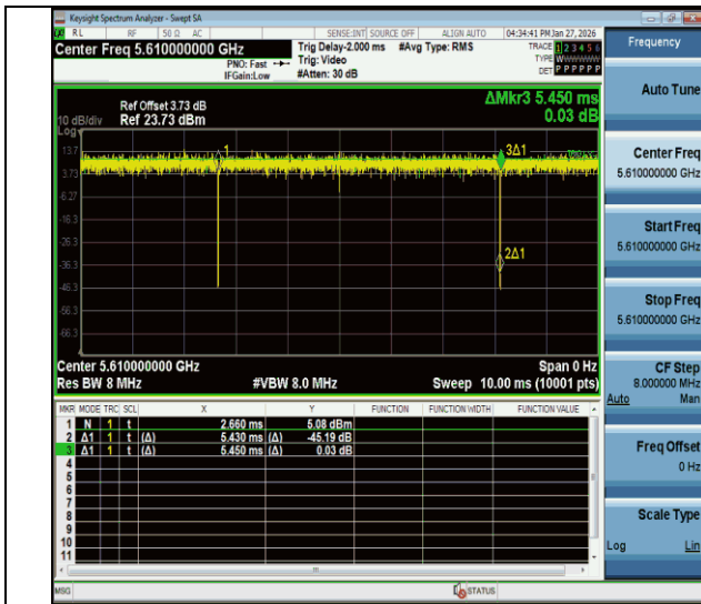
NTNV-11ac80MIMO-Ant1-5610
