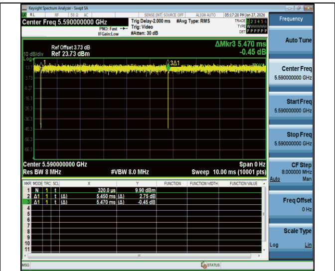
NTNV-11be40MIMO-Ant2-5590
