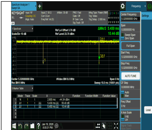
NTVN-11ac20MIMO-Ant1-5320
