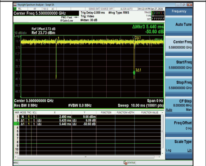
NTNV-11ac40MIMO-Ant2-5590
