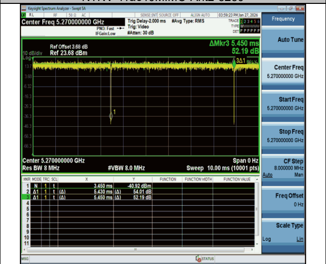
NTNV-11ac40MIMO-Ant2-5270
