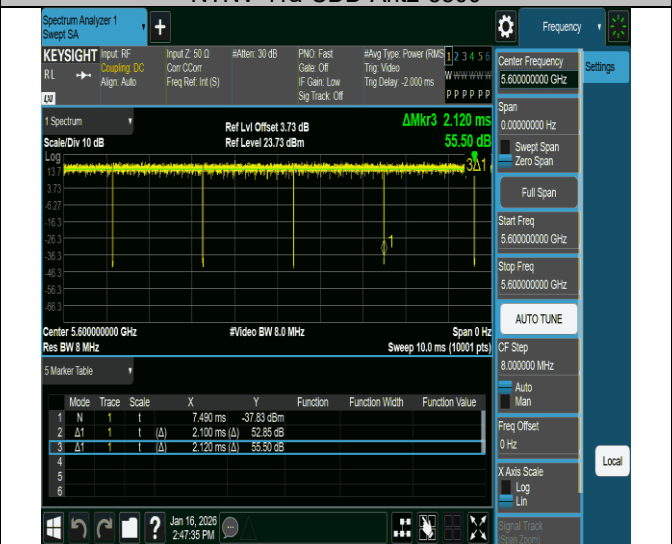
NTNV-11a-CDD-Ant2-5600
