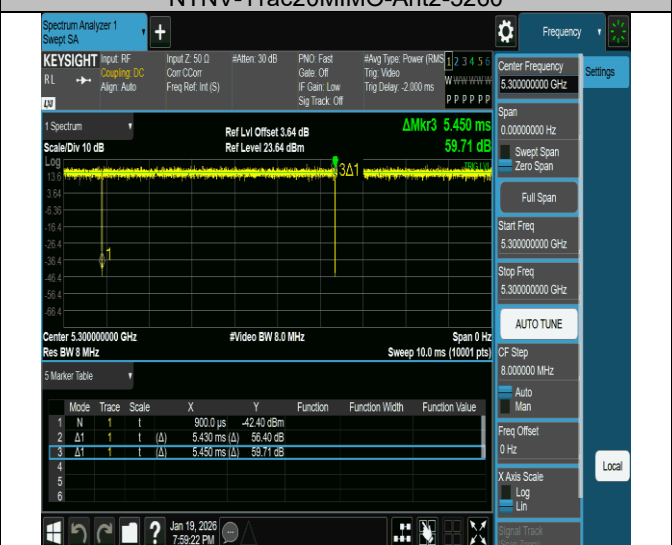
NTNV-11ac20MIMO-Ant2-5300
