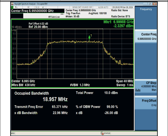
11be20MIMO-Ant2-6995-PASS
