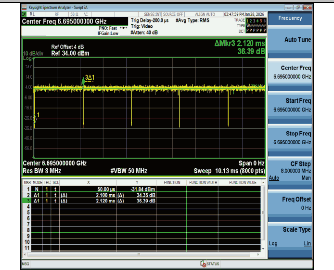
NTNV-11a-CDD-Ant2-6695
