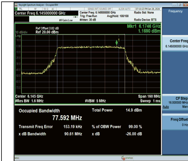
11be80MIMO-Ant1-6145-PASS
