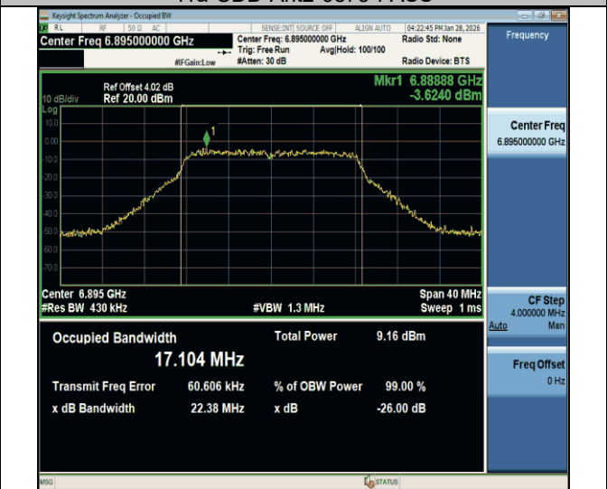
11a-CDD-Ant2-6895-PASS
