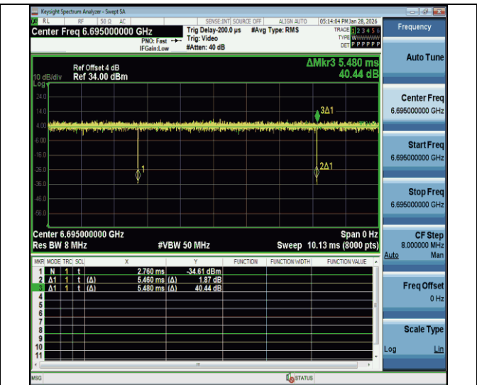
NTNV-11be20MIMO-Ant2-6695
