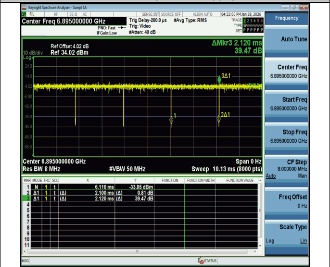
NTNV-11a-CDD-Ant2-6895
