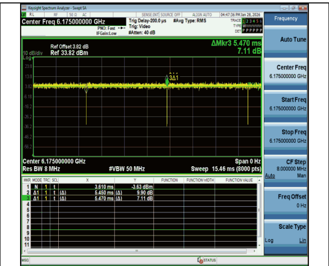
NTNV-11be20MIMO-Ant2-6175
