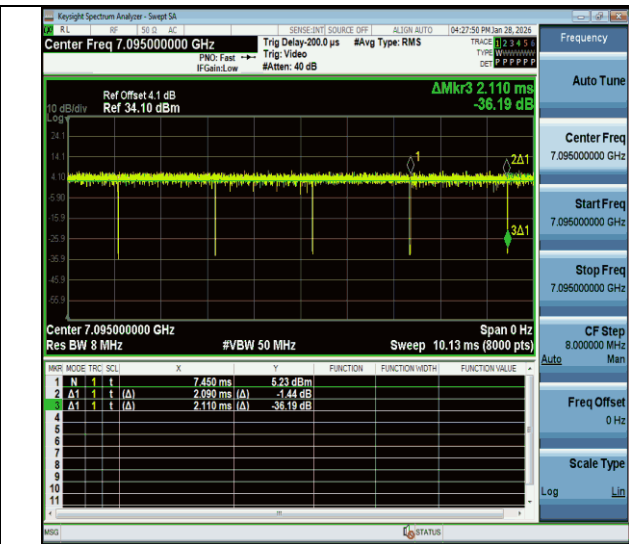
NTNV-11a-CDD-Ant2-7095
