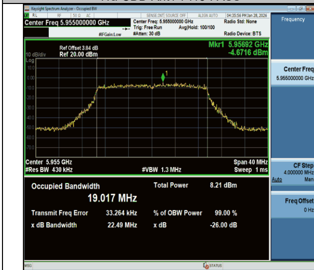
11be20MIMO-Ant1-5955-PASS
