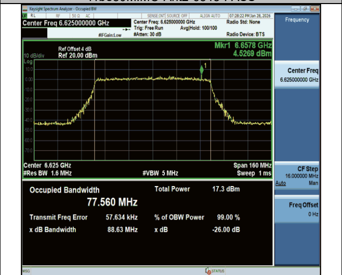
11be80MIMO-Ant2-6625-PASS
