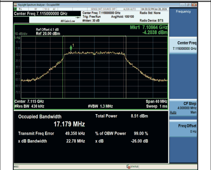
11a-CDD-Ant2-7115-PASS
