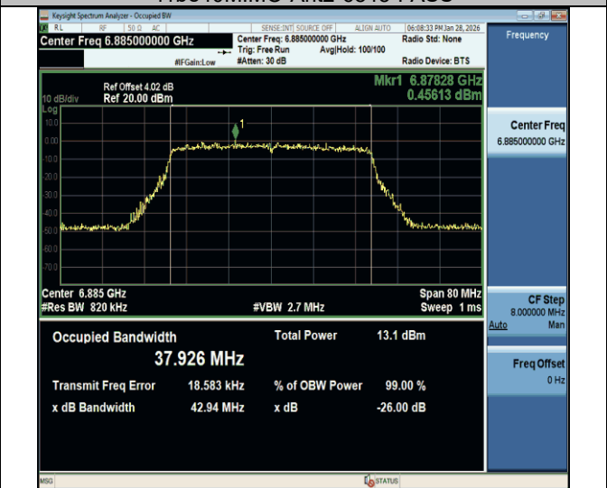
11be40MIMO-Ant2-6885-PASS
