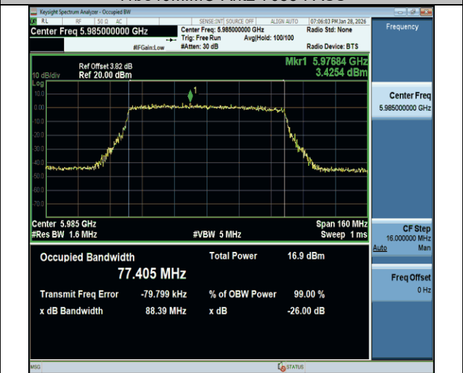
11be80MIMO-Ant2-5985-PASS
