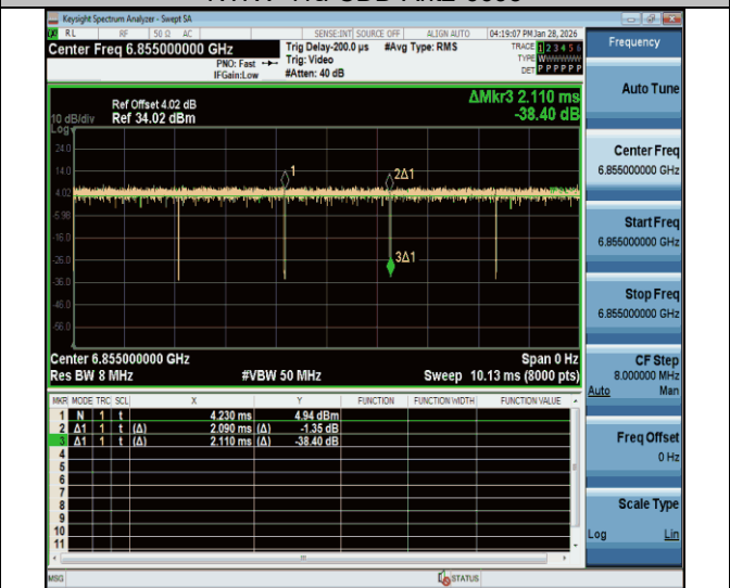
NTNV-11a-CDD-Ant2-6855
