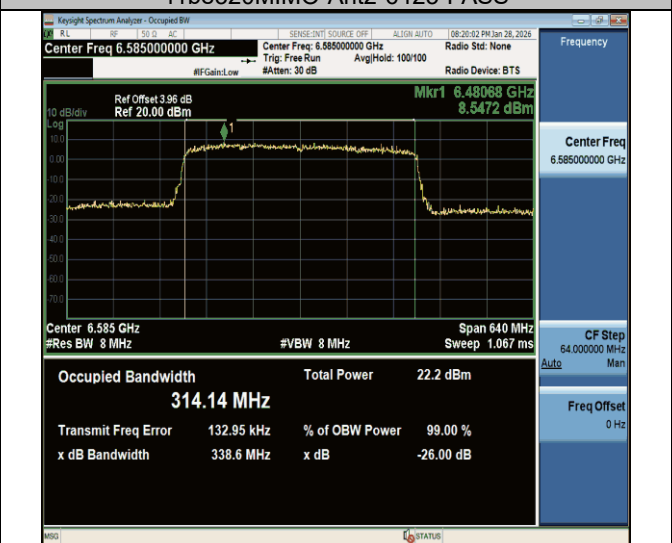
11be320MIMO-Ant2-6585-PASS
