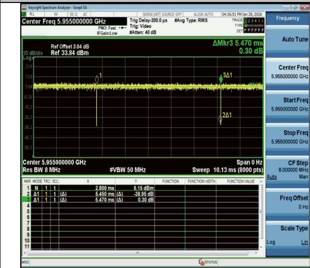
NTNV-11be20MIMO-Ant2-5955
