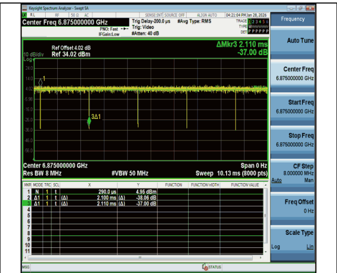
NTNV-11a-CDD-Ant2-6875
