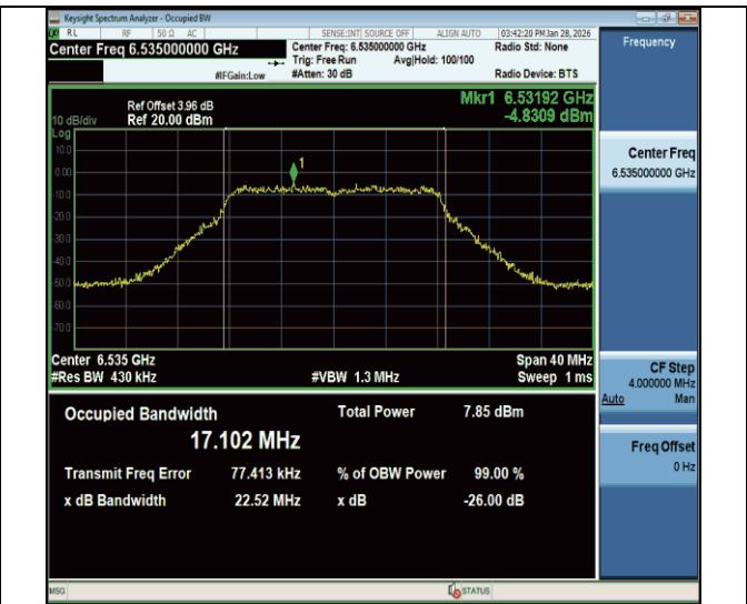
11a-CDD-Ant2-6535-PASS
