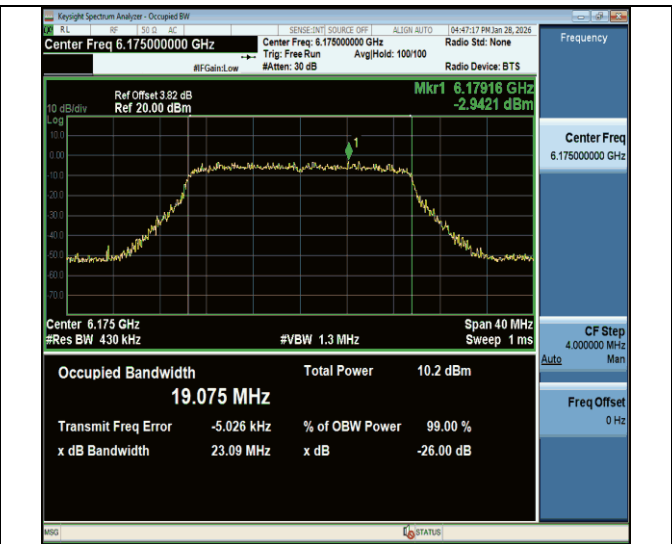
11be20MIMO-Ant2-6175-PASS
