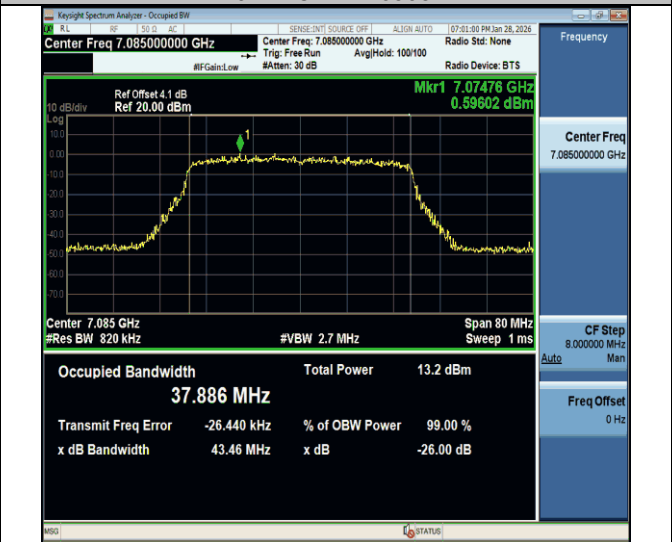
11be40MIMO-Ant2-7085-PASS
