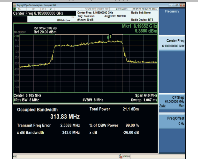
11be320MIMO-Ant2-6105-PASS
