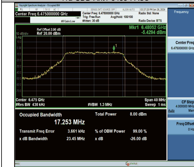
11a-CDD-Ant1-6475-PASS
