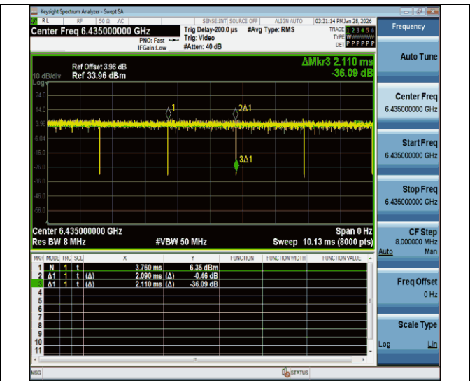
NTVN-11a-CDD-Ant2-6435
