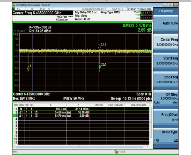
NTNV-11be20MIMO-Ant2-6435
