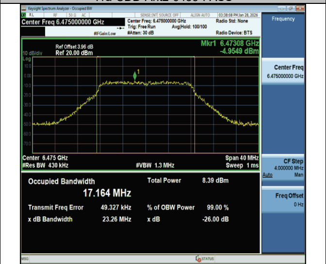
11a-CDD-Ant2-6475-PASS
