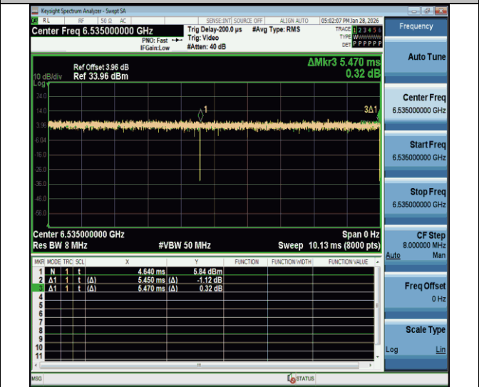
NTNV-11be20MIMO-Ant2-6535
