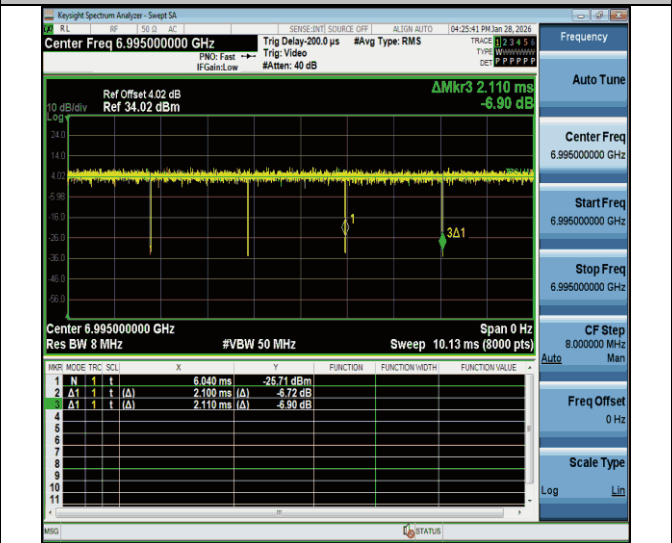
NTNV-11a-CDD-Ant2-6995
