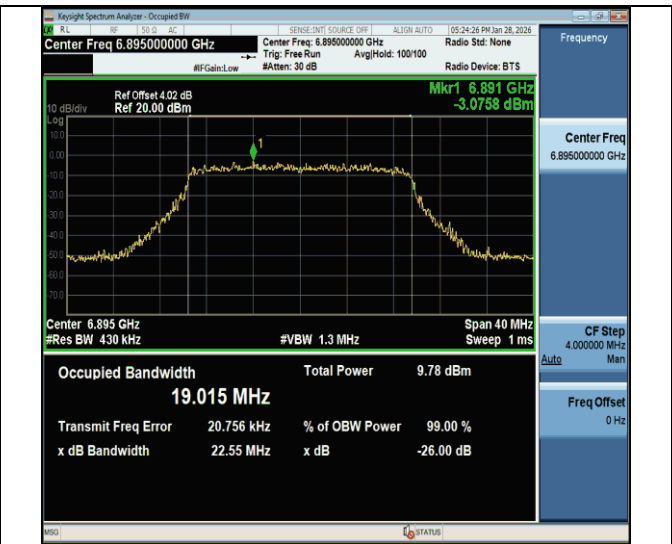
11be20MIMO-Ant2-6895-PASS
