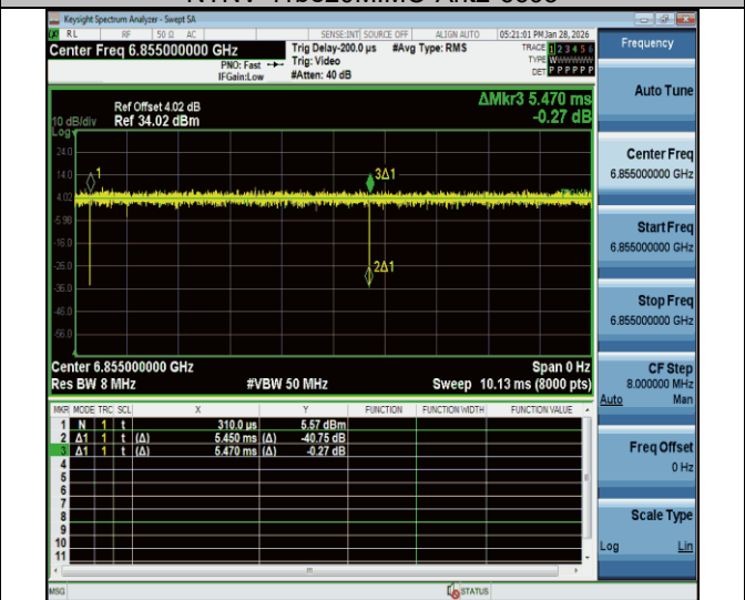
NTNV-11be20MIMO-Ant2-6855
