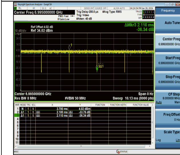
NTNV-11a-CDD-Ant1-6995
