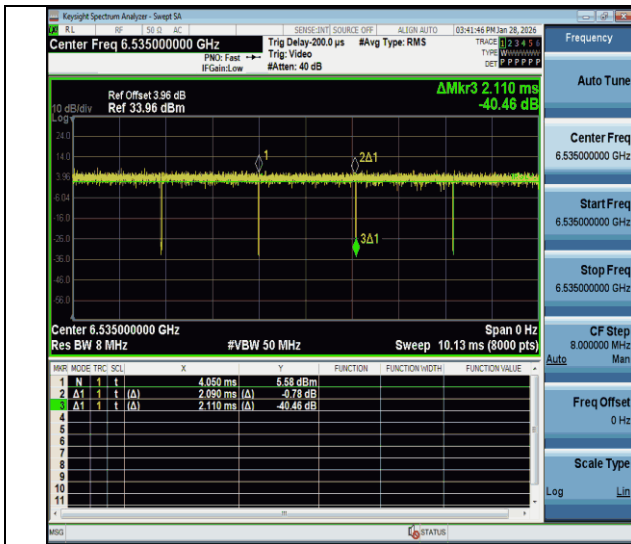
NTNV-11a-CDD-Ant1-6535
