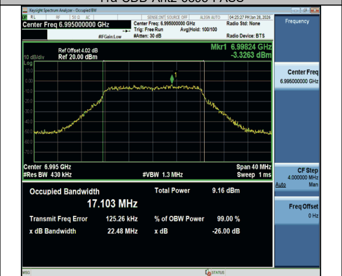
11a-CDD-Ant2-6995-PASS
