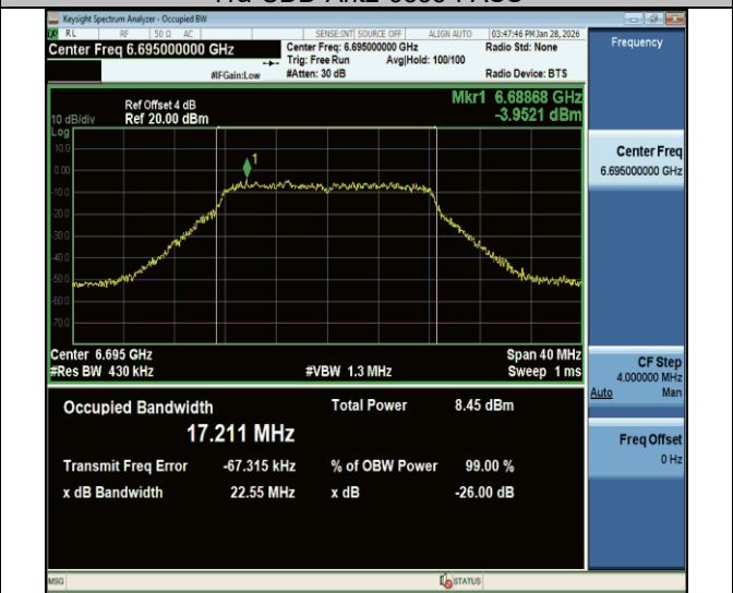
11a-CDD-Ant2-6695-PASS
