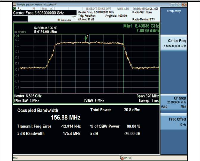
11be160MIMO-Ant2-6505-PASS
