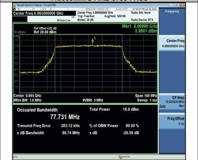
11be80MIMO-Ant2-6865-PASS
