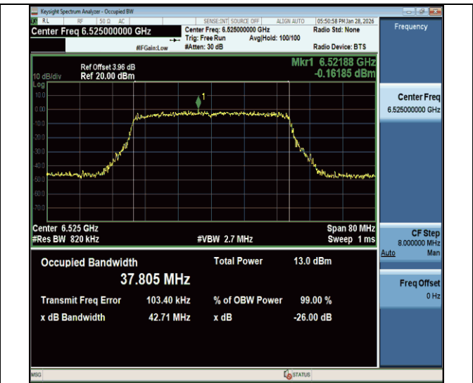
11be40MIMO-Ant2-6525-PASS
