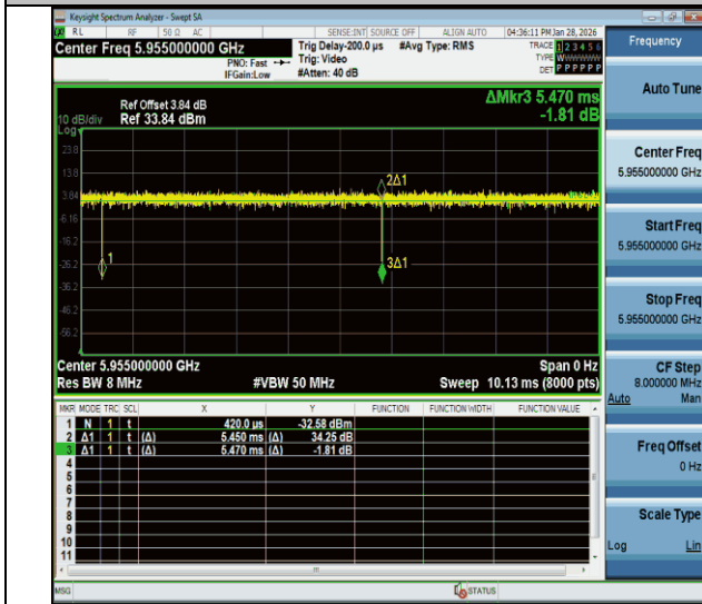
NTNV-11be20MIMO-Ant1-5955
