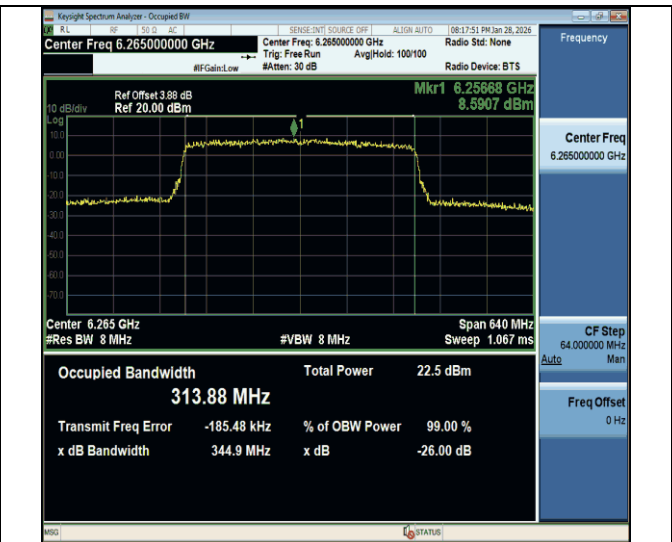
11be320MIMO-Ant2-6265-PASS
