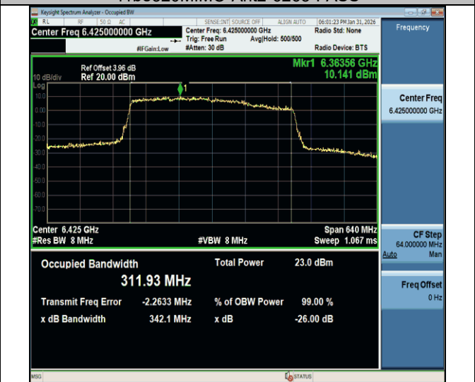
11be320MIMO-Ant2-6425-PASS
