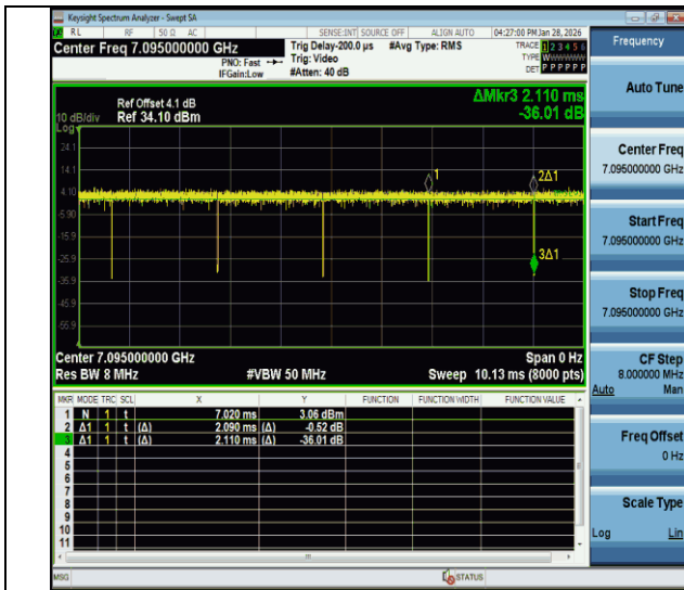
NTNV-11a-CDD-Ant1-7095
