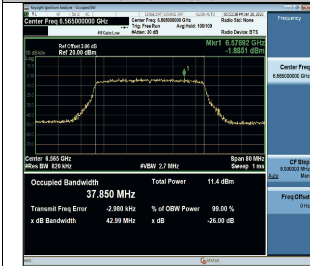
11be40MIMO-Ant1-6565-PASS
