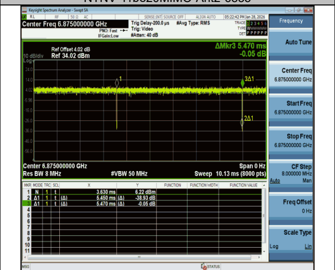
NTNV-11be20MIMO-Ant2-6875
