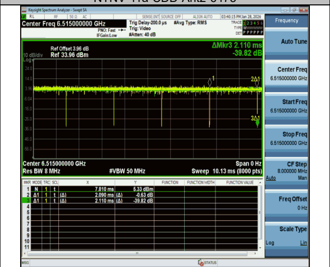
NTVN-11a-CDD-Ant2-6515
