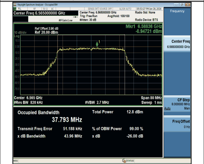
11be40MIMO-Ant2-6565-PASS
