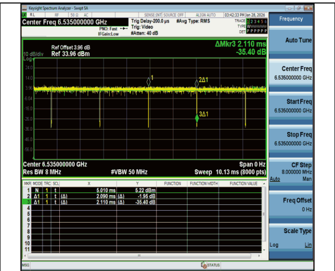
NTNV-11a-CDD-Ant2-6535
