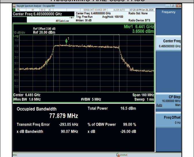
11be80MIMO-Ant2-6465-PASS
