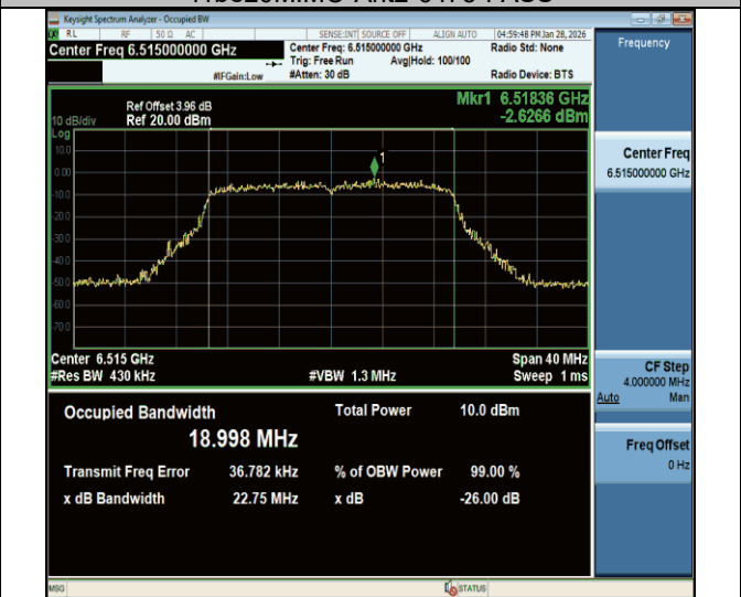
11be20MIMO-Ant2-6515-PASS
