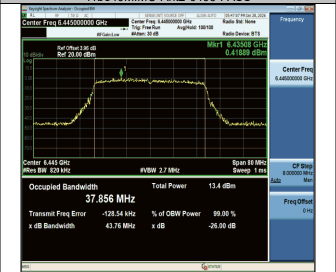
11be40MIMO-Ant2-6445-PASS
