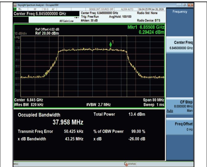
11be40MIMO-Ant2-6845-PASS
