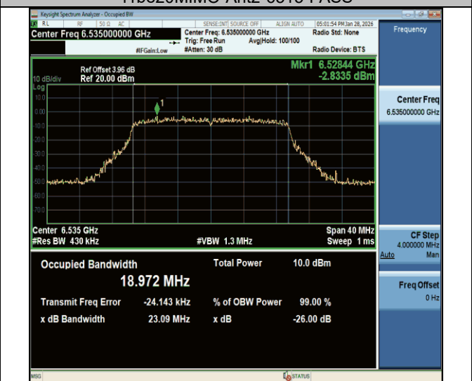
11be20MIMO-Ant2-6535-PASS
