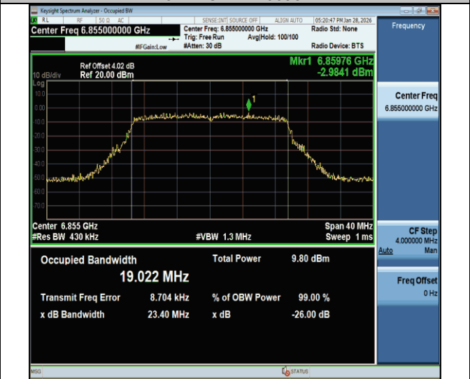
11be20MIMO-Ant2-6855-PASS
