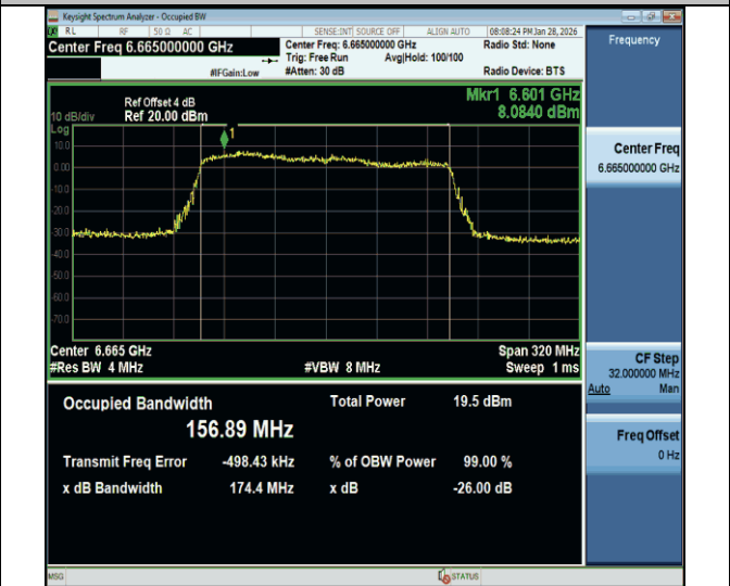
11be160MIMO-Ant2-6665-PASS
