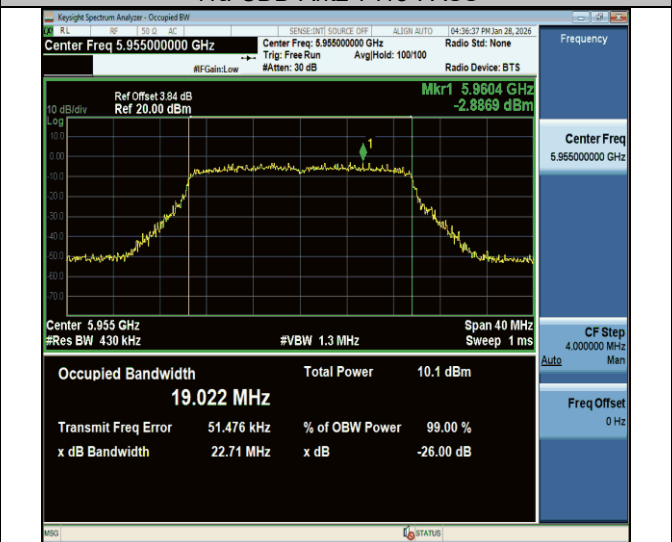
11be20MIMO-Ant2-5955-PASS
