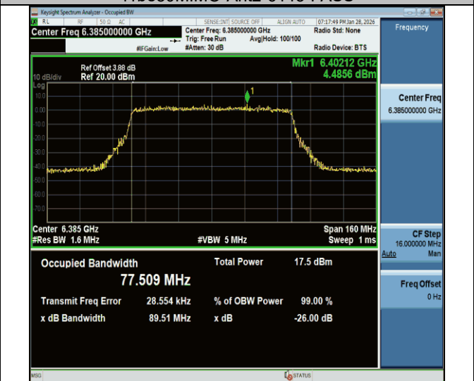
11be80MIMO-Ant2-6385-PASS
