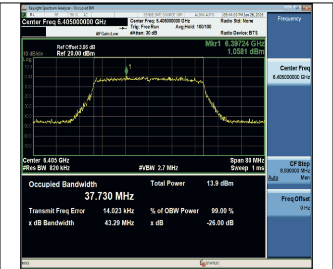
11be40MIMO-Ant2-6405-PASS
