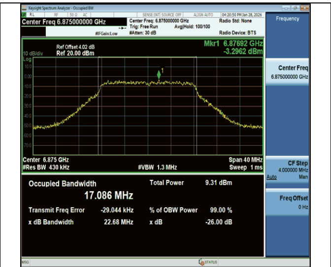
11a-CDD-Ant2-6875-PASS
