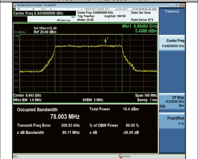
11be80MIMO-Ant2-6945-PASS
