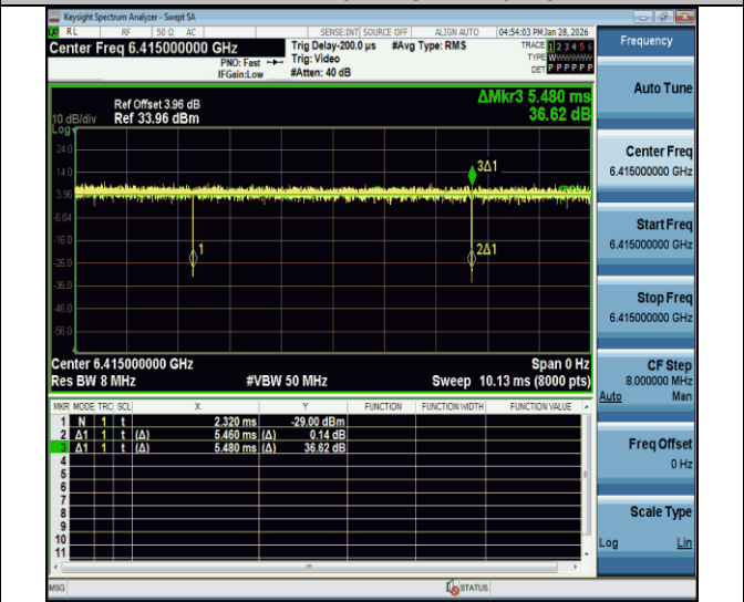
NTNV-11be20MIMO-Ant2-6415
