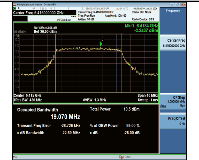
11be20MIMO-Ant2-6415-PASS
