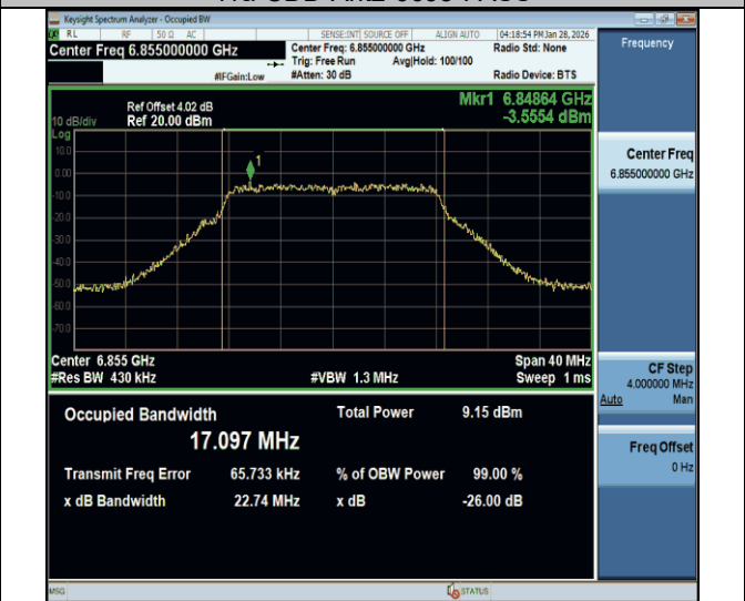
11a-CDD-Ant2-6855-PASS
