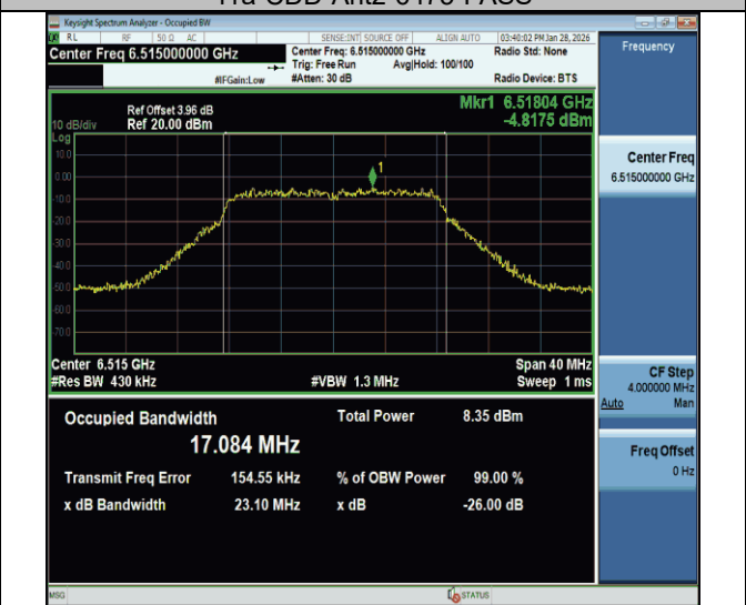
11a-CDD-Ant2-6515-PASS
