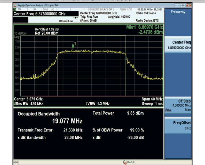
11be20MIMO-Ant2-6875-PASS
