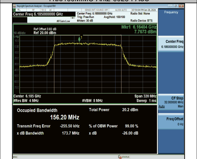
11be160MIMO-Ant2-6185-PASS
