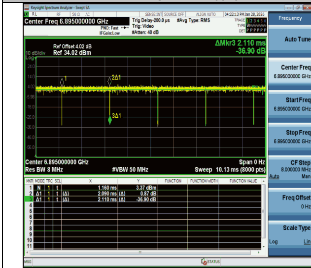
NTNV-11a-CDD-Ant1-6895
