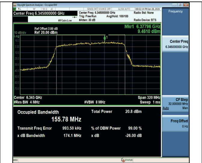
11be160MIMO-Ant2-6345-PASS
