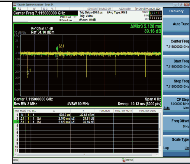
NTNV-11a-CDD-Ant2-7115
