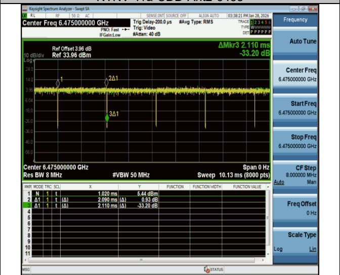
NTVN-11a-CDD-Ant2-6475
