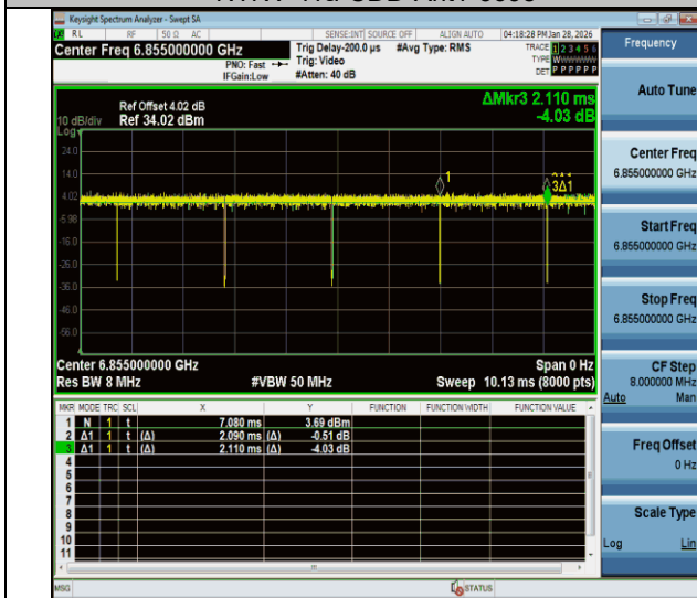
NTNV-11a-CDD-Ant1-6855
