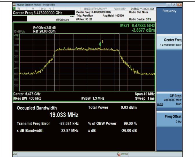
11be20MIMO-Ant2-6475-PASS
