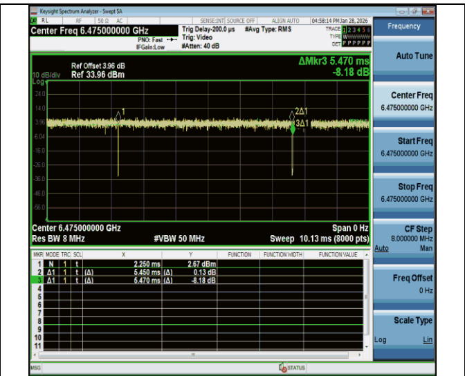
NTNV-11be20MIMO-Ant2-6475
