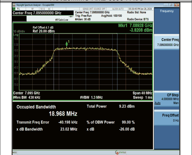
11be20MIMO-Ant2-7095-PASS
