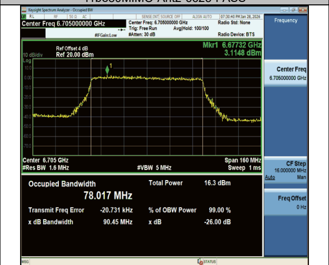
11be80MIMO-Ant2-6705-PASS
