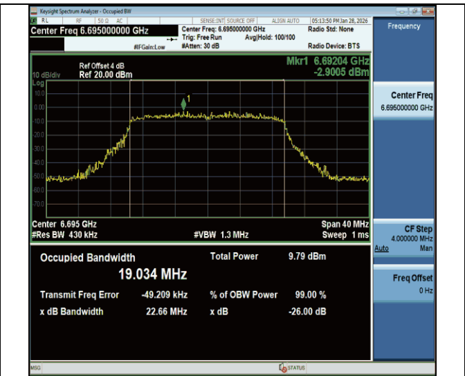
11be20MIMO-Ant2-6695-PASS
