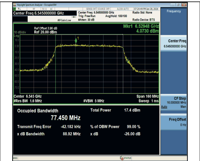
11be80MIMO-Ant2-6545-PASS
