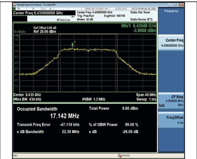
11a-CDD-Ant2-6435-PASS
