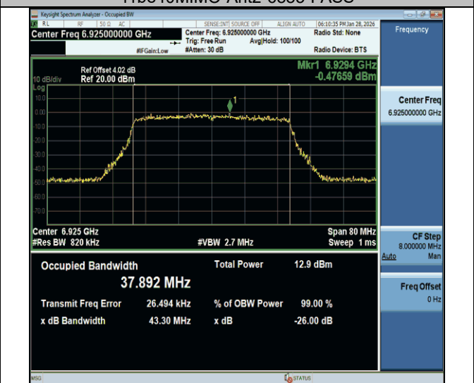
11be40MIMO-Ant2-6925-PASS
