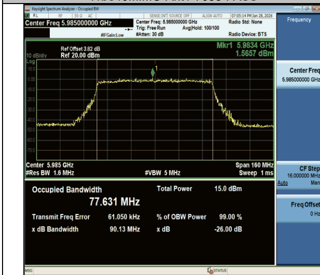
11be80MIMO-Ant1-5985-PASS
