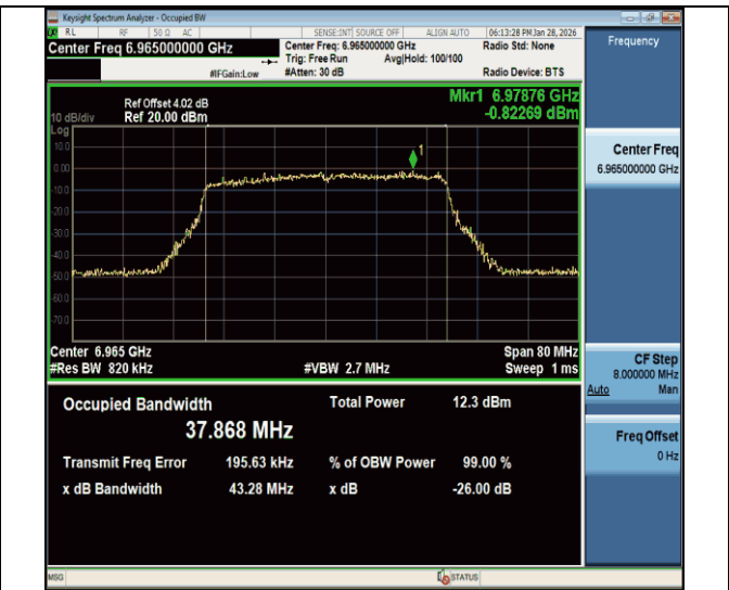
11be40MIMO-Ant2-6965-PASS
