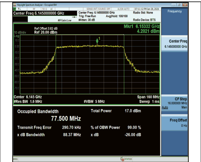
11be80MIMO-Ant2-6145-PASS
