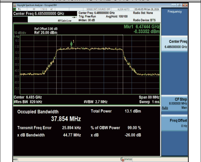
11be40MIMO-Ant2-6485-PASS
