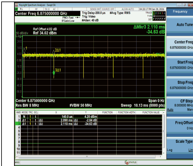
NTNV-11a-CDD-Ant1-6875
