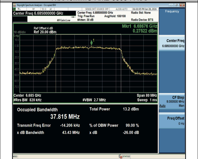
11be40MIMO-Ant2-6685-PASS
