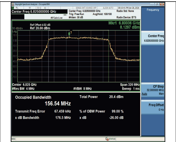
11be160MIMO-Ant2-6825-PASS
