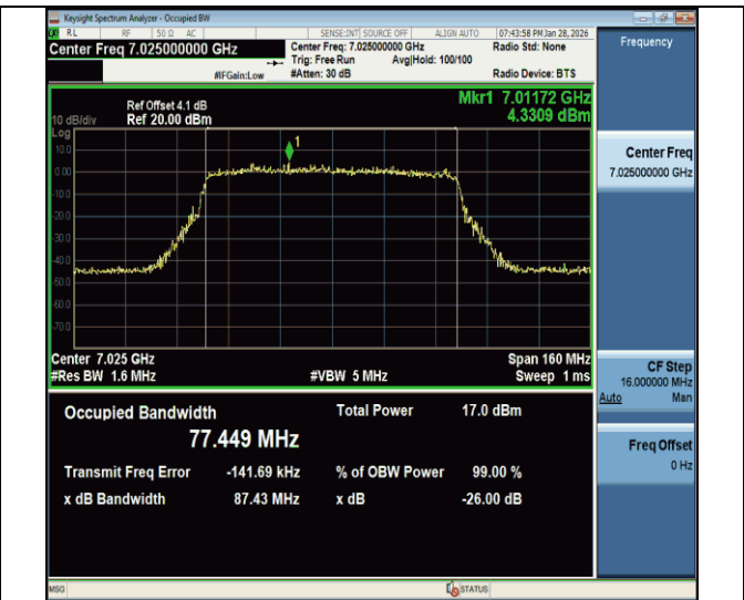
11be80MIMO-Ant2-7025-PASS
