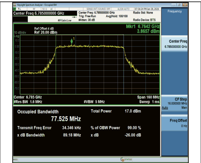
11be80MIMO-Ant2-6785-PASS
