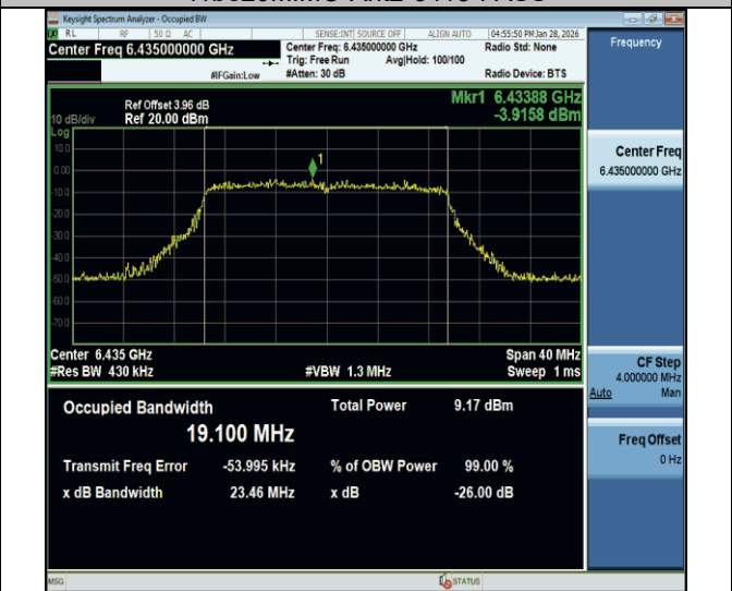
11be20MIMO-Ant2-6435-PASS
