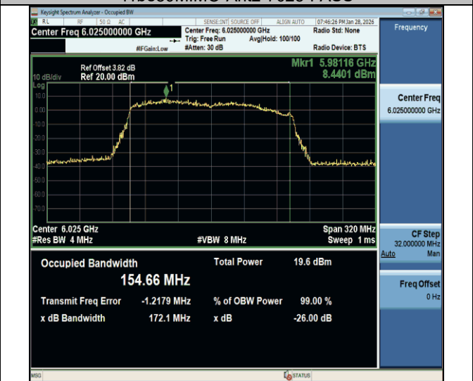
11be160MIMO-Ant2-6025-PASS
