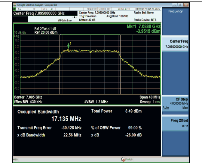
11a-CDD-Ant2-7095-PASS
