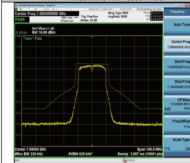
NTVN-11be20MIMO-Ant1-7095-PASS
