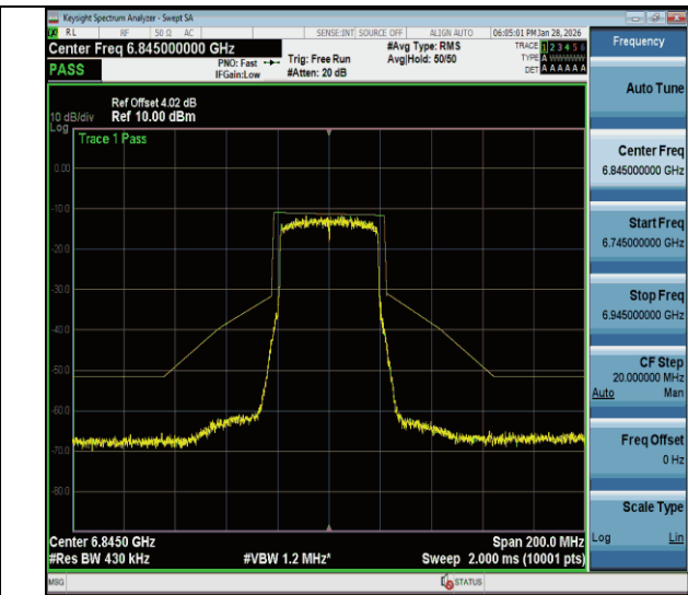
NTVN-11be40MIMO-Ant2-6845-PASS
