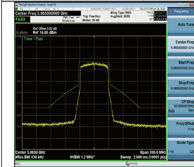
NTVN-11be40MIMO-Ant1-5965-PASS
