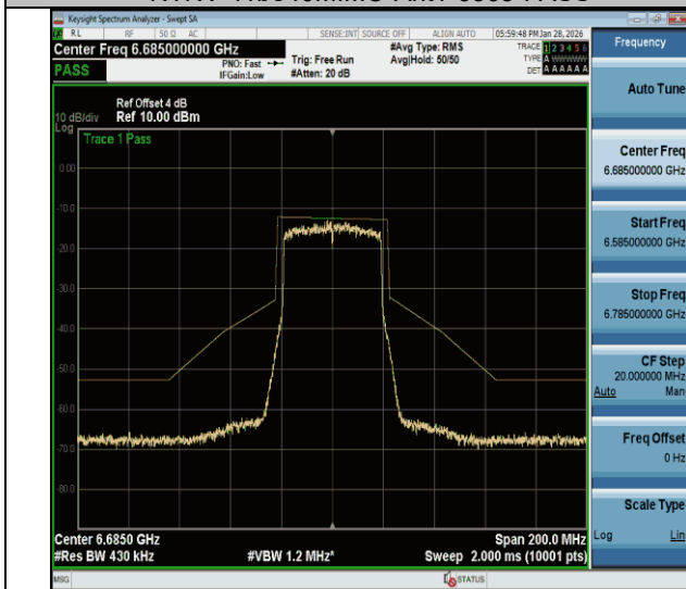
NTVN-11be40MIMO-Ant1-6685-PASS
