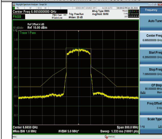
NTNV-11be160MIMO-Ant1-6665-PASS
