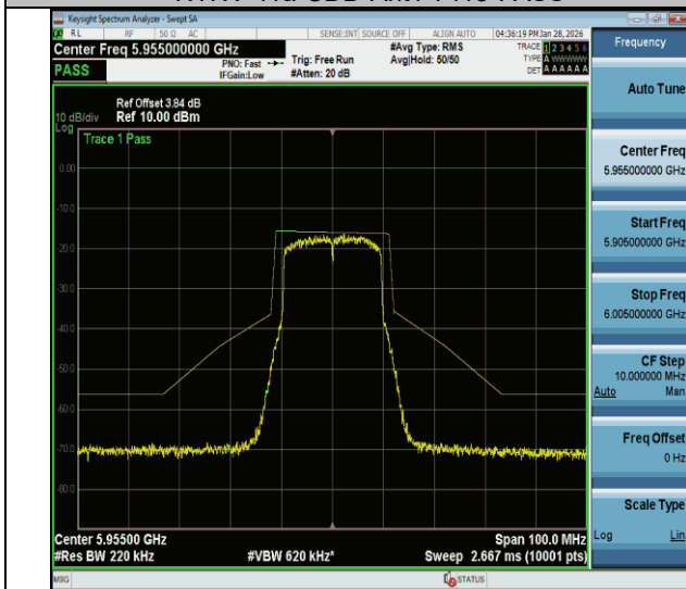
NTVN-11be20MIMO-Ant1-5955-PASS
