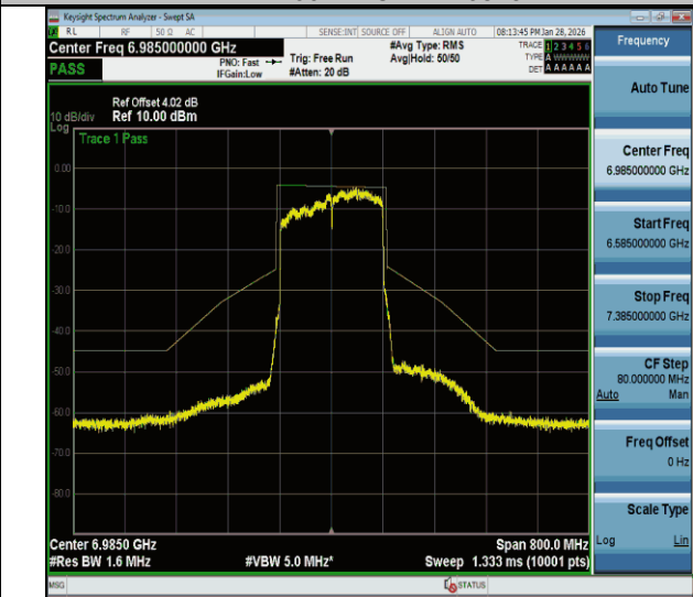
NTNV-11be160MIMO-Ant2-6985-PASS
