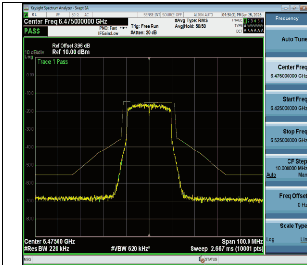
NTVN-11be20MIMO-Ant2-6475-PASS
