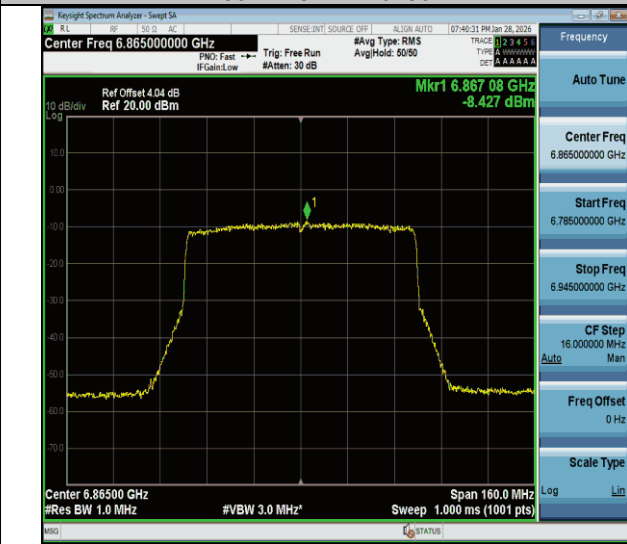
11be80MIMO-Ant2-6865-PASS
