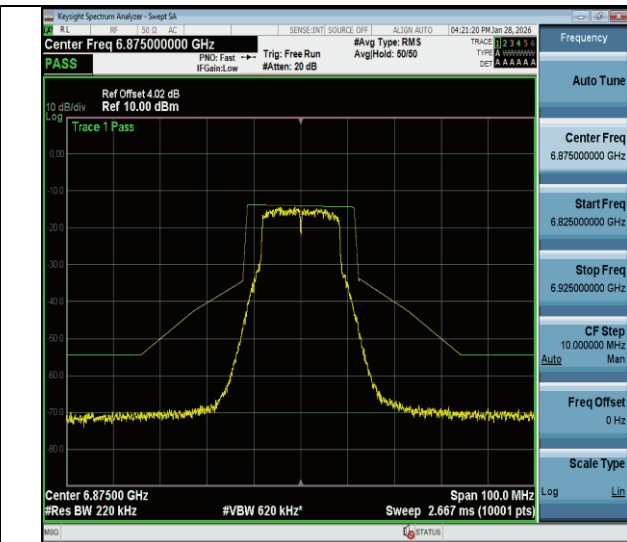
NTVN-11a-CDD-Ant2-6875-PASS
