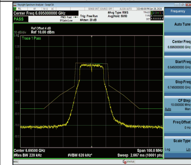
NTVN-11a-CDD-Ant2-6695-PASS
