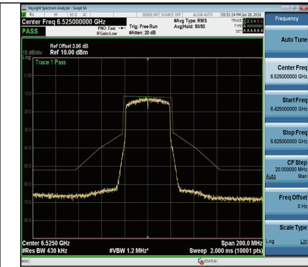
NTVN-11be40MIMO-Ant2-6525-PASS
