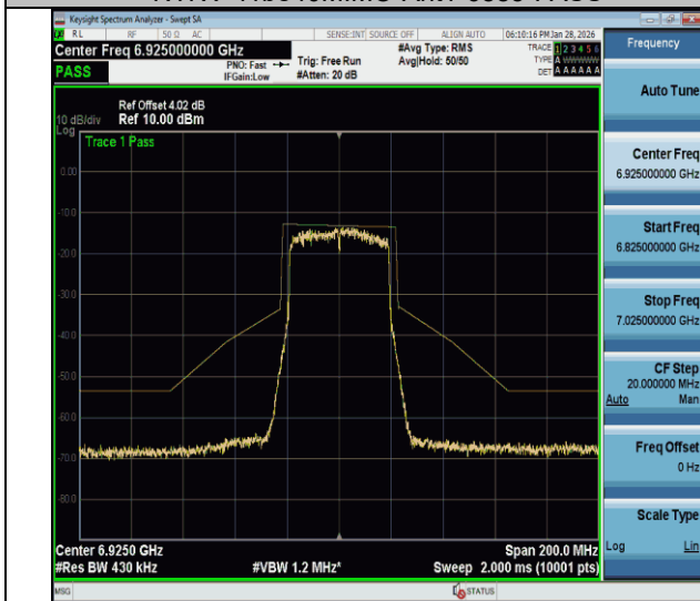
NTVN-11be40MIMO-Ant1-6925-PASS
