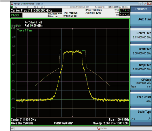
NTVN-11a-CDD-Ant2-7115-PASS
