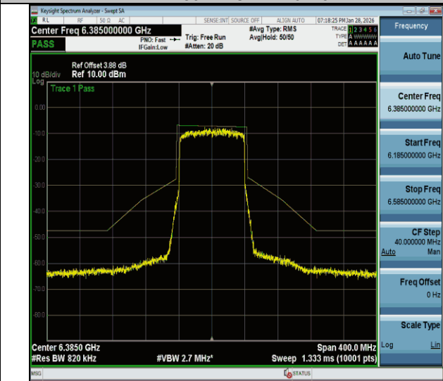
NTVN-11be80MIMO-Ant2-6385-PASS
