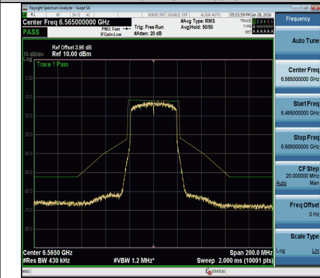
NTVN-11be40MIMO-Ant2-6565-PASS
