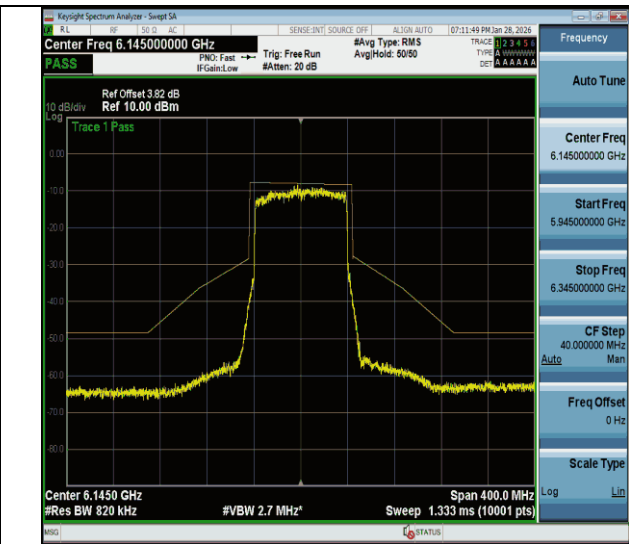
NTVN-11be80MIMO-Ant2-6145-PASS
