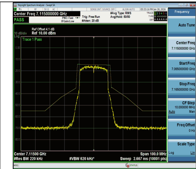
NTVN-11be20MIMO-Ant2-7115-PASS
