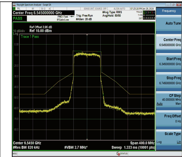
NTVN-11be80MIMO-Ant2-6545-PASS
