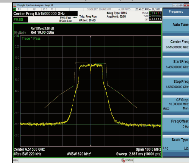
NTVN-11a-CDD-Ant2-6515-PASS
