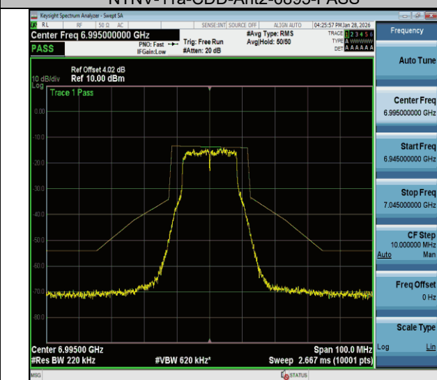
NTVN-11a-CDD-Ant2-6995-PASS
