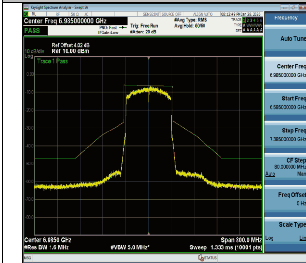
NTNV-11be160MIMO-Ant1-6985-PASS
