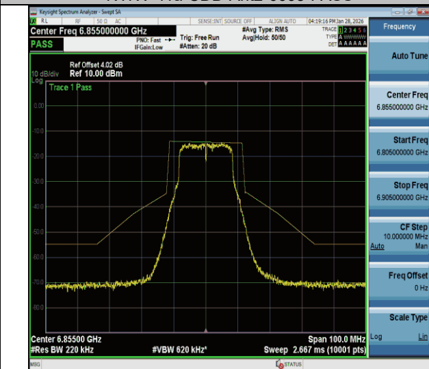
NTVN-11a-CDD-Ant2-6855-PASS
