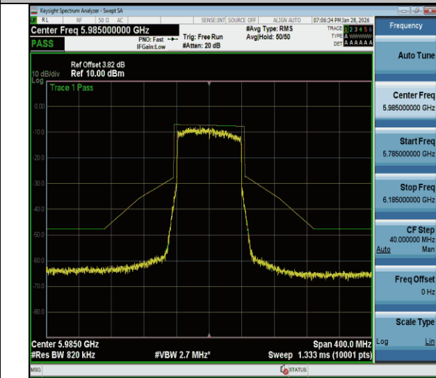
NTVN-11be80MIMO-Ant2-5985-PASS
