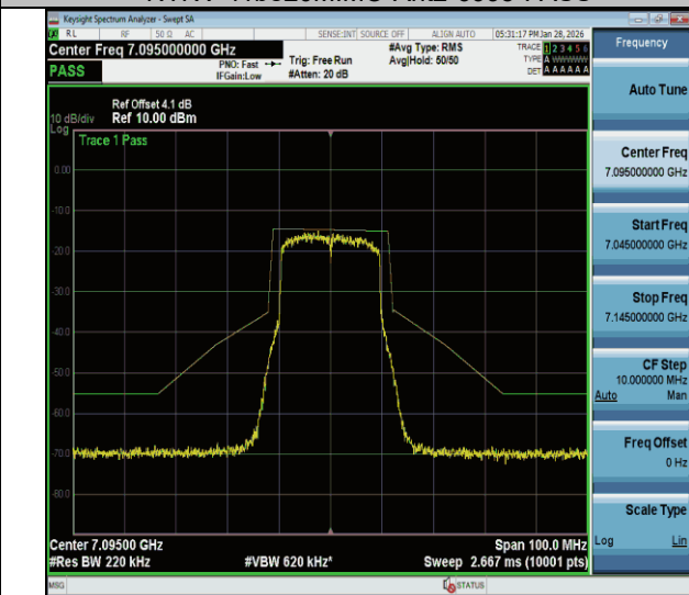
NTVN-11be20MIMO-Ant2-7095-PASS
