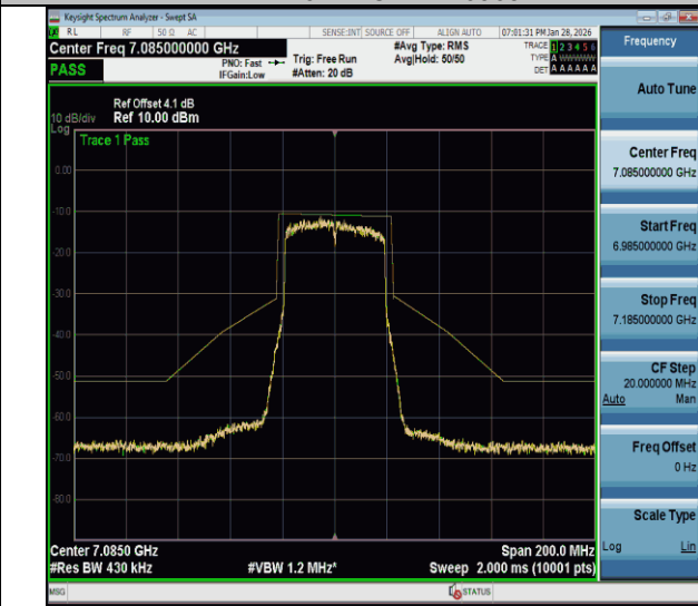
NTVN-11be40MIMO-Ant2-7085-PASS
