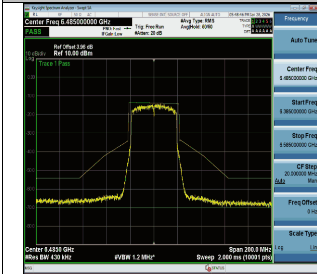
NTVN-11be40MIMO-Ant1-6485-PASS
