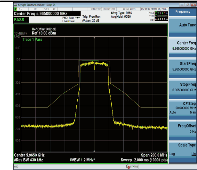
NTVN-11be40MIMO-Ant2-5965-PASS
