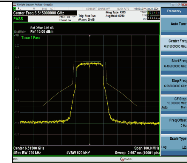
NTVN-11be20MIMO-Ant2-6515-PASS
