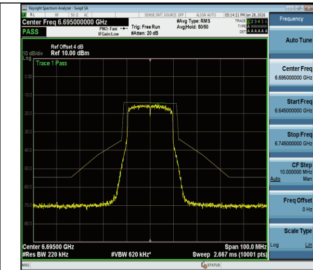
NTVN-11be20MIMO-Ant2-6695-PASS
