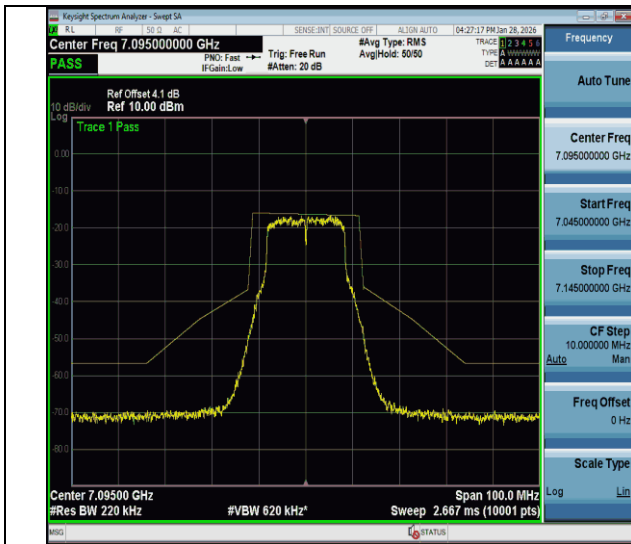
NTVN-11a-CDD-Ant1-7095-PASS
