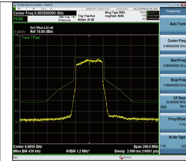
NTVN-11be40MIMO-Ant2-6965-PASS
