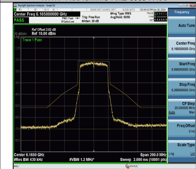
NTVN-11be40MIMO-Ant2-6165-PASS
