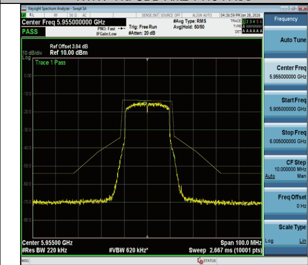
NTVN-11be20MIMO-Ant2-5955-PASS
