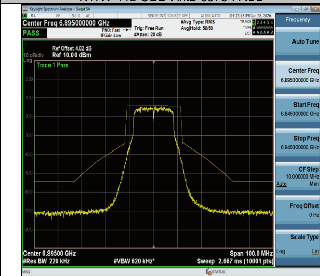
NTVN-11a-CDD-Ant2-6895-PASS
