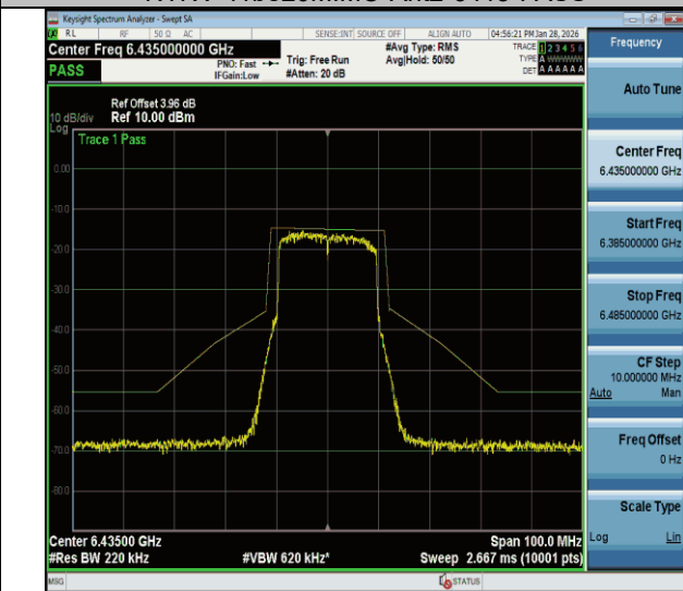
NTVN-11be20MIMO-Ant2-6435-PASS
