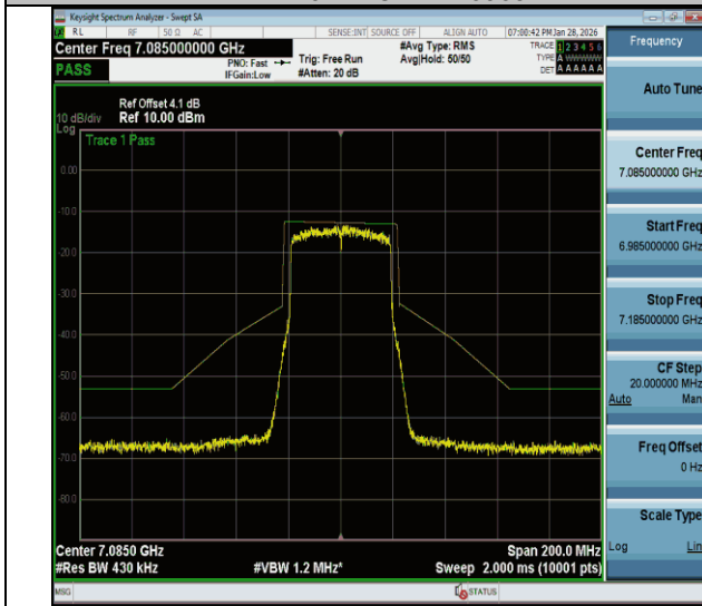
NTVN-11be40MIMO-Ant1-7085-PASS
