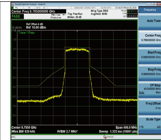
NTVN-11be80MIMO-Ant2-6785-PASS
