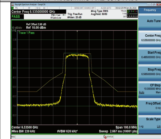
NTVN-11be20MIMO-Ant2-6535-PASS
