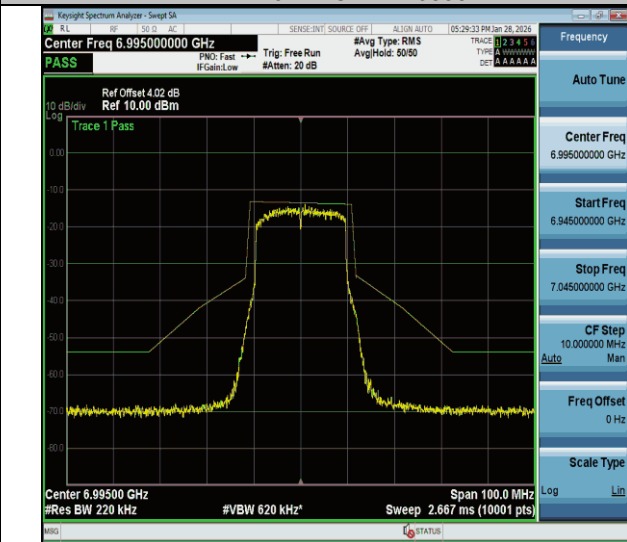
NTVN-11be20MIMO-Ant2-6995-PASS
