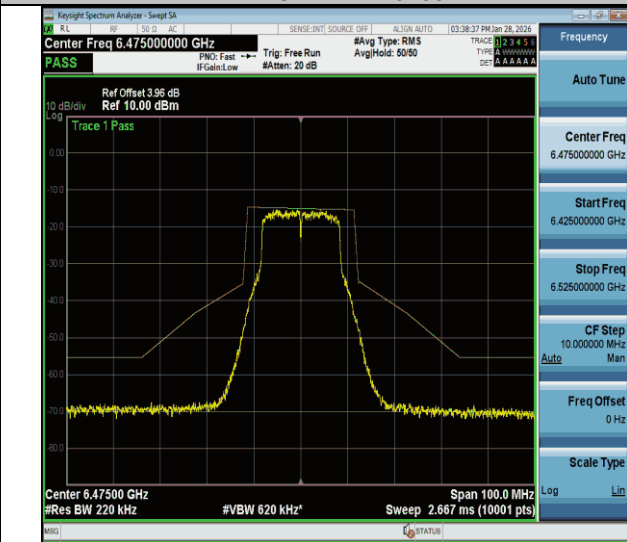
NTVN-11a-CDD-Ant2-6475-PASS
