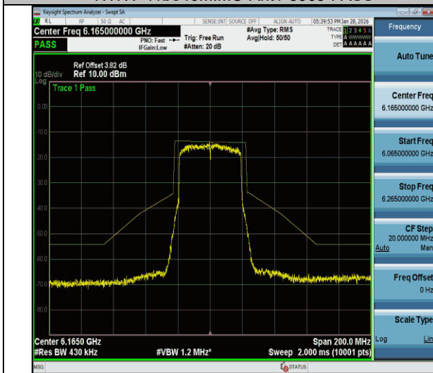
NTVN-11be40MIMO-Ant1-6165-PASS
