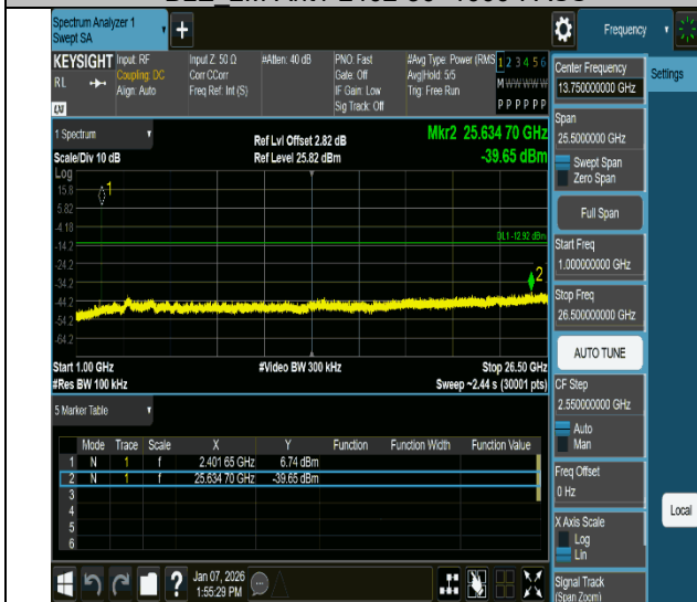
BLE_2M-Ant1-2402-1000~26500-PASS
