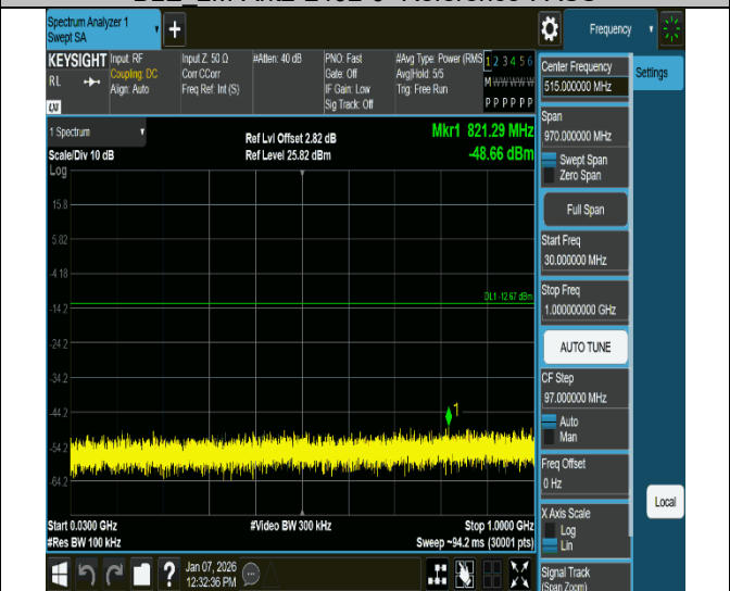
BLE_2M-Ant2-2402-30~1000-PASS
