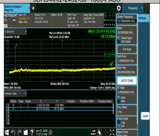
3DH5-Ant2-2402-1000~26500-PASS
