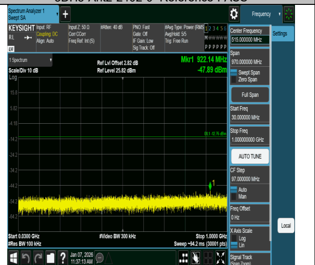
3DH5-Ant2-2402-30~1000-PASS
