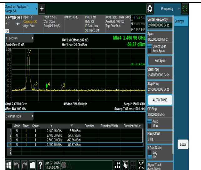
3DH5-Ant2-2480-PASS
