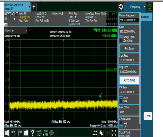
DH5-Ant2-2480-30~1000-PASS
