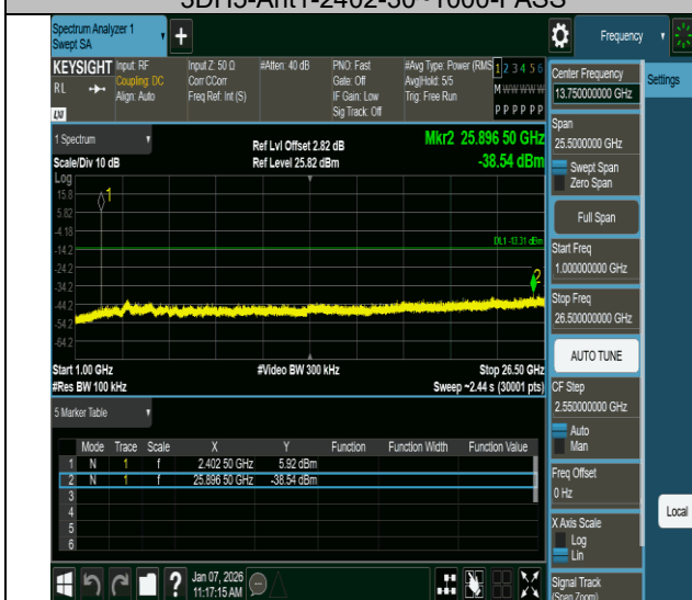
3DH5-Ant1-2402-1000~26500-PASS
