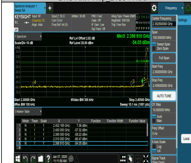
2DH5-Ant1-2402-PASS
