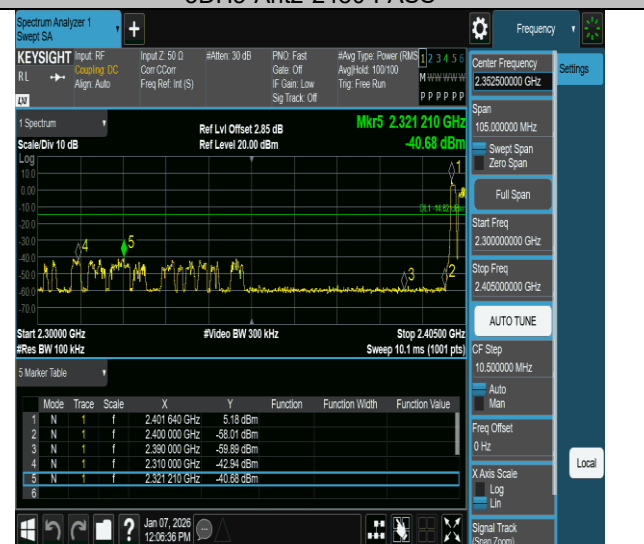
3DH5-Ant2-Hop 2402-PASS
