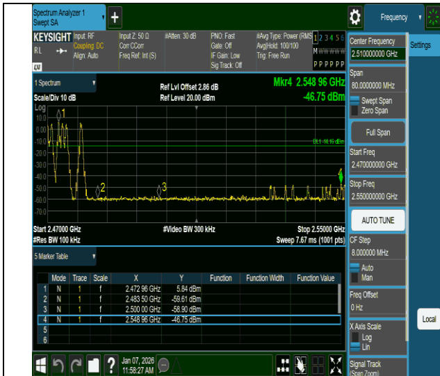
DH5-Ant1-Hop 2480-PASS
