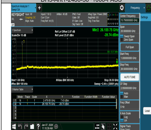
DH5-Ant1-2480-1000~26500-PASS
