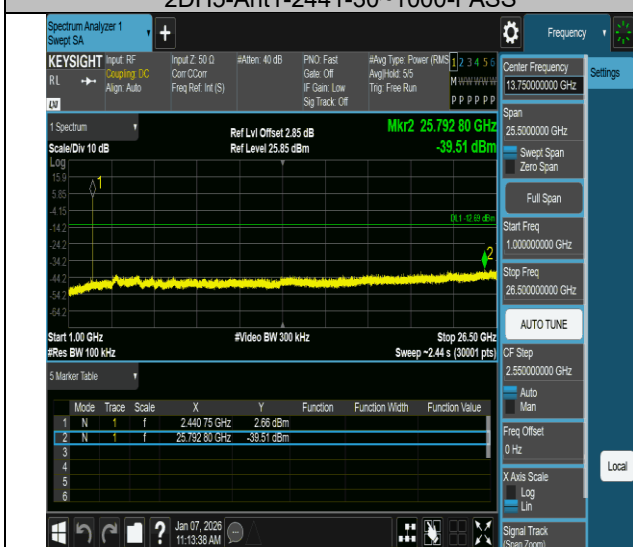
2DH5-Ant1-2441-1000~26500-PASS
