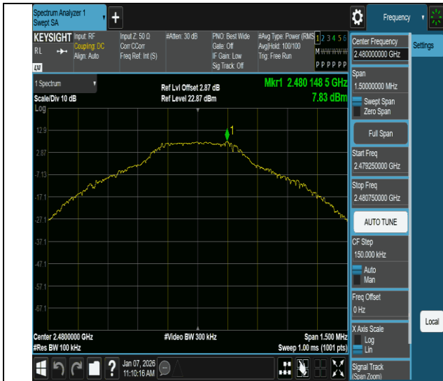
DH5-Ant1-2480-0~Reference-PASS
