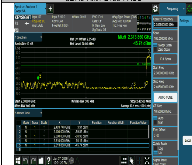
3DH5-Ant1-Hop 2402-PASS
