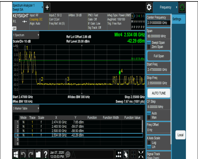
DH5-Ant2-Hop 2480-PASS
