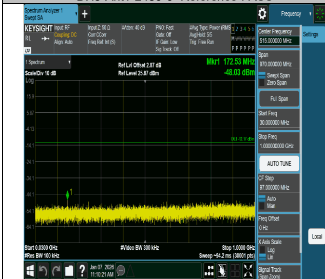
DH5-Ant1-2480-30~1000-PASS
