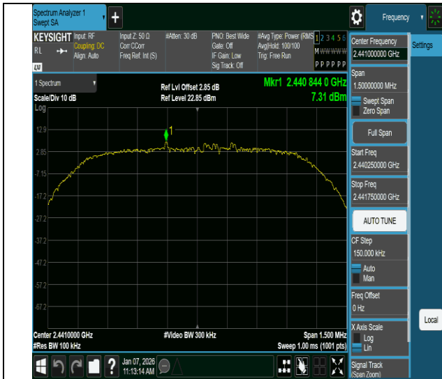
2DH5-Ant1-2441-0~Reference-PASS
