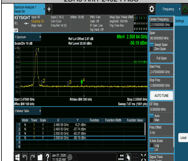
2DH5-Ant1-2480-PASS
