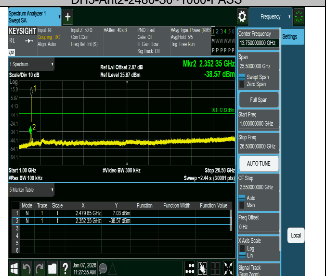
DH5-Ant2-2480-1000~26500-PASS
