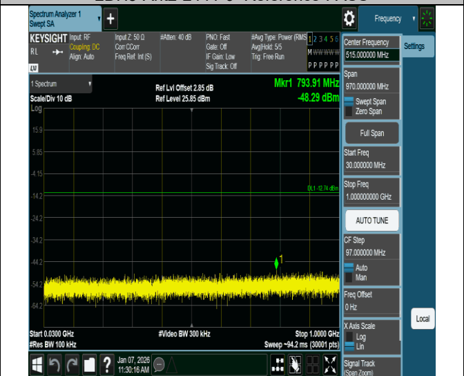
2DH5-Ant2-2441-30~1000-PASS
