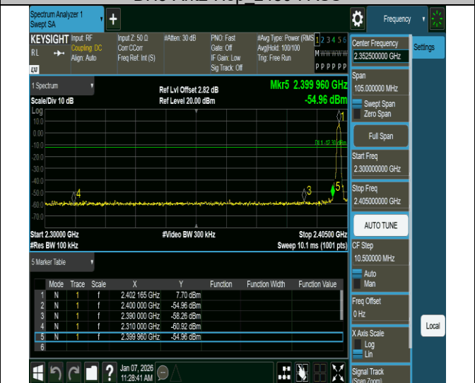
2DH5-Ant2-2402-PASS
