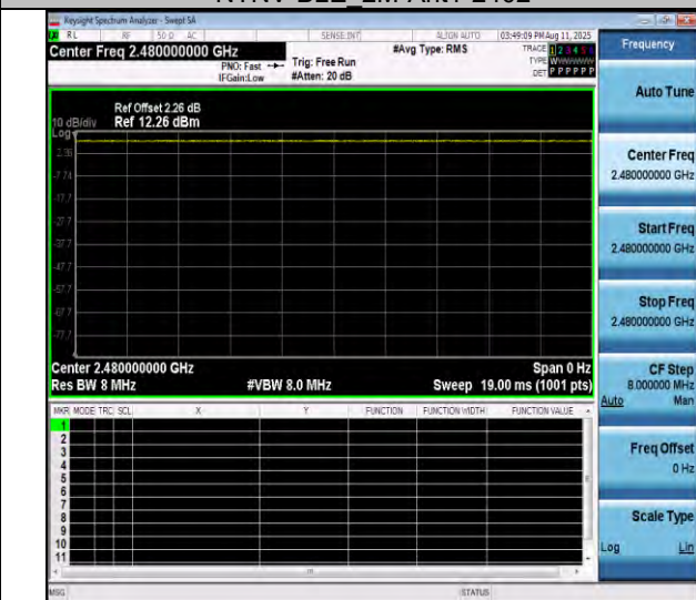
NTVN-BLE_2M-Ant1-2480
