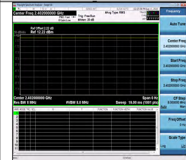
NTVN-BLE_2M-Ant1-2402
