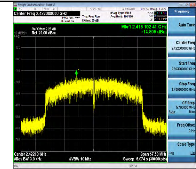
11ax40SISO-Ant1-2422-PASS
