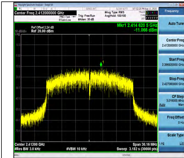
11ax20SISO-Ant1-2412-PASS
