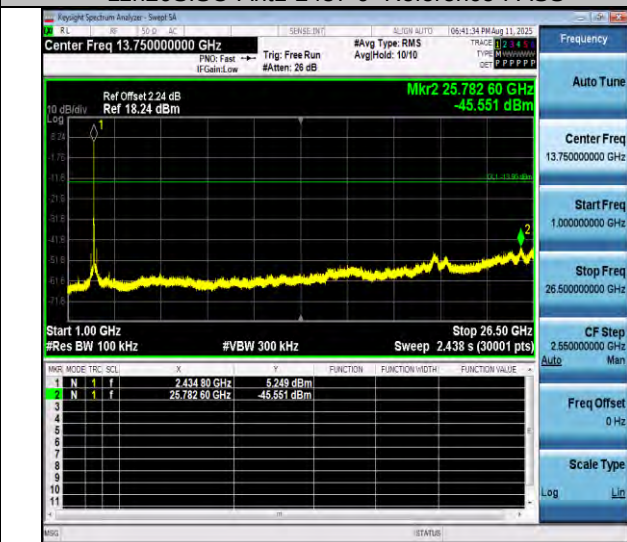
11n20SISO-Ant1-2437-1000-26500-PASS
