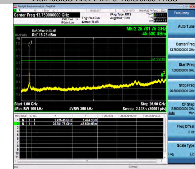
11ax40SISO-Ant1-2422-1000~26500-PASS
