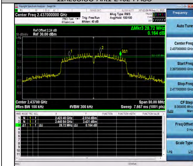
11n40SISO-Ant1-2437-PASS
