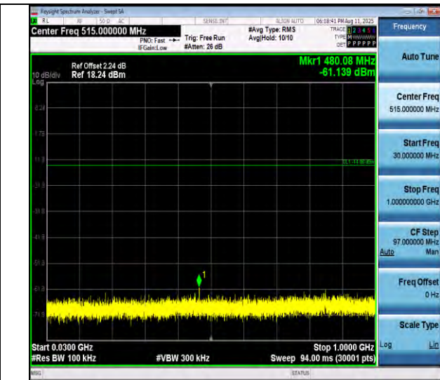
11g-Ant1-2437-30-1000-PASS
