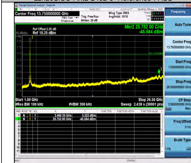
11n20SISO-Ant1-2462-1000~26500-PASS
