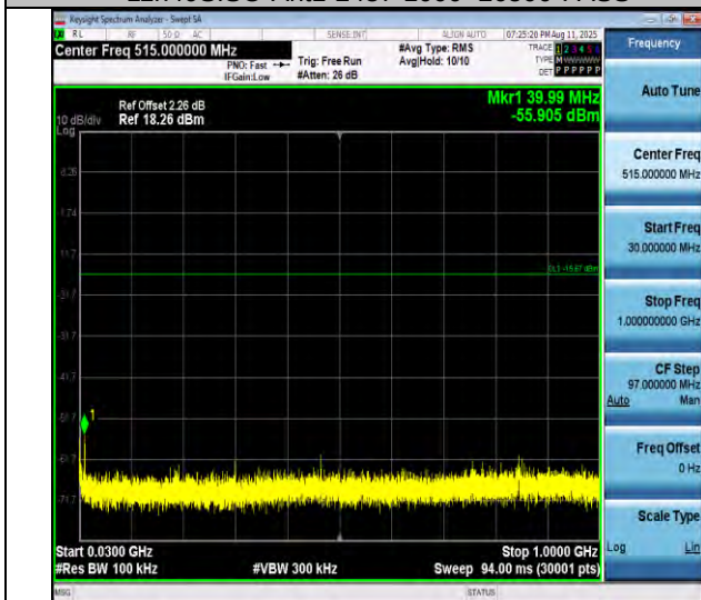
11n40SISO-Ant1-2452-30-1000-PASS
