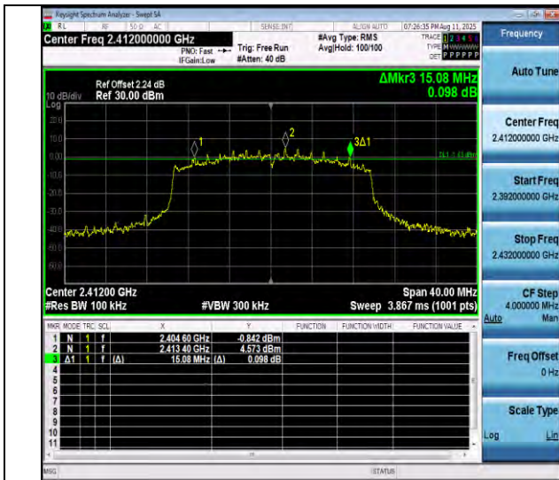
11ax20ISO-Ant1-2412-PASS
