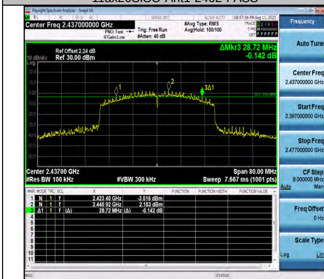
11ax40ISO-Ant1-2437-PASS
