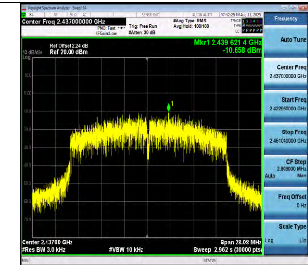
11ax20SISO-Ant1-2437-PASS
