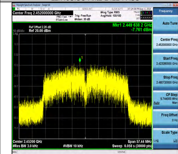
11n40SISO-Ant1-2452-PASS
