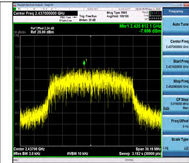
11n20SISO-Ant1-2437-PASS
