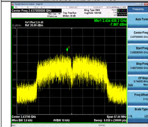
11n40SISO-Ant1-2437-PASS
