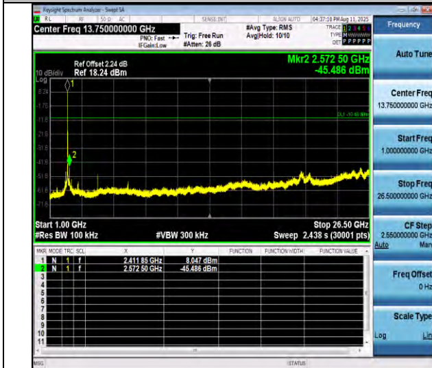
11b-Ant1-2412-1000~26500-PASS
