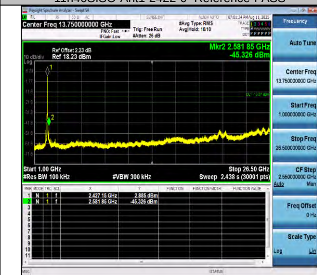
11n40SISO-Ant1-2422-1000~26500-PASS
