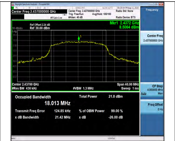
11n20SISO-Ant1-2437
