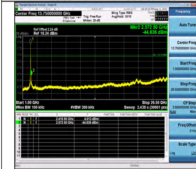
11n20SISO-Ant1-2412-1000-26500-PASS
