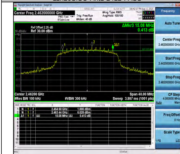
11n20SISO-Ant1-2462-PASS
