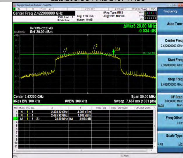
11ax40ISO-Ant1-2422-PASS
