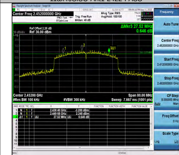
11ax40ISO-Ant1-2452-PASS
