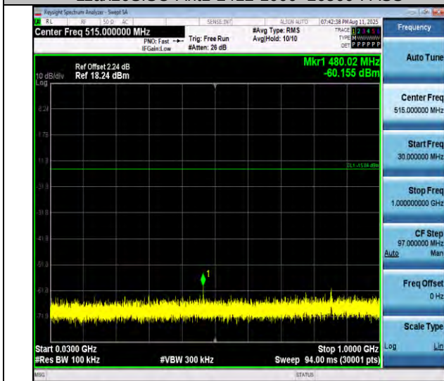
11ax20SISO-Ant1-2437-30~1000-PASS
