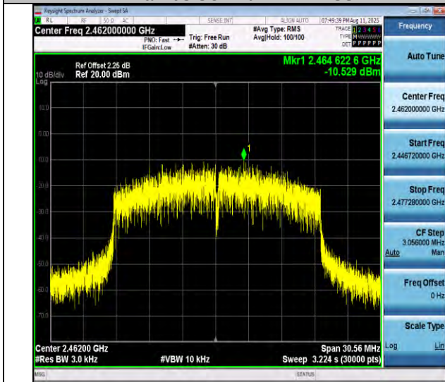
11ax20SISO-Ant1-2462-PASS
