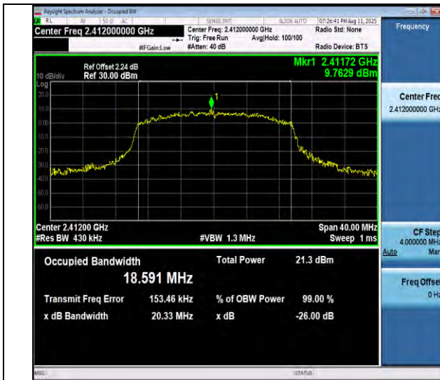
11ax20SISO-Ant1-2412
