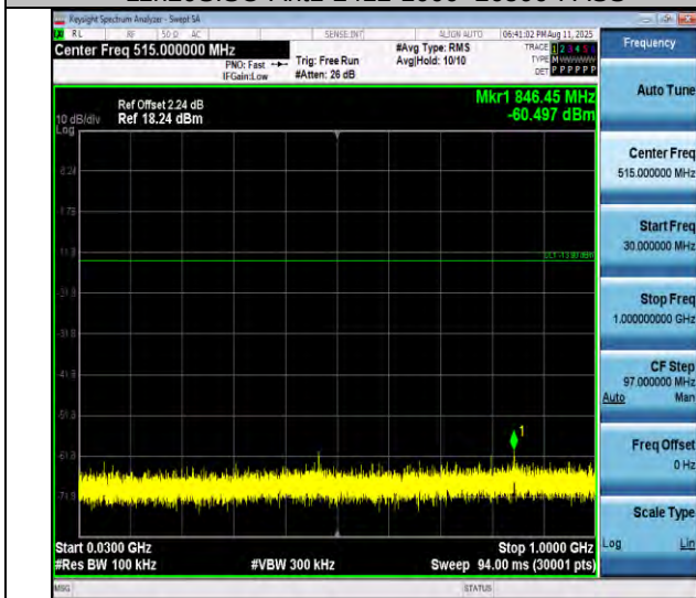
11n20SISO-Ant1-2437-30-1000-PASS
