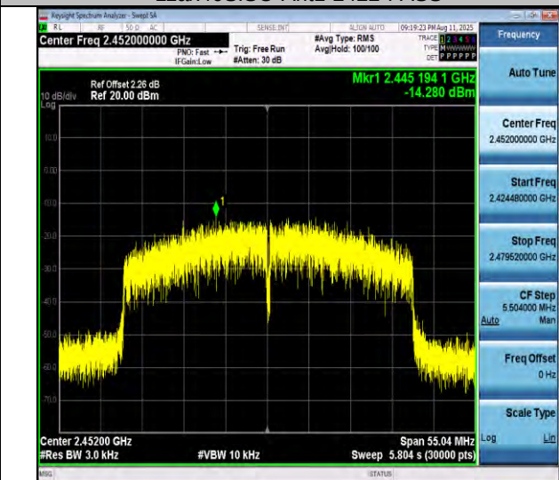
11ax40SISO-Ant1-2452-PASS
