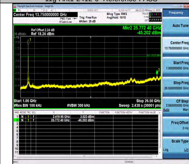
11g-Ant1-2412-1000-26500-PASS
