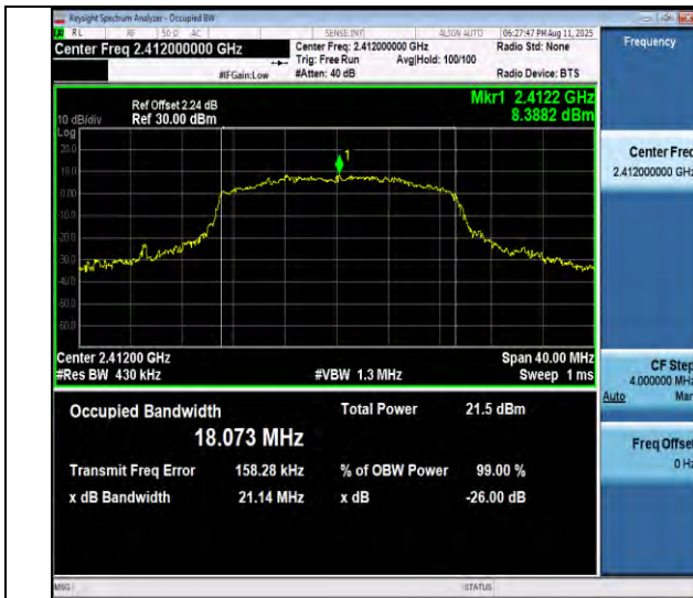
11n20SISO-Ant1-2412
