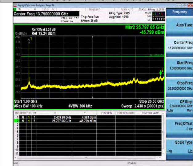
11ax20SISO-Ant1-2437-1000~26500-PASS
