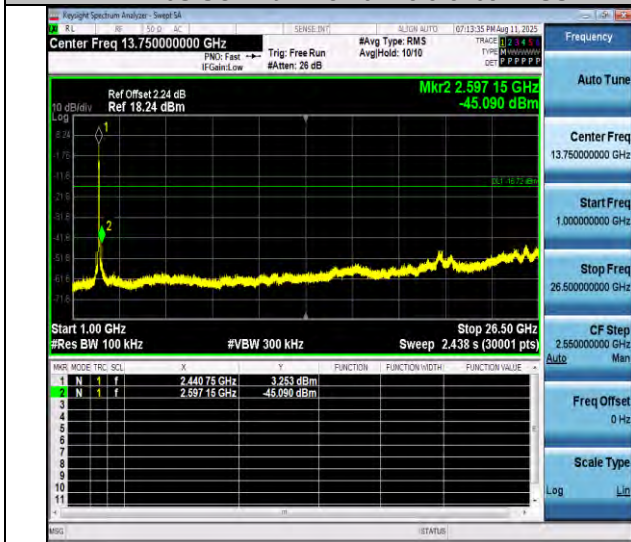
11n40SISO-Ant1-2437-1000-26500-PASS
