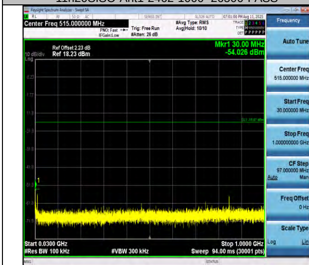
11n40SISO-Ant1-2422-30~1000-PASS
