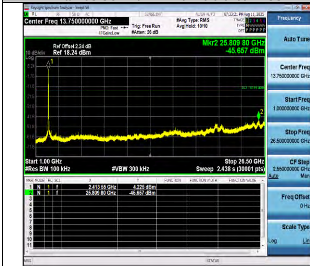
11ax20SISO-Ant1-2412-1000~26500-PASS
