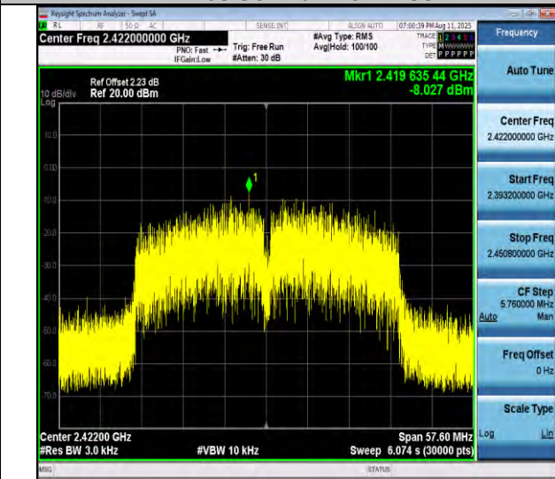
11n40SISO-Ant1-2422-PASS
