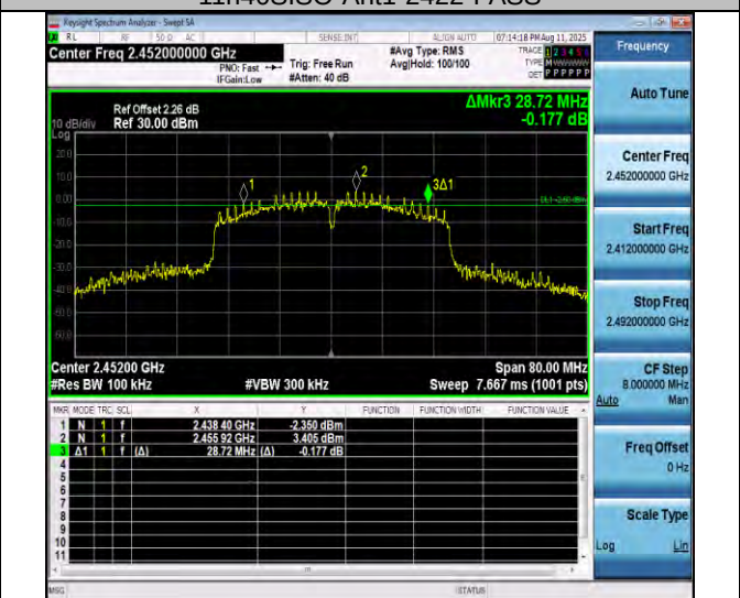
11n40SISO-Ant1-2452-PASS
