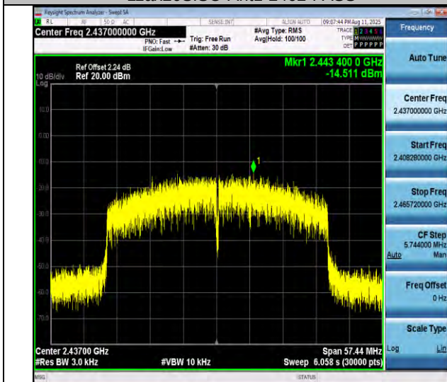
11ax40SISO-Ant1-2437-PASS
