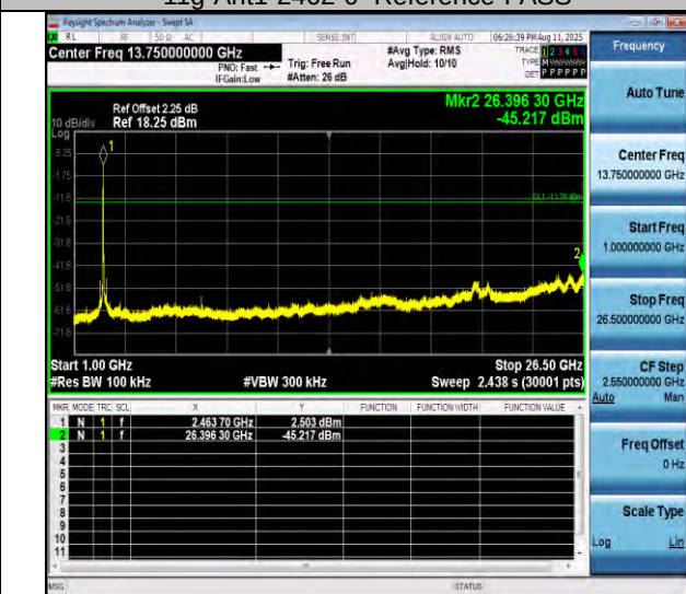
11g-Ant1-2462-1000-26500-PASS
