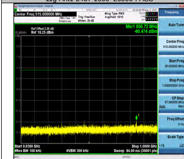
11g-Ant1-2462-30-1000-PASS
