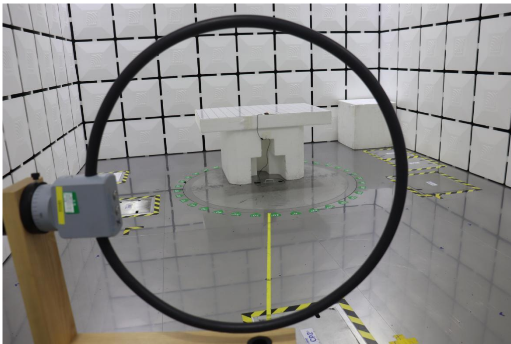
Below 30MHz
