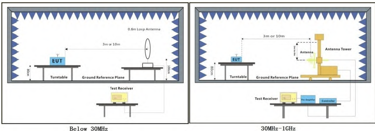
Below 30MHz
