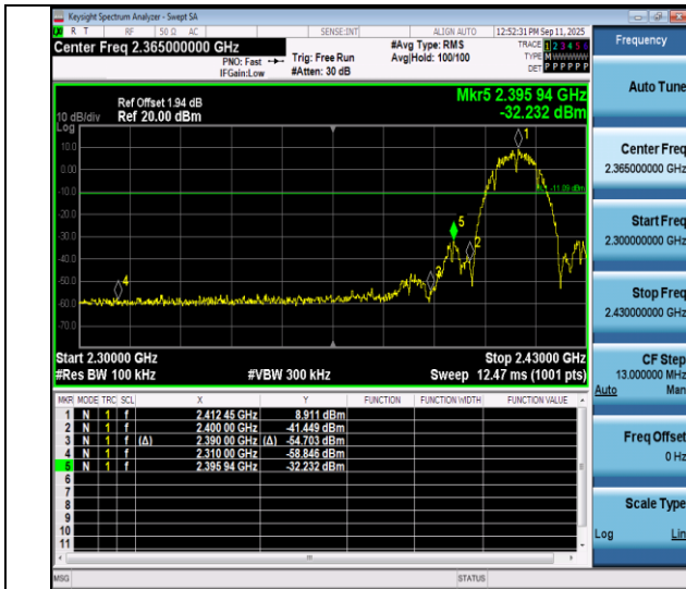
11b-Ant1-2412-PASS
