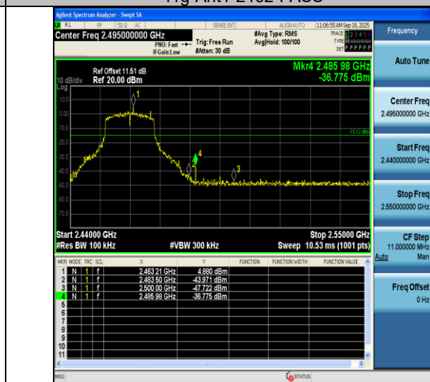
11n20SISO-Ant1-2462-PASS
