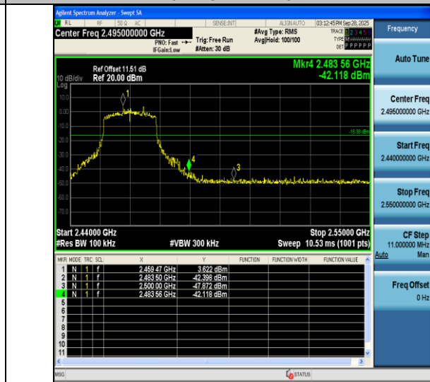
11ax20SISO-Ant1-2462-PASS
