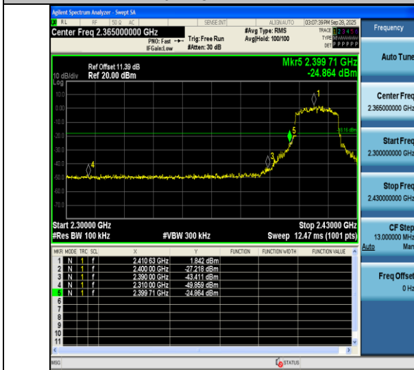
11ax20SISO-Ant1-2412-PASS
