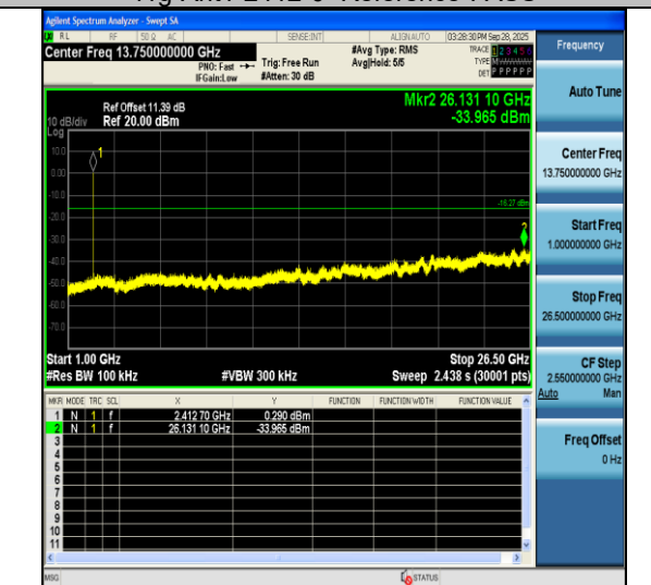
11g-Ant1-2412-1000~26500-PASS
