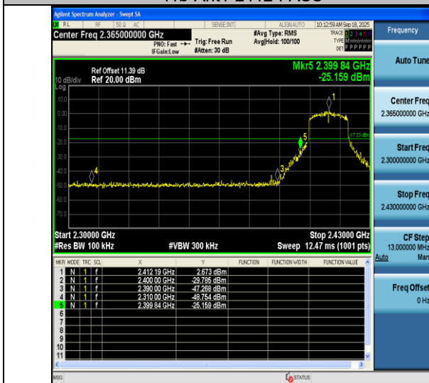
11g-Ant1-2412-PASS
