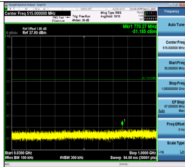
11b-Ant1-2462-30~1000-PASS
