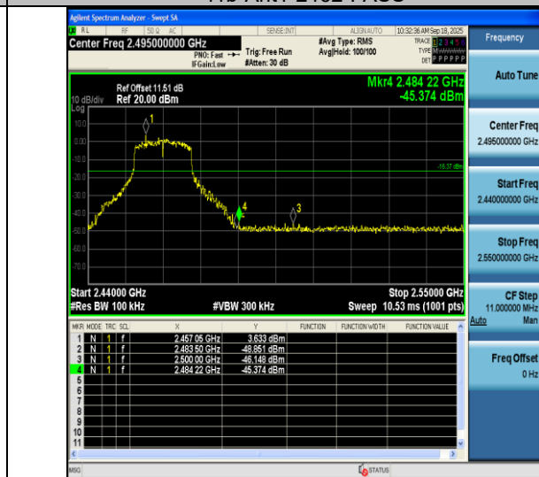
11g-Ant1-2462-PASS
