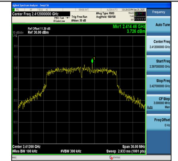
11g-Ant1-2412-0~Reference-PASS
