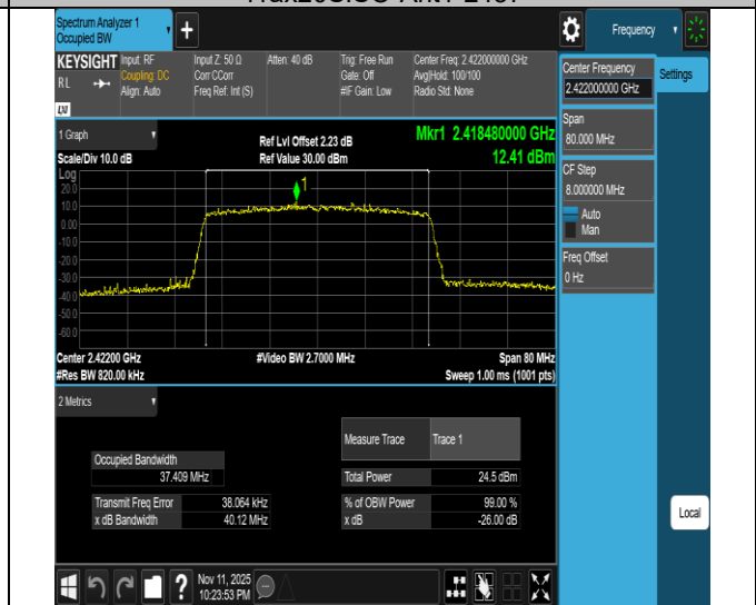
11ax40SISO-Ant1-2422
