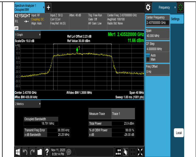
11ax20SISO-Ant1-2437
