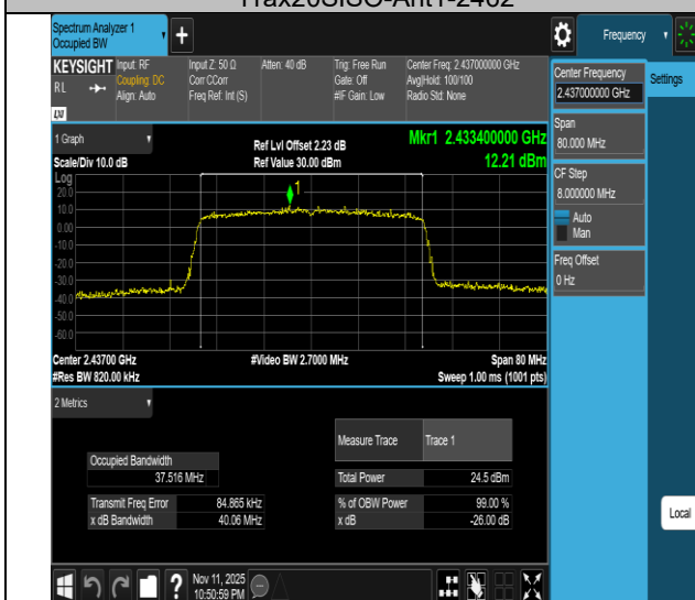
11ax40SISO-Ant1-2437
