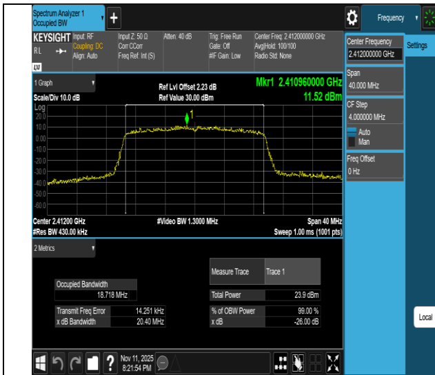
11ax20SISO-Ant1-2412
