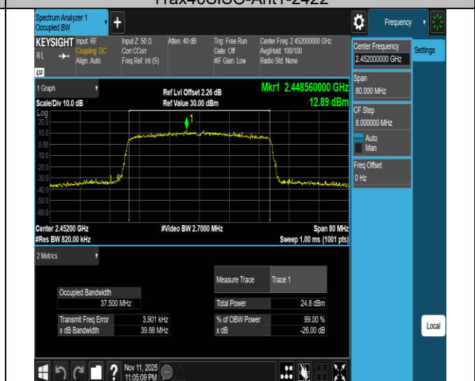
11ax40SISO-Ant1-2452
