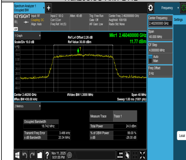
11ax20SISO-Ant1-2462
