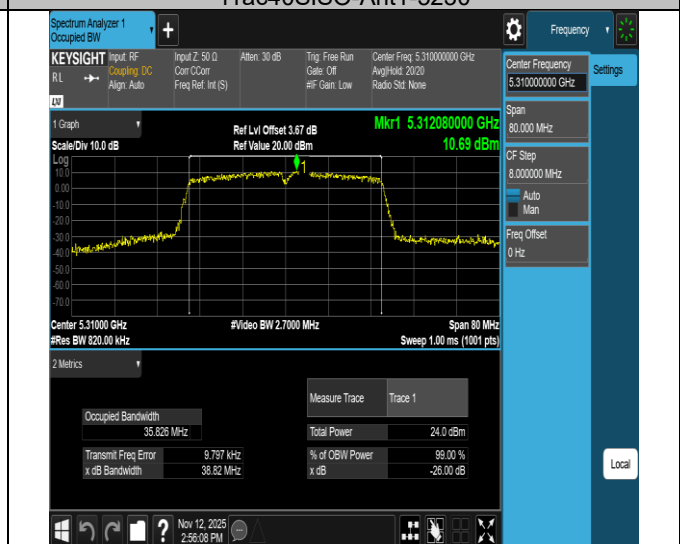
11ac40SISO-Ant1-5310
