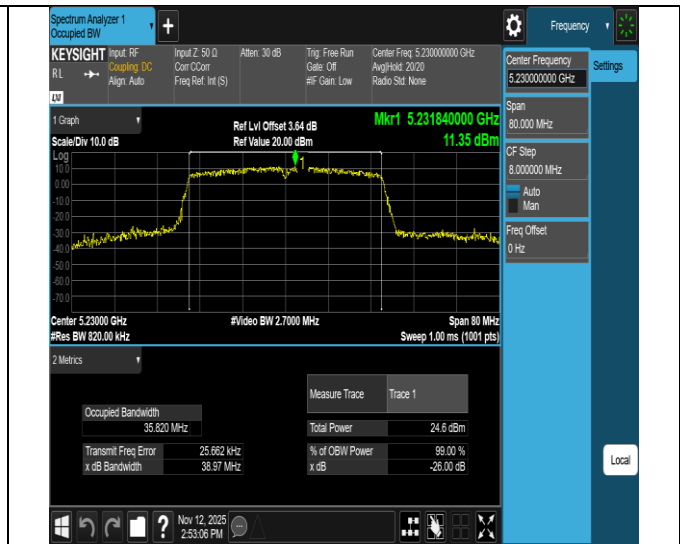
11ac40SISO-Ant1-5230
