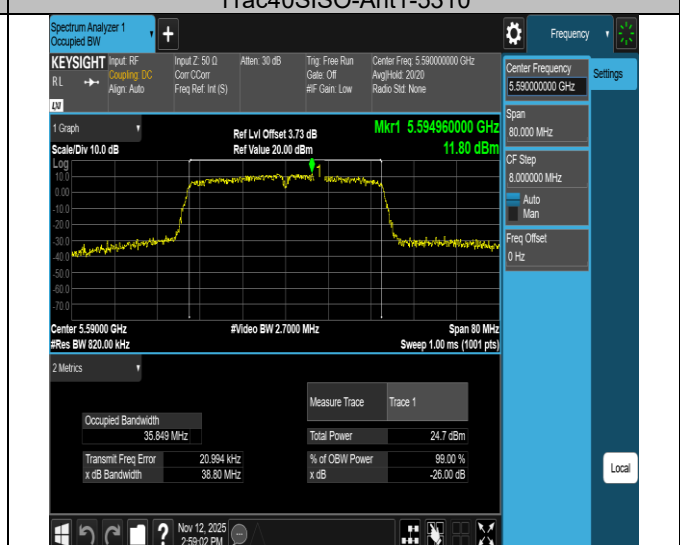
11ac40SISO-Ant1-5590
