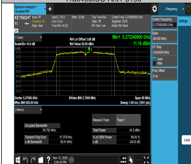
11ac40SISO-Ant1-5270
