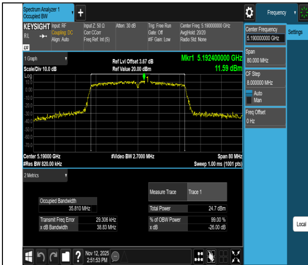
11ac40SISO-Ant1-5190
