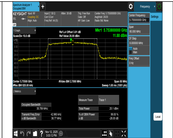
11ac40SISO-Ant1-5755
