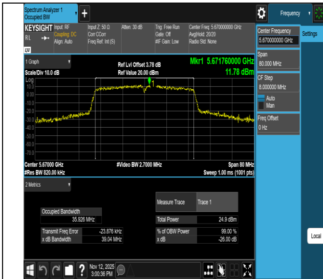
11ac40SISO-Ant1-5670
