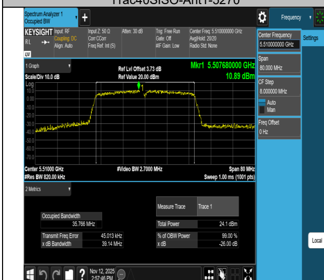
11ac40SISO-Ant1-5510
