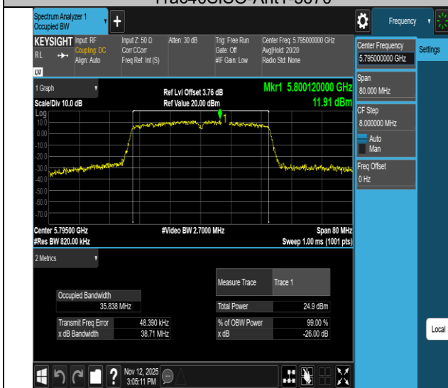
11ac40SISO-Ant1-5795
