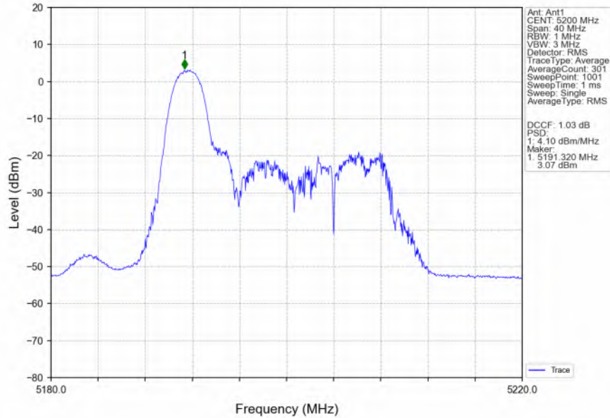
802.11ax(HEW20)_MCH_5200MHz_RU52_Left_Ant1_NTNV
