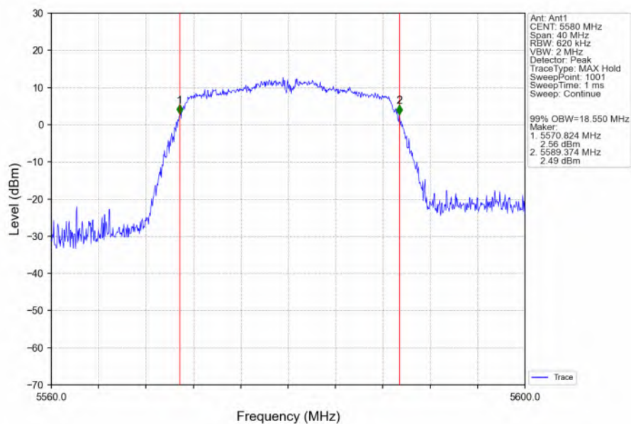
802.11ac(VHT20)_MCH_5580MHz_Ant1_NTNV
