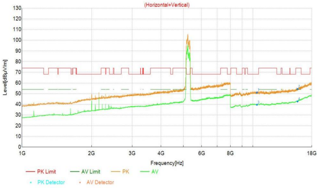
11AC_80M_5530
