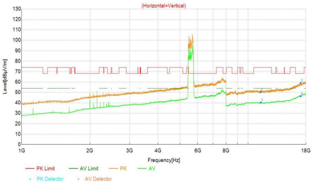
11AX_20M_5240
