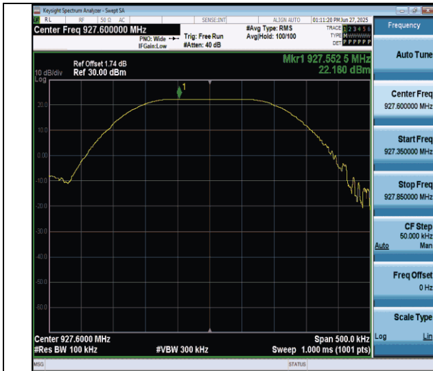
LORA_DSS-Ant1-927.6-0~Reference-PASS
