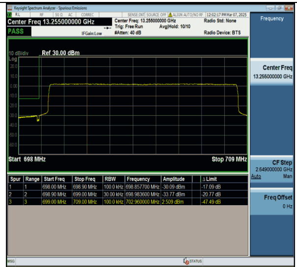
Band12-10MHz-QPSK-23060-50RB#0-PASS
