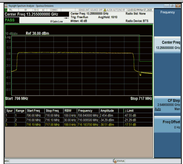
Band12-10MHz-QPSK-23130-50RB#0-PASS
