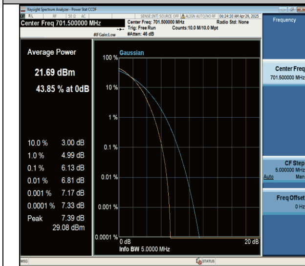
Band12-5MHz-64QAM-23035-25RB#0-PASS
