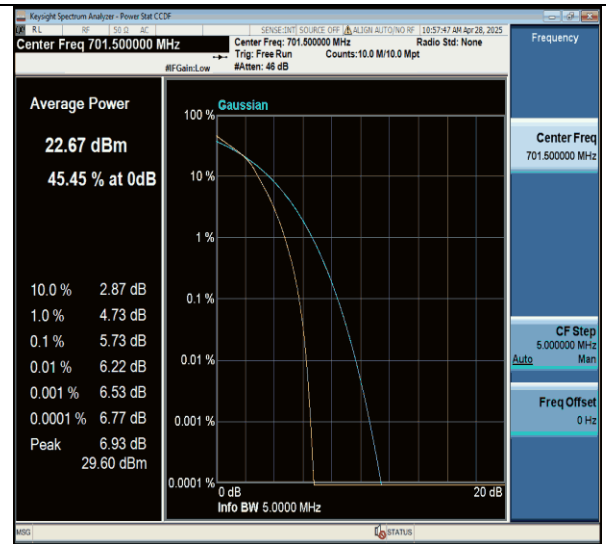
Band12-5MHz-16QAM-23035-25RB#0-PASS
