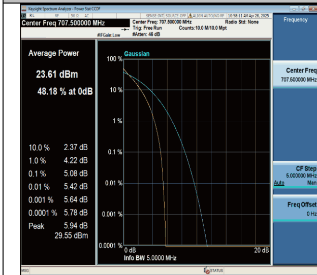
Band12-5MHz-QPSK-23095-25RB#0-PASS
