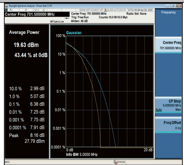
Band12-5MHz-256QAM-23035-25RB#0-PASS
