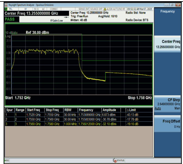
Band4-3MHz-QPSK-20385-15RB#0-PASS
