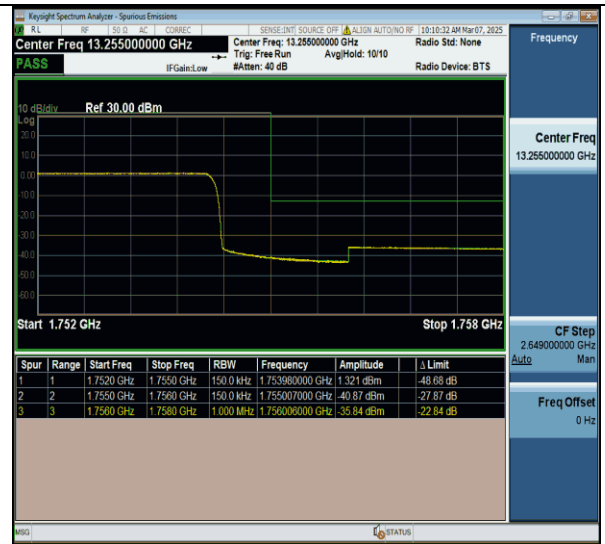
Band4-15MHz-QPSK-20325-75RB#0-PASS
