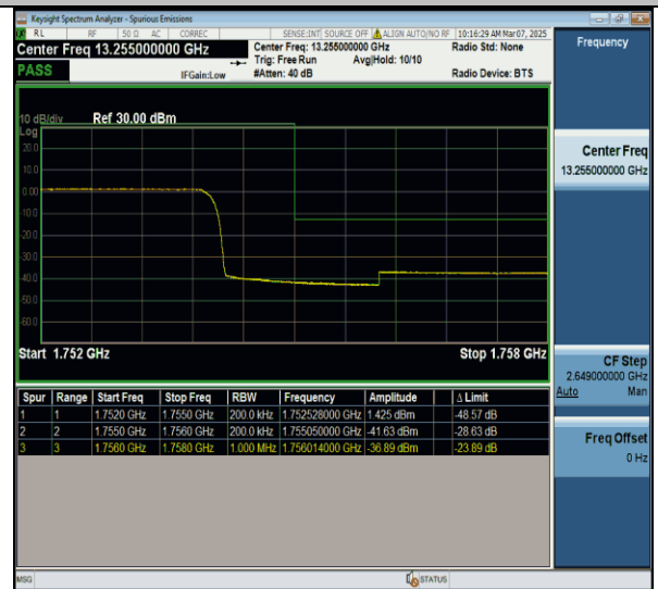
Band4-20MHz-QPSK-20300-100RB#0-PASS
