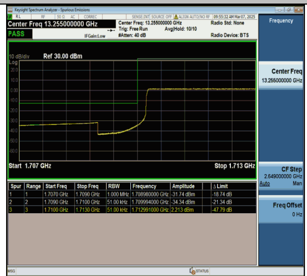
Band4-5MHz-QPSK-19975-25RB#0-PASS
