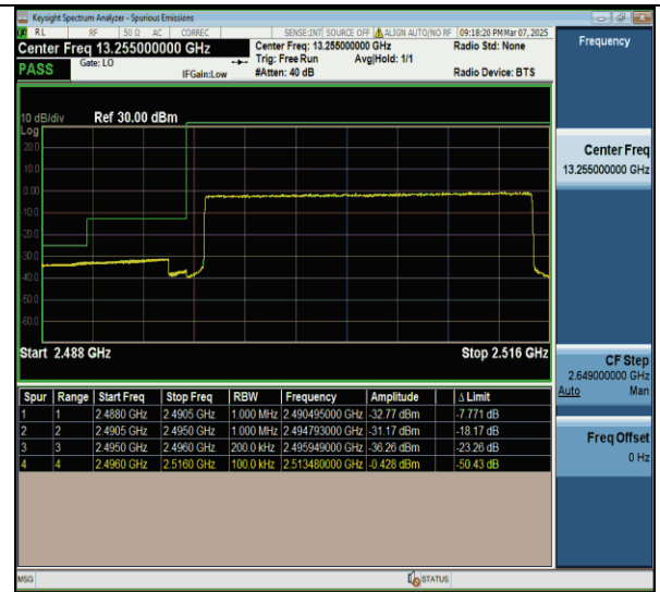
Band41-20MHz-QSPK-39750-100RB#0-PASS
