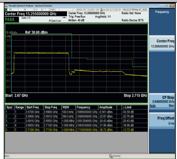
Band41-20MHz-QSPK-41490-100RB#0-PASS
