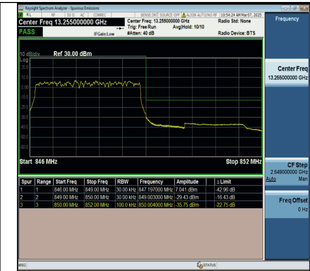
Band5-3MHz-QPSK-20635-15RB#0-PASS
