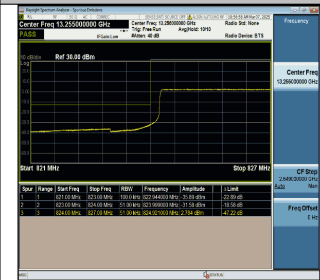
Band5-5MHz-QPSK-20425-25RB#0-PASS
