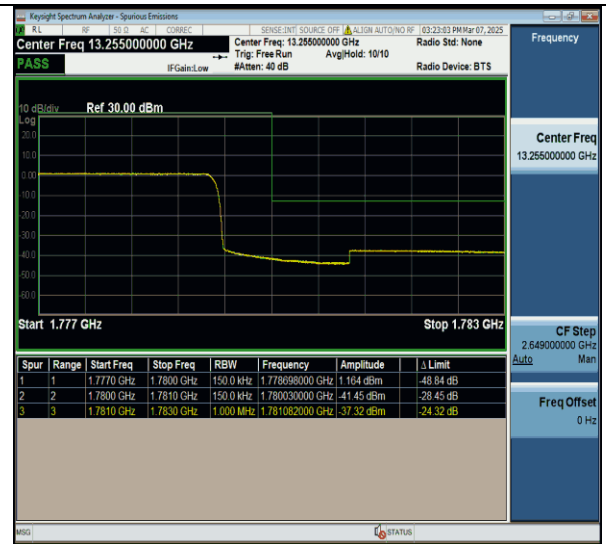
Band66-15MHz-QSPK-132597-75RB#0-PASS
