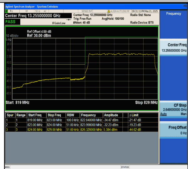
Band5-5MHz-QPSK-20425-25RB#0-PASS
