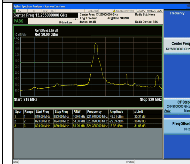
Band5-5MHz-QPSK-20425-1RB#0-PASS
