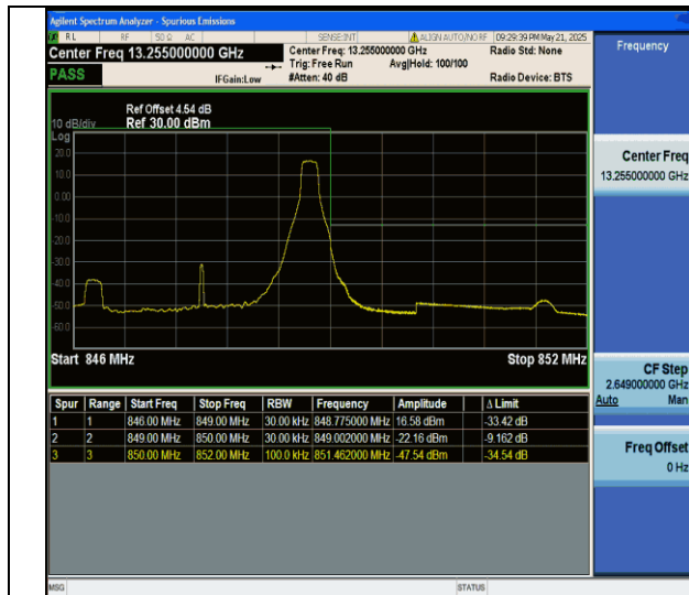
Band5-3MHz-QPSK-20635-1RB#14-PASS
