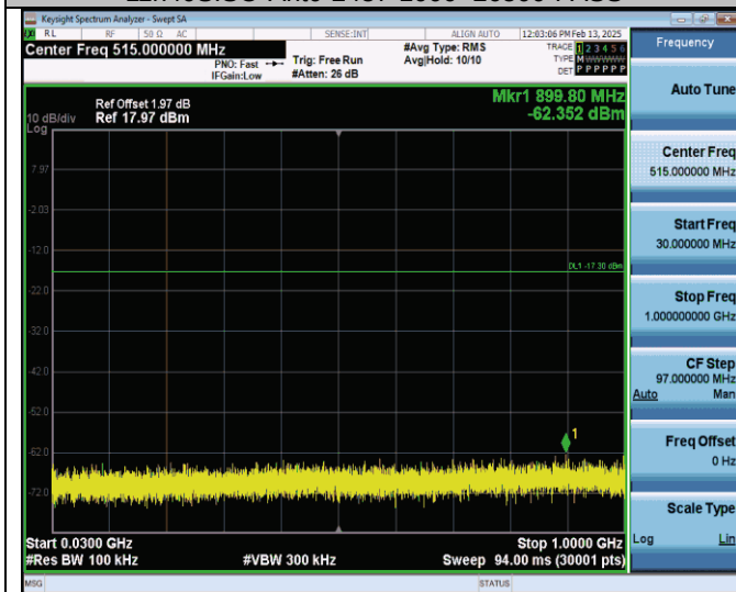
11n40SISO-Ant0-2452-30-1000-PASS
