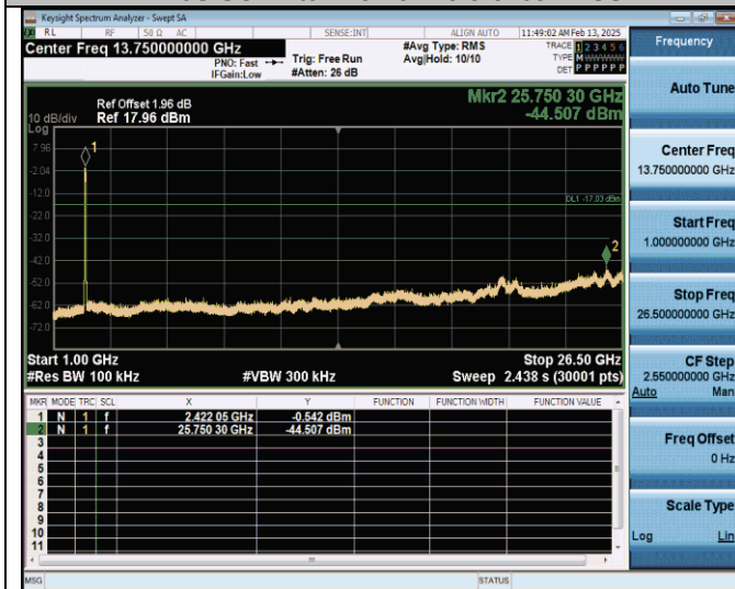
11n40SISO-Ant0-2437-1000-26500-PASS
