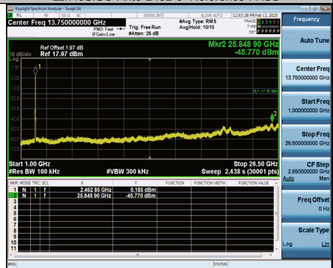
11n40SISO-Ant0-2452-1000-26500-PASS
