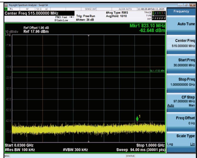
11n40SISO-Ant0-2437-30-1000-PASS
