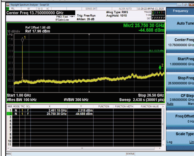
11n20SISO-Ant0-2462-1000-26500-PASS
