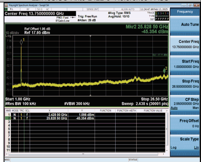
11n40SISO-Ant0-2422-1000-26500-PASS
