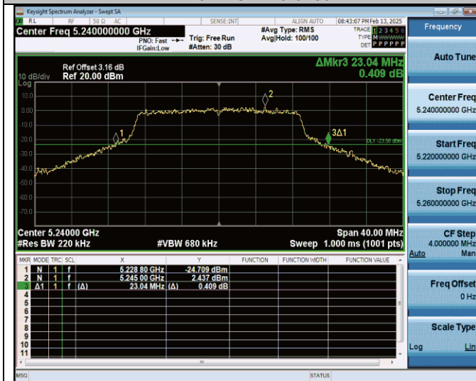
11ac20SISO-Ant0-5240
