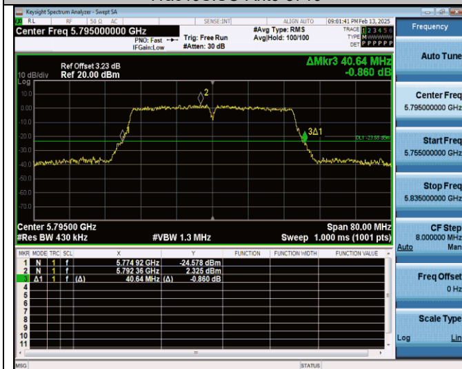
11ac40SISO-Ant0-5795
