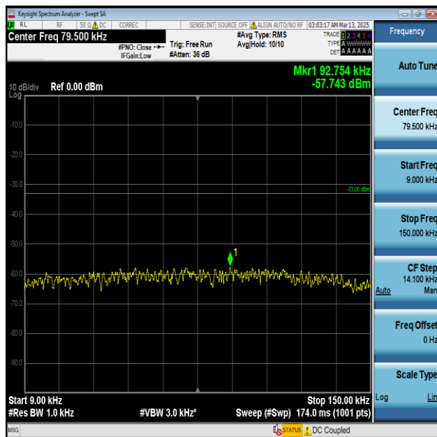
Band5-10MHz-QPSK-20600-1RB#0-0.009~0.15-PASS
