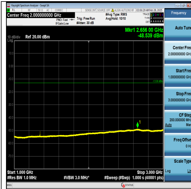
Band71-20MHz-QPSK-133322-1RB#0-1000~3000-PASS
