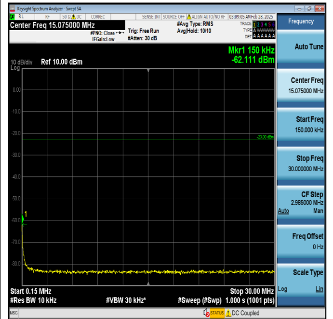
Band71-20MHz-QPSK-133372-1RB#0-0.15~30-PASS
