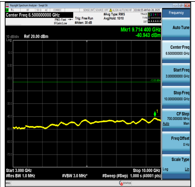
Band71-20MHz-QPSK-133322-1RB#0-3000~10000-PASS
