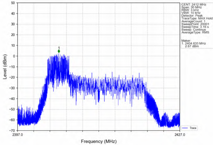
802.11ax(HEW20)_LCH_2412MHz_RU106_Ant1 (SISO) NTNv
