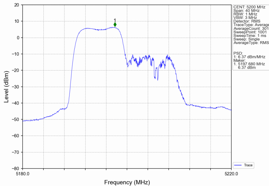
802.11ax(HEW20)_MCH_5200MHz_RU106_Ant1_NTNV
