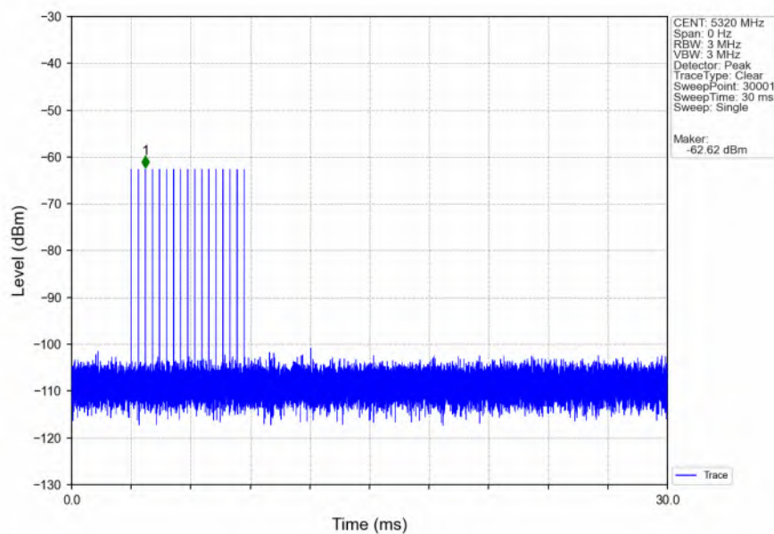
Signal Calibration_802.11ax(HEW20)_2A_5320MHz_RadarType3_Trial0
