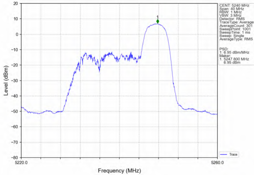
802.11ax(HEW20) HCH 5240MHz RU106 Ant1 NTV
