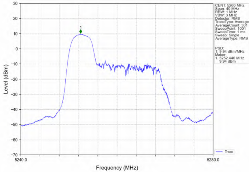
802.11ax(HEW20)_LCH_5260MHz_RU106_Ant1_NTNV
