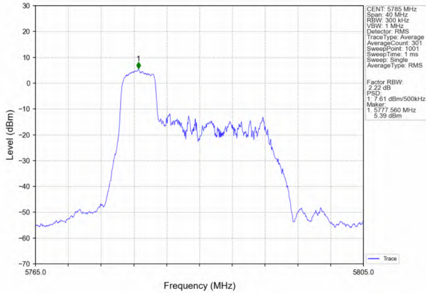
802.11ax(HEW20)_MCH_5785MHz_RU106_Ant1_NTNV
