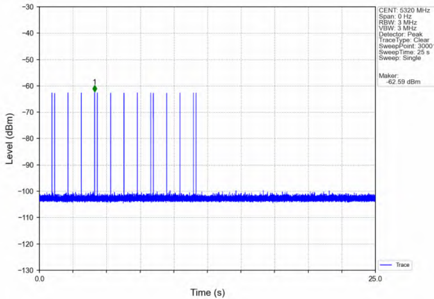
Signal Calibration_802.11ax(HEW20)_2A_5320MHz_RadarType5_Trial0
