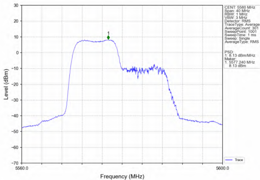
802.11ax(HEW20)_MCH_5580MHz_RU106_Ant1_NTNV
