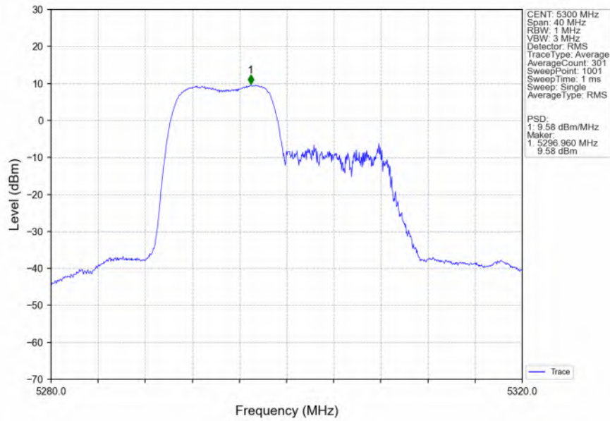
802.11ax(HEW20)_MCH_5300MHz_RU106_Ant1_NTNV
