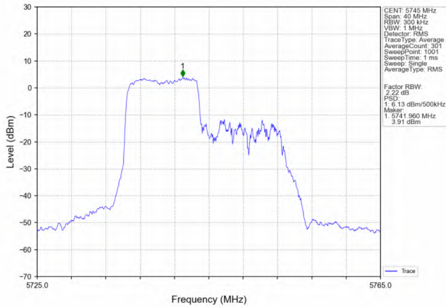
802.11ax(HEW20)_LCH_5745MHz_RU106_Ant1_NTNV
