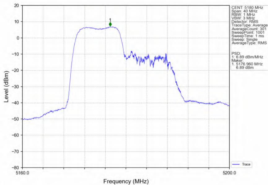
802.11ax(HEW20)_LCH_5180MHz_RU106_Ant1_NTNV
