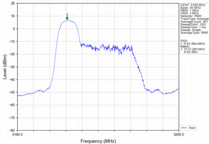
802.11ax(HEW20)_LCH_5180MHz_RU106_Ant1_NTNV
