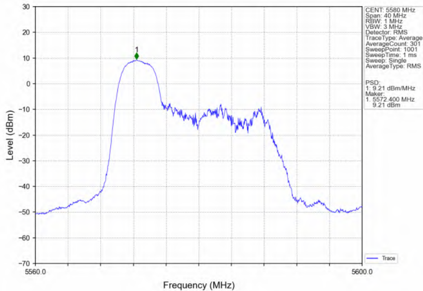
802.11ax(HEW20)_MCH_5580MHz_RU106_Ant1_NTNV
