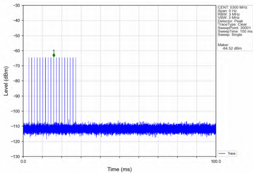
Signal Calibration_802.11ax(HEW20)_2A_5300MHz_RadarType1_Trial0
