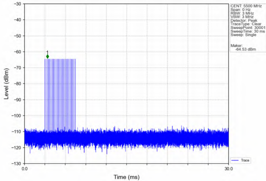
Signal Calibration_802.11ax(HEW20)_2C_5500MHz_RadarType3_Trial0
