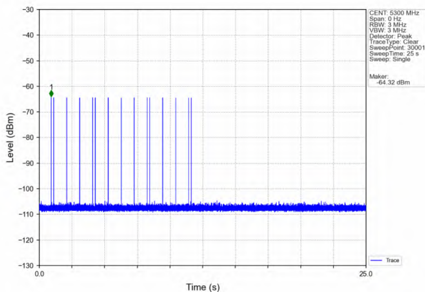
Signal Calibration_802.11ax(HEW20)_2A_5300MHz_RadarType5_Trial0
