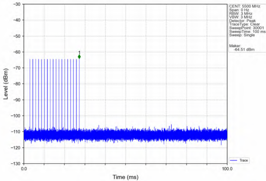
Signal Calibration_802.11ax(HEW20)_2C_5500MHz_RadarType1_Trial0
