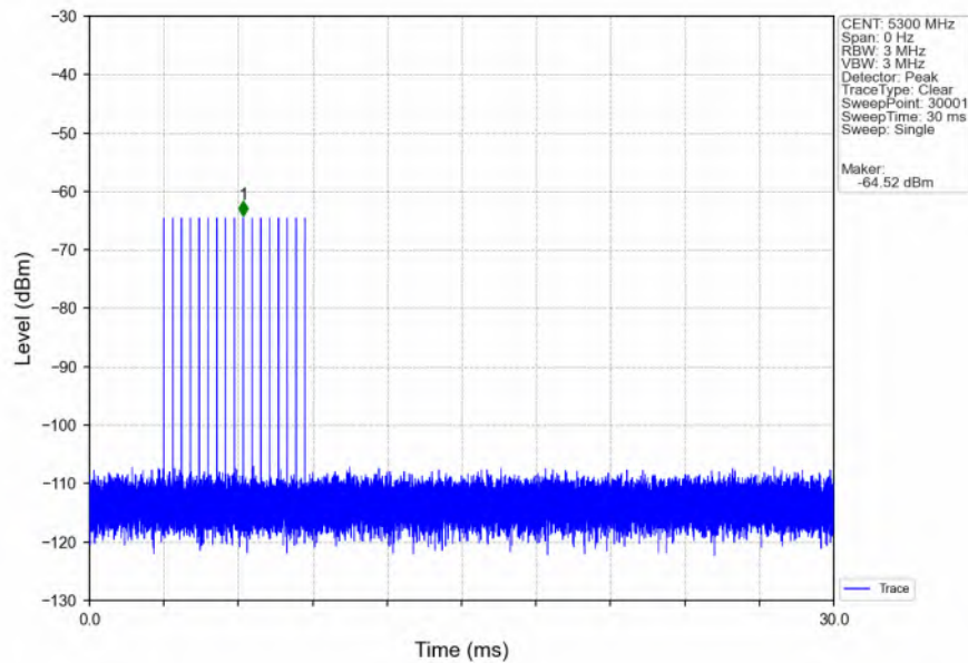
Signal Calibration_802.11ax(HEW20)_2A_5300MHz_RadarType3_Trial0
