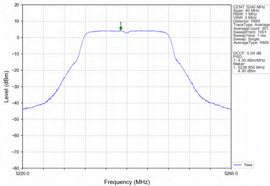
802.11a_HCH_5240MHz_Ant1_NTNV
