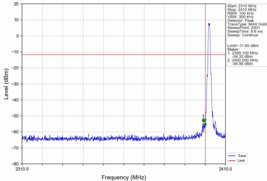
1M_LCH_2402MHz_Ant1_NTNV
