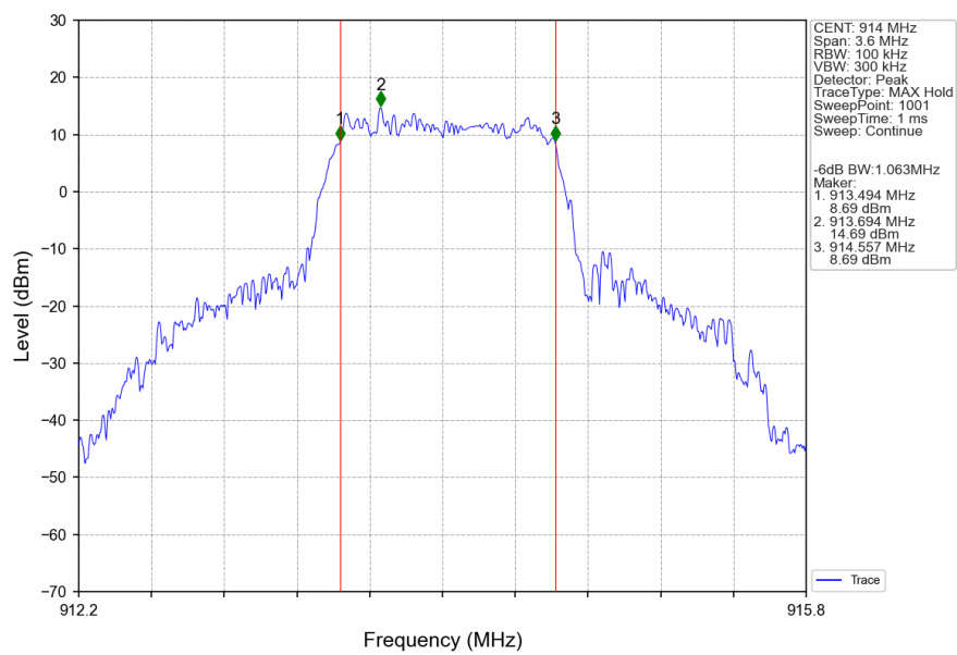
1200kHz_MCH_914MHz_Ant1_NTNV
