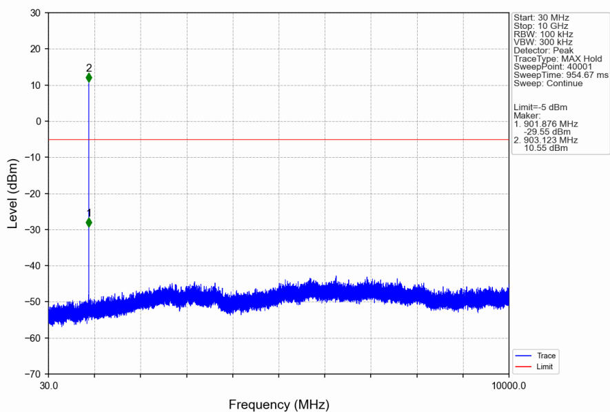
1200kHz_LCH_903.2MHz_Ant1_NTNV
