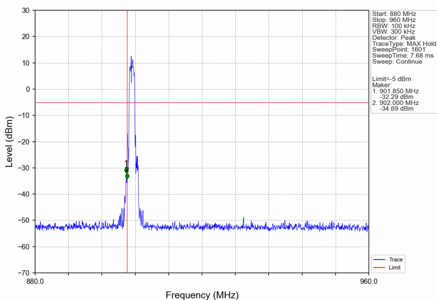
1200kHz_LCH_903.2MHz_Ant1_NTNV
