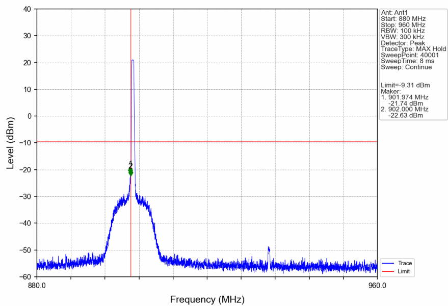
CSS_500KHz_LCH_902.5MHz_Ant1_NTNV
