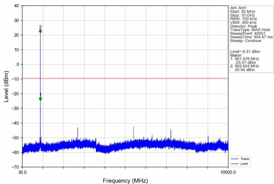
CSS_500KHz_LCH_902.5MHz_Ant1_NTNV
