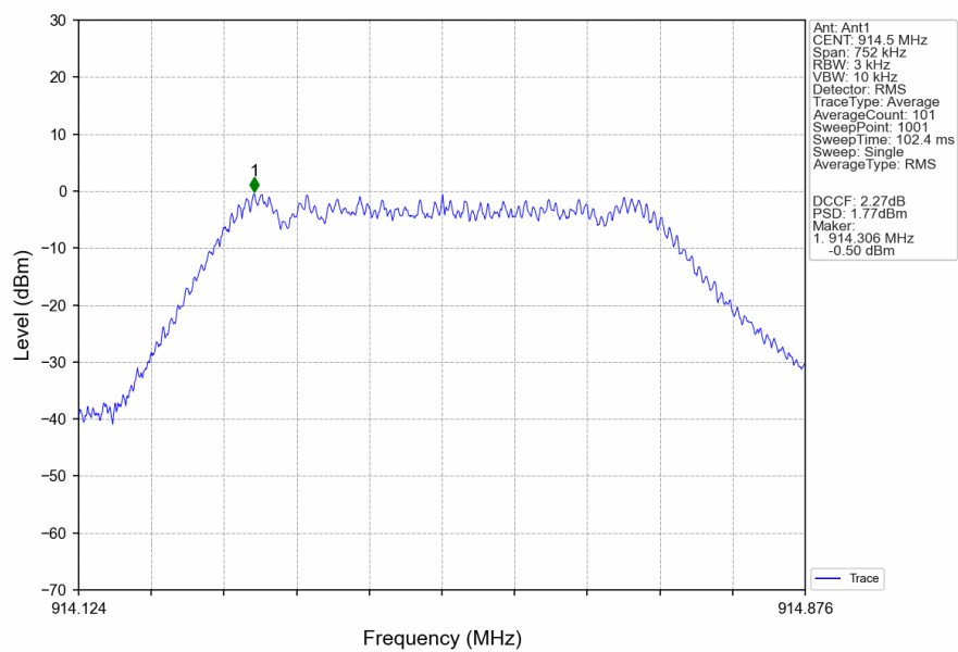
CSS_500KHz_MCH_914.5MHz_Ant1_NTNV
