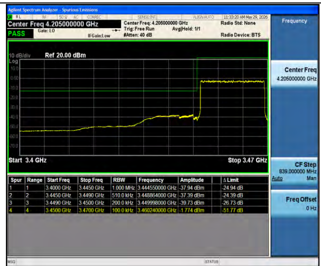
Band42(3450-3550)-20MHz-QPSK-42190-100RB#0-PASS
