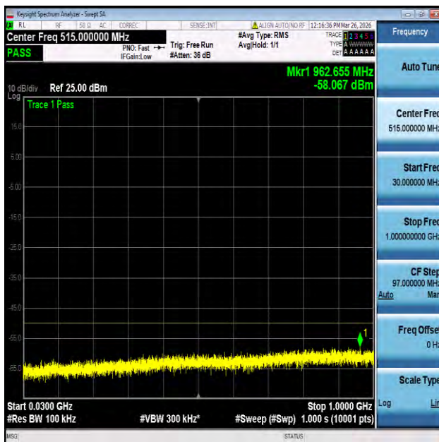
NTNV-n30-PC3-15-10-M-DFT-BPSK-Edge_1RB_Left-30-1000- PASS
