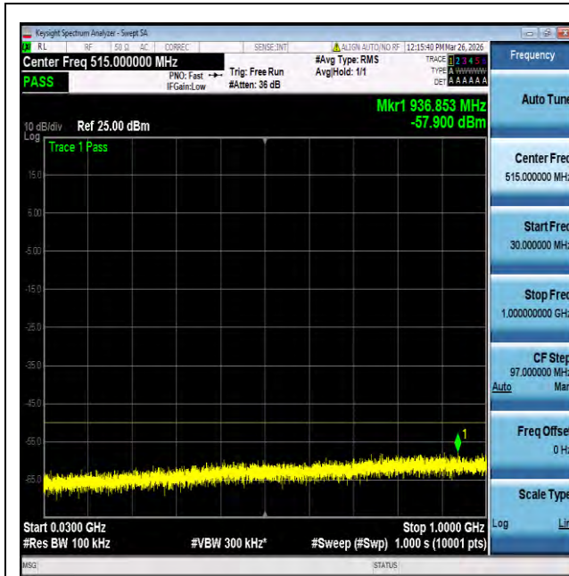
NTNV-n30-PC3-15-10-L-CP-QPSK-Edge_1RB_Left-30-1000- PASS
