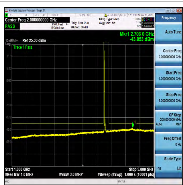
NTNV-n30-PC3-15-10-M-CP-QPSK-Edge_1RB_Left-1000-3000- PASS
