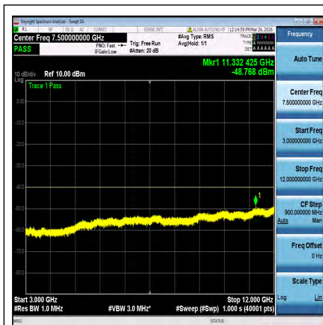
NTNV-n30-PC3-15-10-L-DFT-BPSK-Edge_1RB_Left-3000-12000- PASS
