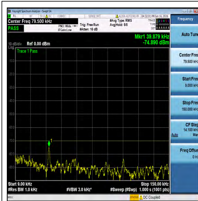
NTNV-n30-PC3-15-10-M-DFT-BPSK-Edge_1RB_Left-0.009-0.15- PASS
