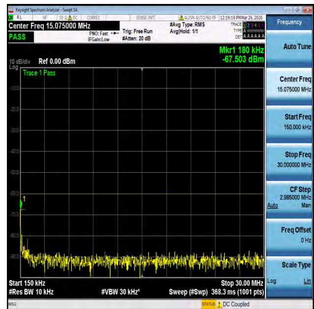
NTNV-n30-PC3-15-10-H-CP-QPSK-Edge_1RB_Left-0.15-30-PASS
