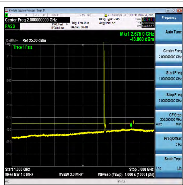
NTNV-n30-PC3-15-10-L-CP-QPSK-Edge_1RB_Left-1000-3000- PASS
