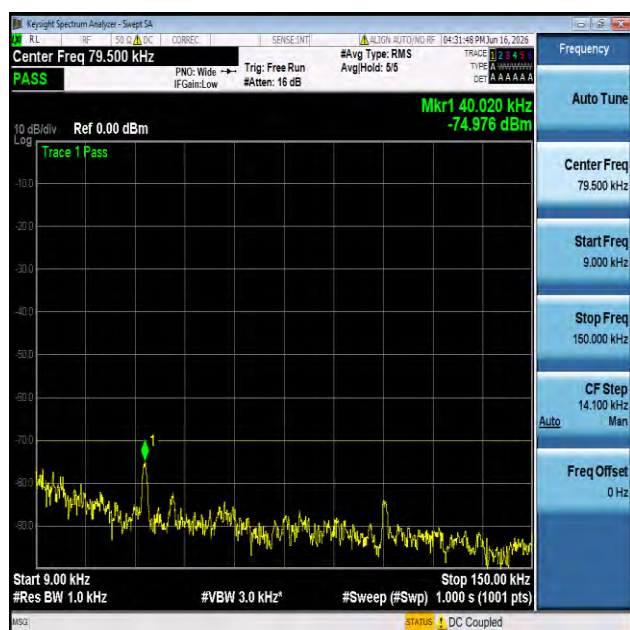
NTNV-n30-PC3-15-10-L-CP-QPSK-Edge_1RB_Left-0.009-0.15- PASS
