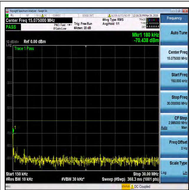
NTNV-n30-PC3-15-10-M-DFT-BPSK-Edge_1RB_Left-0.15-30- PASS
