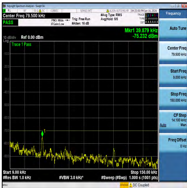
NTNV-n30-PC3-15-10-H-CP-QPSK-Edge_1RB_Left-0.009-0.15-PASS
