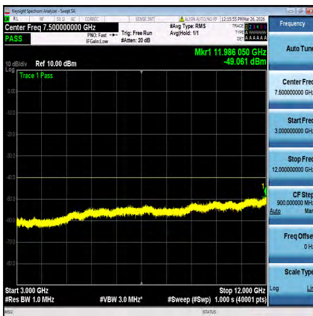
NTNV-n30-PC3-15-10-L-CP-QPSK-Edge_1RB_Left-3000-12000- PASS
