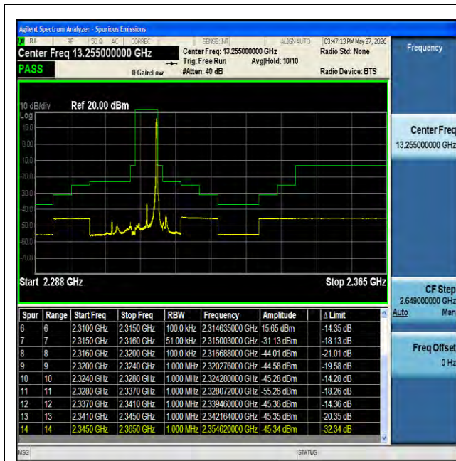
NTNV-n30-PC3-15-5-H-CP-QPSK-Edge_1RB_Right-PASS
