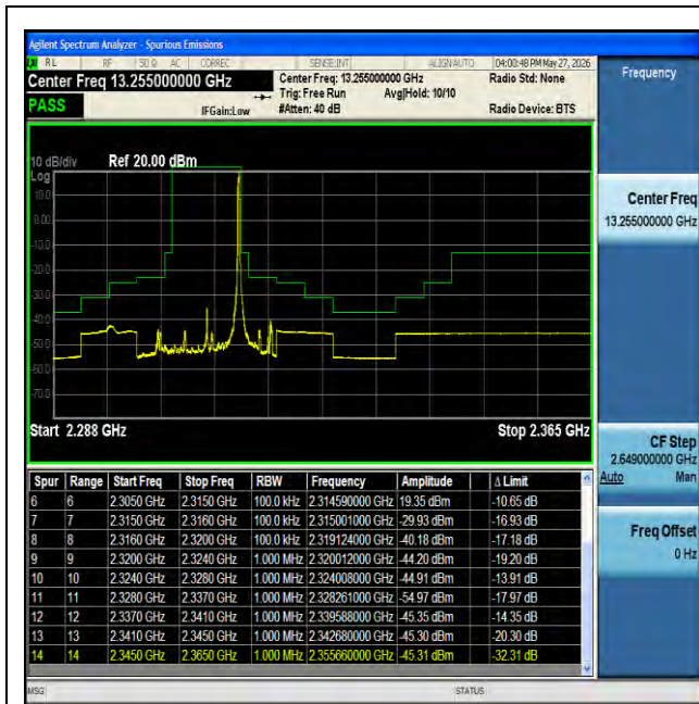
NTNV-n30-PC3-15-10-H-DFT-BPSK-Edge_1RB_Right-PASS
