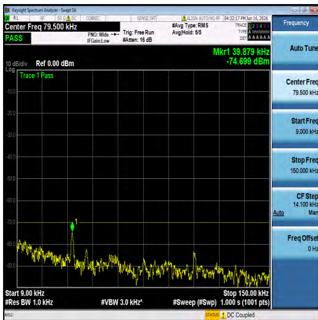
NTNV-n30-PC3-15-10-M-CP-QPSK-Edge_1RB_Left-0.009-0.15-PASS
