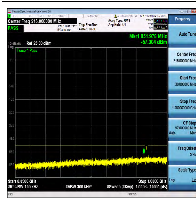
NTNV-n30-PC3-15-10-M-CP-QPSK-Edge_1RB_Left-30-1000- PASS
