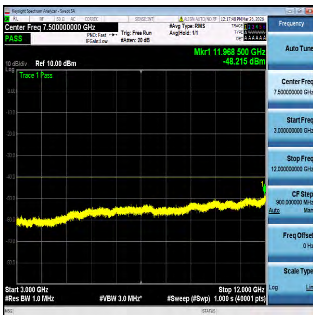
NTNV-n30-PC3-15-10-M-CP-QPSK-Edge_1RB_Left-3000-12000- PASS
