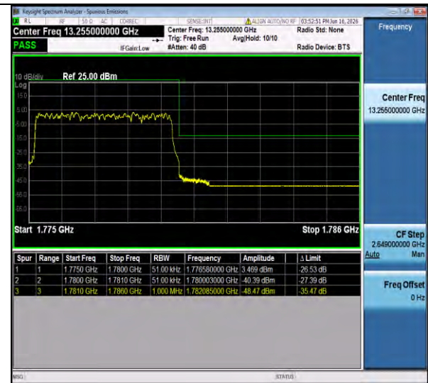
NTNV-n66-PC3-15-5-H-CP-QPSK-Outer_Full-PASS
