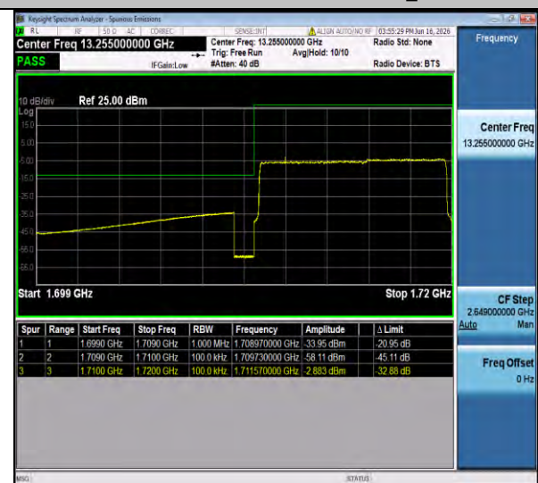
NTNV-n66-PC3-15-10-L-CP-QPSK-Outer_Full-PASS
