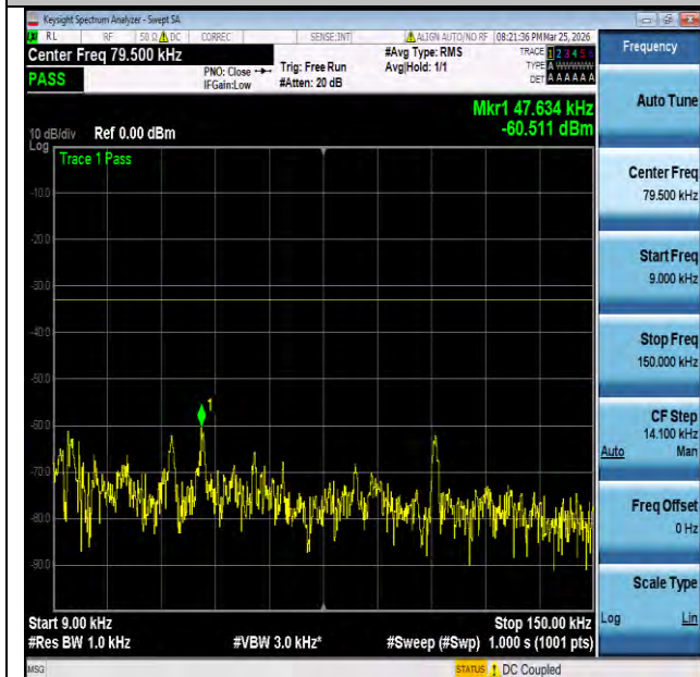
NTNV-n13-PC3-15-10-L-CP-QPSK-Edge_1RB_Left-0.009-0.15-PASS
