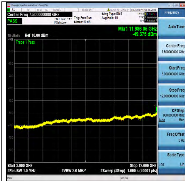
NTNV-n13-PC3-15-10-L-DFT-BPSK-Edge_1RB_Left-3000-12000-PASS
