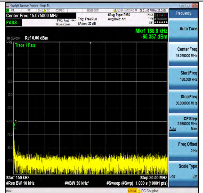
NTNV-n13-PC3-15-10-L-CP-QPSK-Edge_1RB_Left-0.15-30-PASS
