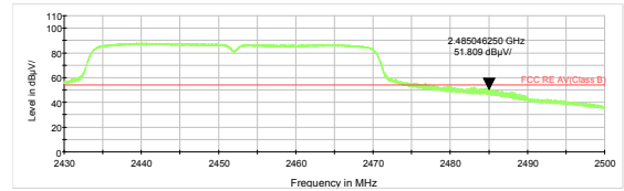
802.11n HT40 -Channel 9 Average
