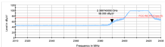
802.11g-Channel 1 Peak
