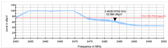
802.11g-Channel 11 Peak
