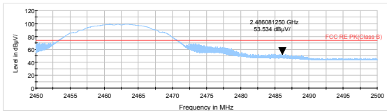
802.11b-Channel 11 Peak
