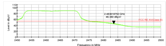
802.11n HT20 -Channel 11 Average
