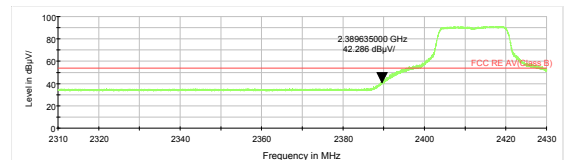
802.11g-Channel 1 Average
