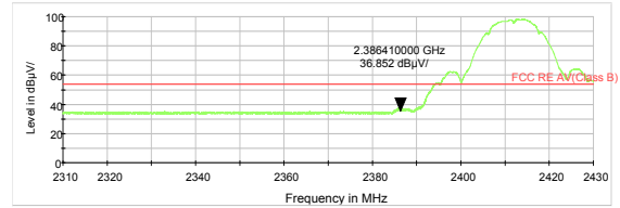
802.11b-Channel 1 Average
