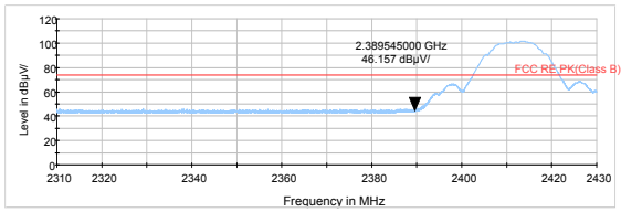
802.11b-Channel 1 Peak
