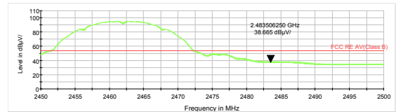
802.11b-Channel 11 Average
