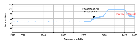
802.11n HT20 -Channel 1 Peak
