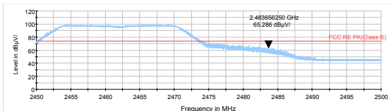
802.11n HT20 -Channel 11 Peak
