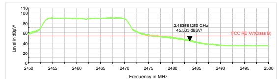
802.11g-Channel 11 Average
