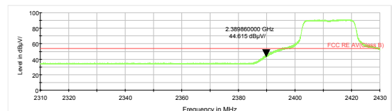
802.11n HT20 -Channel 1 Average
